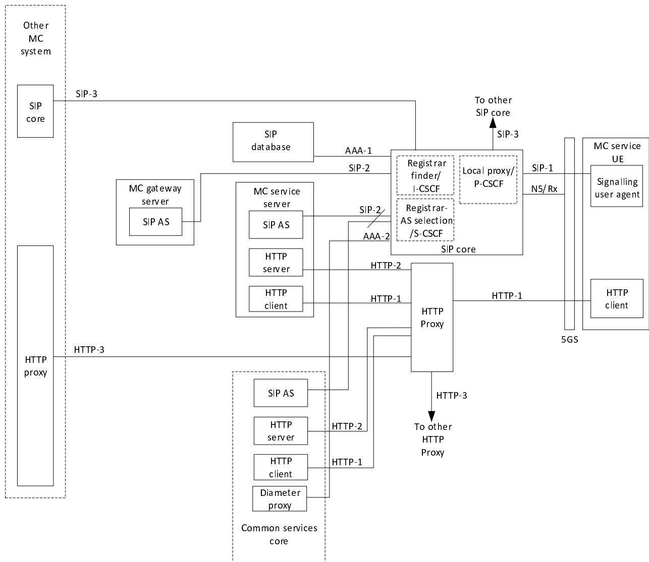
Figure 5.3.1-2: Common functional model for signalling control plane
