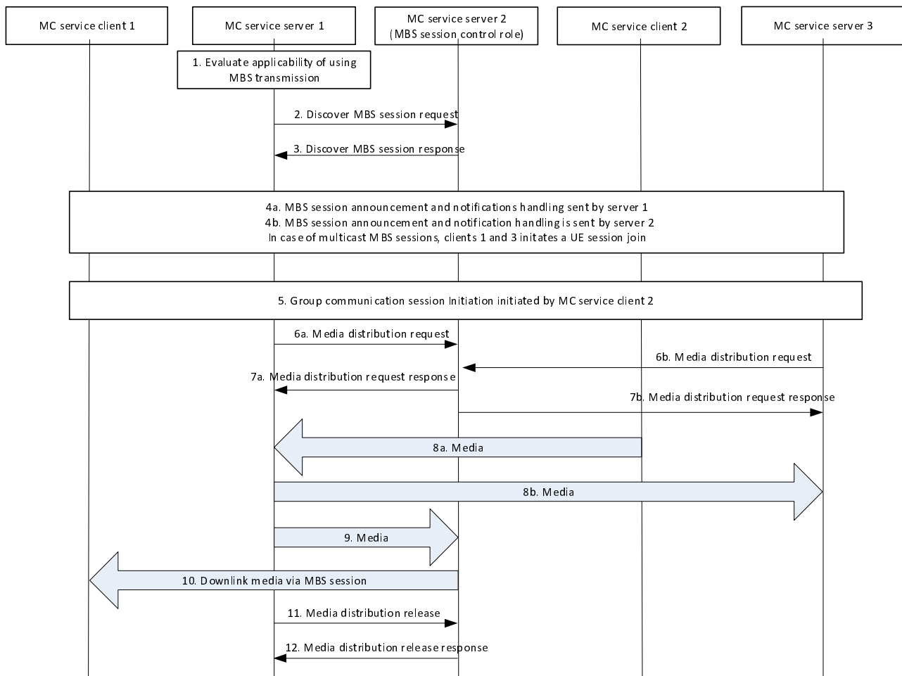
Figure 7.3.3.7.2.2-1: Multiple server MBS procedure within one group call
