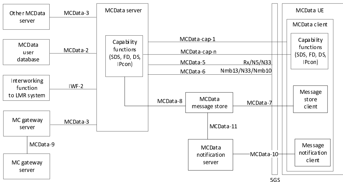
Figure 5.6.1-1: Generic MCDATA functional model for application plane
