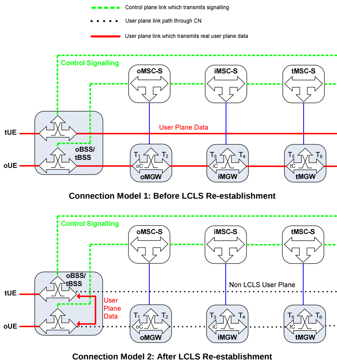
Figure 7.3.4.1.1: LCLS Re-establishment (Network model)
