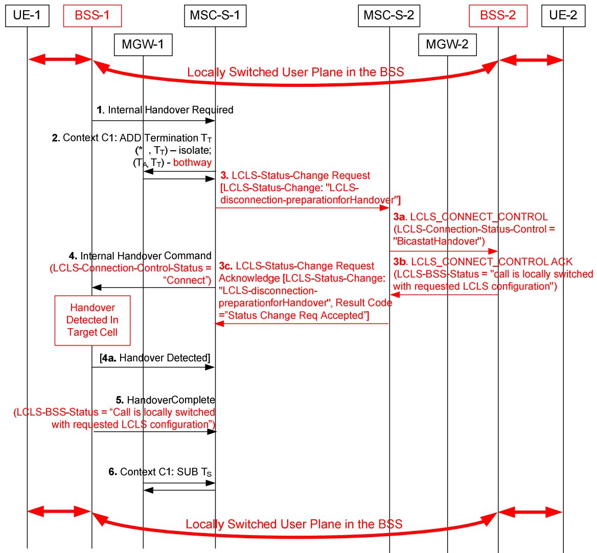
Figure 8.4.5.7.2.1: BSS Internal Handover for AoIP that Does Not Modify LCLS Status of a Locally Switched Call
