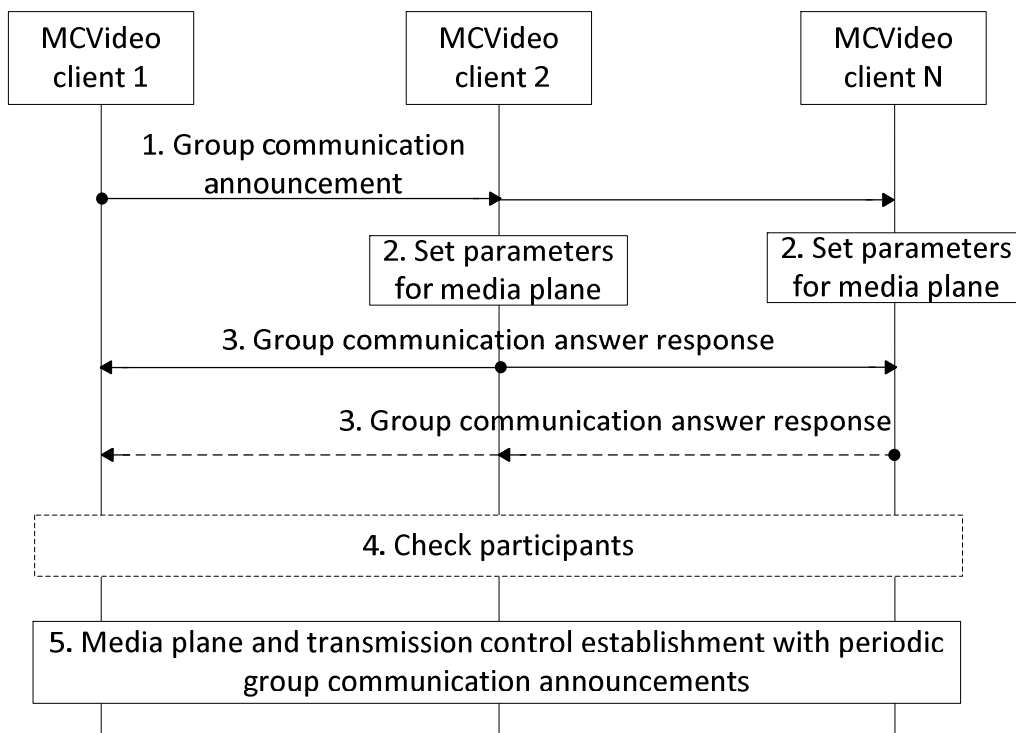
Figure 7.1.3.3.2-1: MCVideo group communication setup
