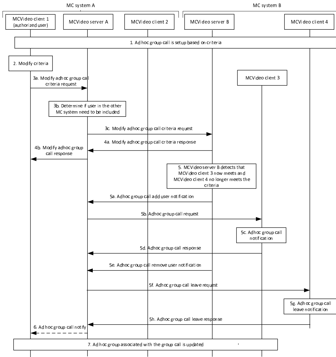
Figure 7.19.3.2.7-1: Modifying the criteria for determining the participants during an ongoing ad hoc group call between multiple MC systems
