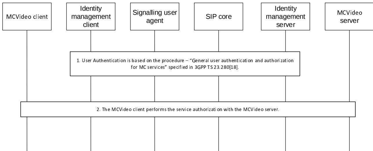
Figure 7.12-1: MCVideo user authentication and registration, single domain
