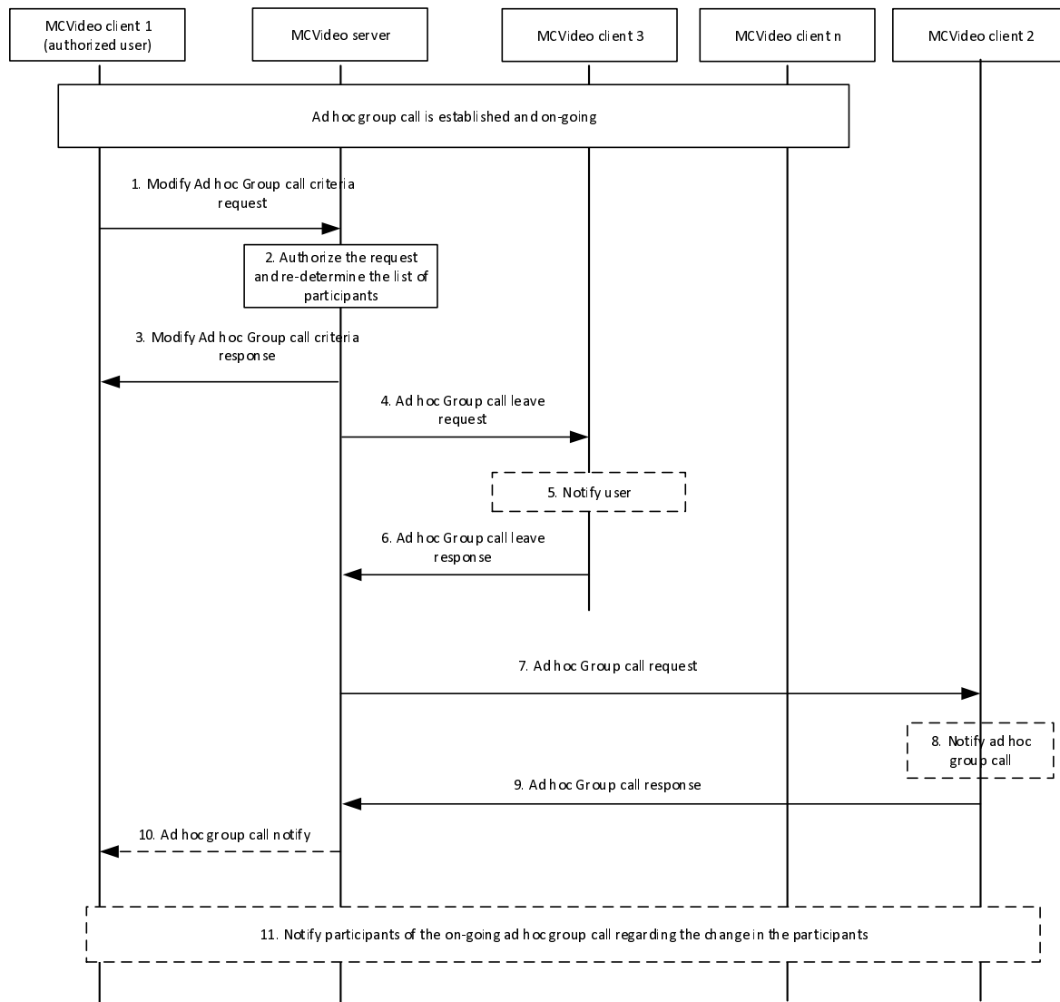
Figure 7.19.3.1.6-1: Modification of ad hoc group call criteria by the authorized user
