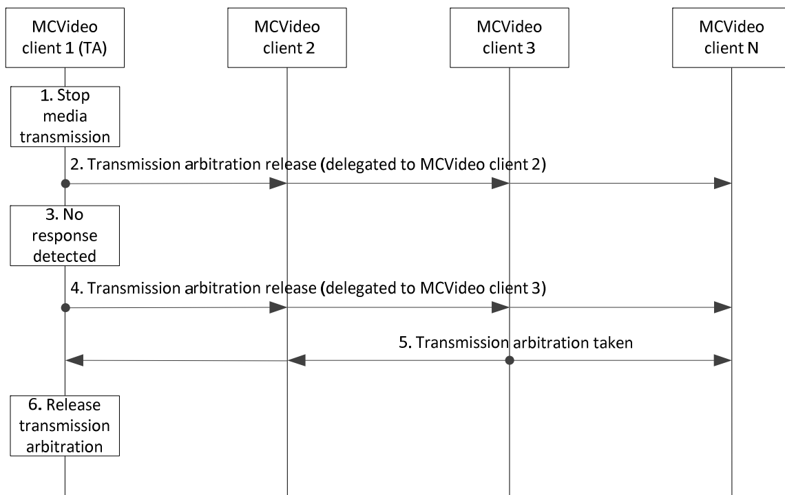
Figure 7.7.2.9.2-1: Transmission arbitration release with delegation
