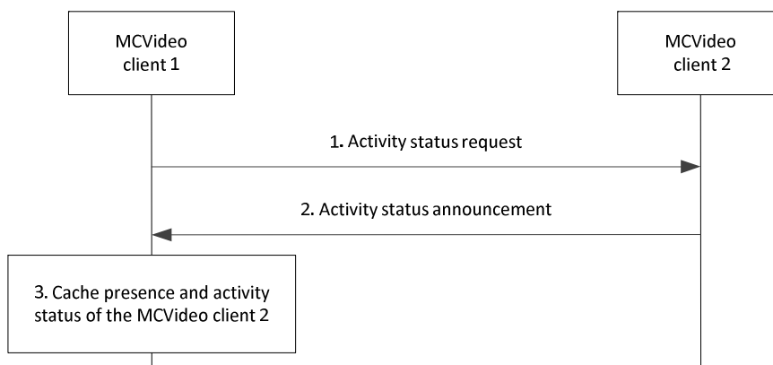
Figure 7.5.3.5.3-1: Request activity status from a particular client
