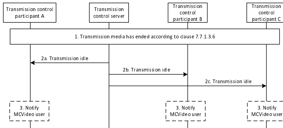
Figure 7.7.1.3.8-1: Transmission idle
