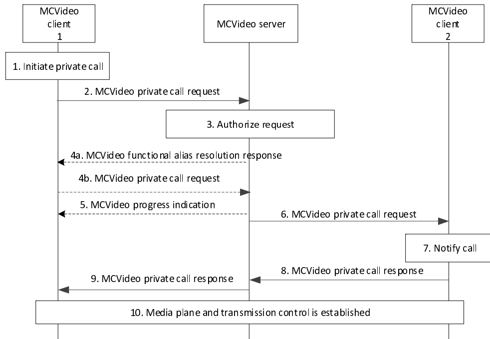
Figure 7.2.2.3.1-1: Private call setup in automatic commencement mode– MCVidéo users in the same MC system
