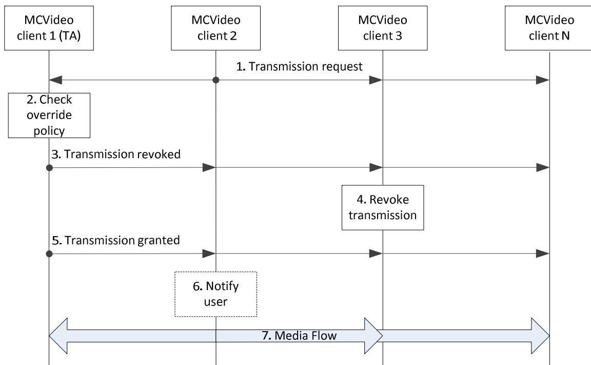
Figure 7.7.2.7-1: Transmission override
