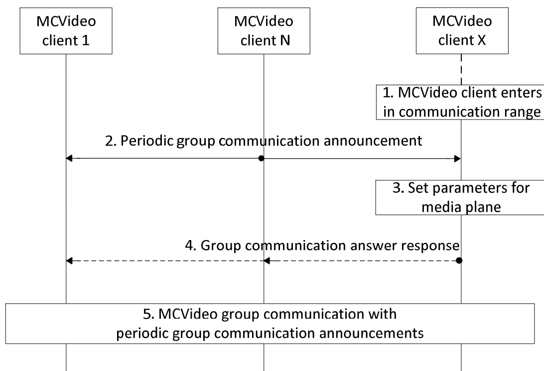
Figure 7.1.3.4.2-1: Passive join to MCVidéo group communication
