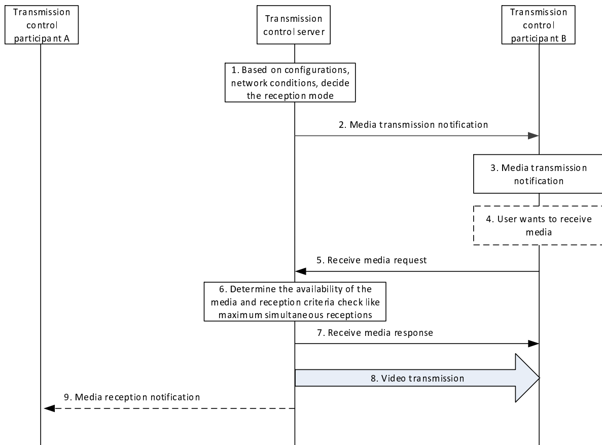
Figure 7.7.1.3.2-1: Reception control during an MCVideo session
