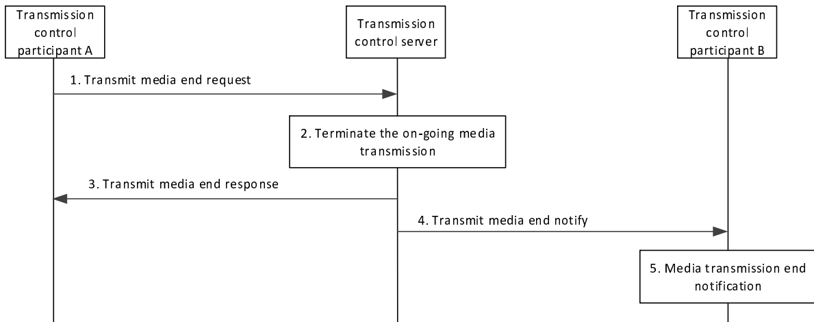
Figure 7.7.1.3.6.1-1: End a media transmission by an MCVidéo user
