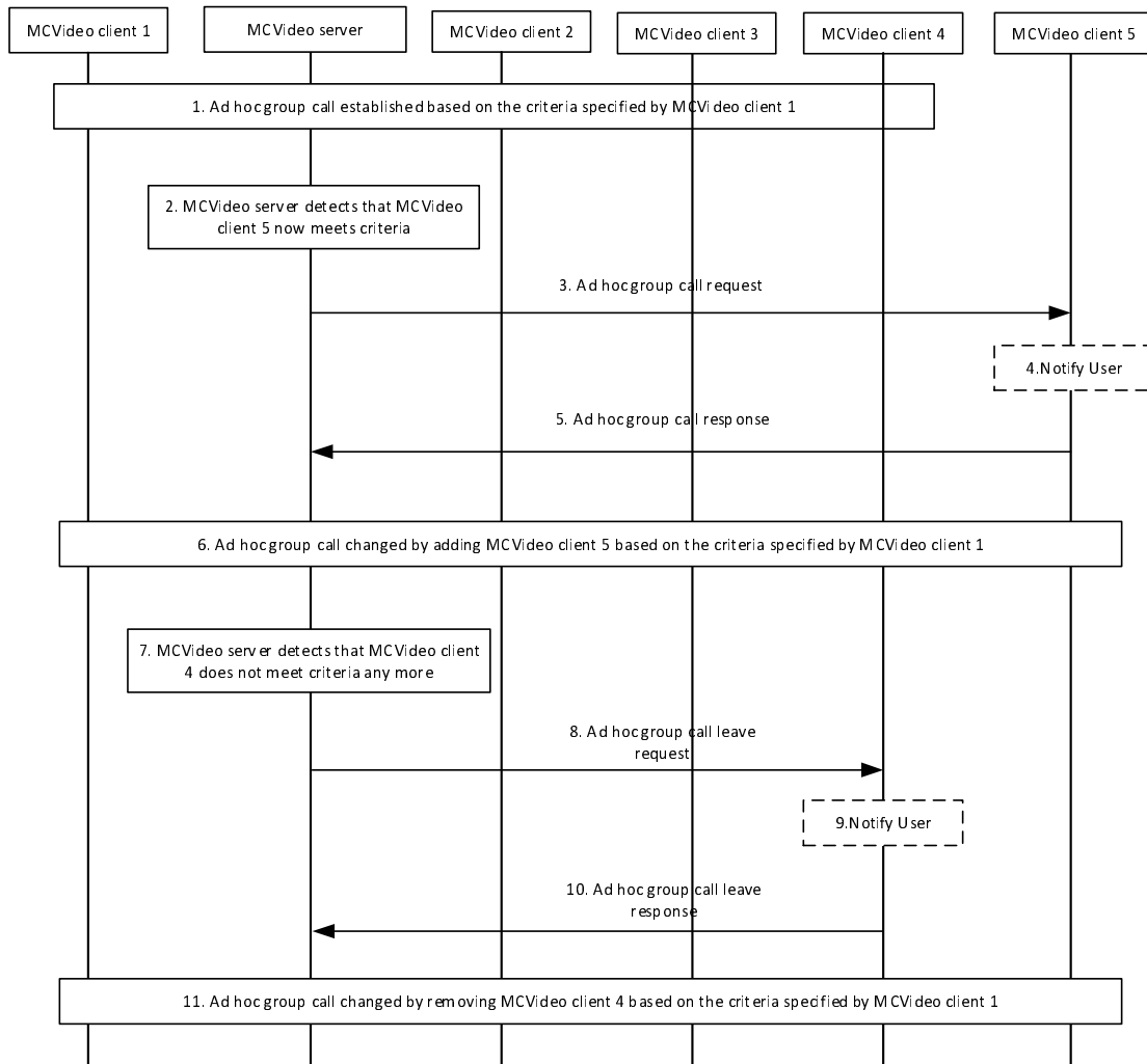
Figure 7.19.3.1.5-1: Modification of ad hoc group call participants by the MCVideo server
