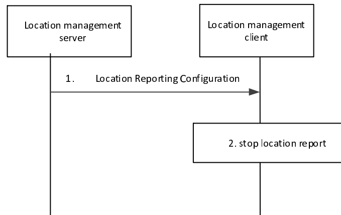
Figure 10.9.3.4-1: Location reporting cancel procedure
