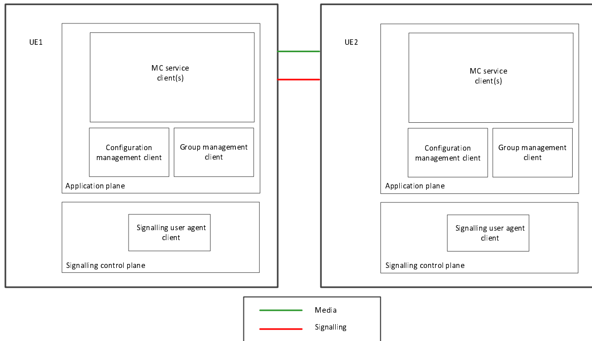
Figure 7.3.2-1: Functional model for MC service off-network operation
