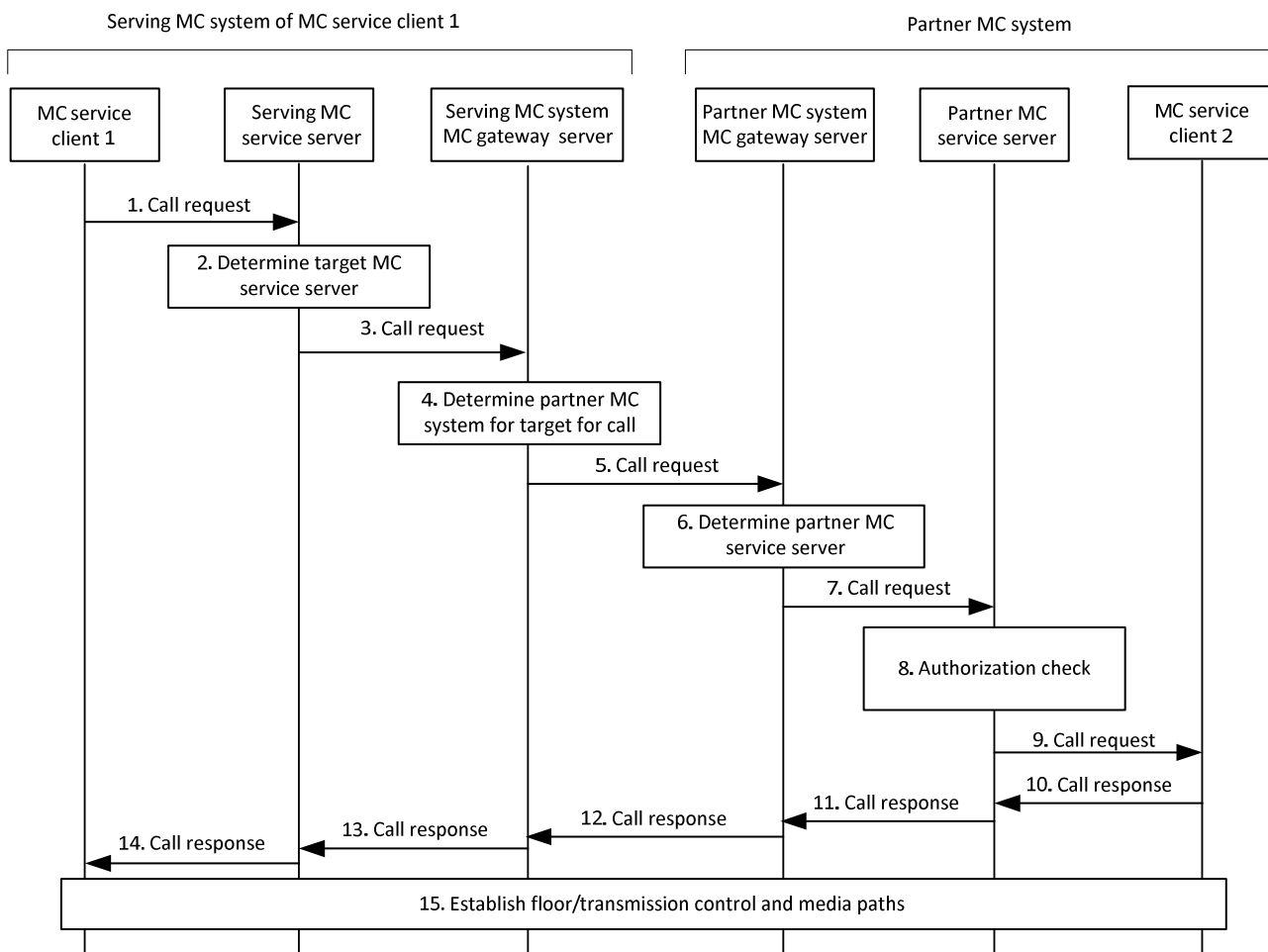
Figure 10.14.2.2-1: Call to target in interconnected MC system
