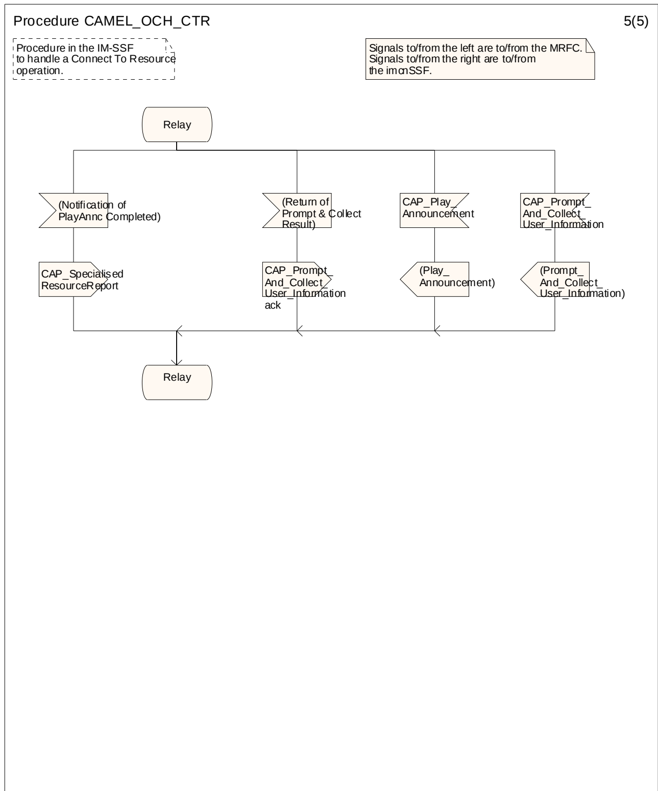
Figure 4.21-5: Procedure CAMEL_OCH_CTR (sheet 5)
