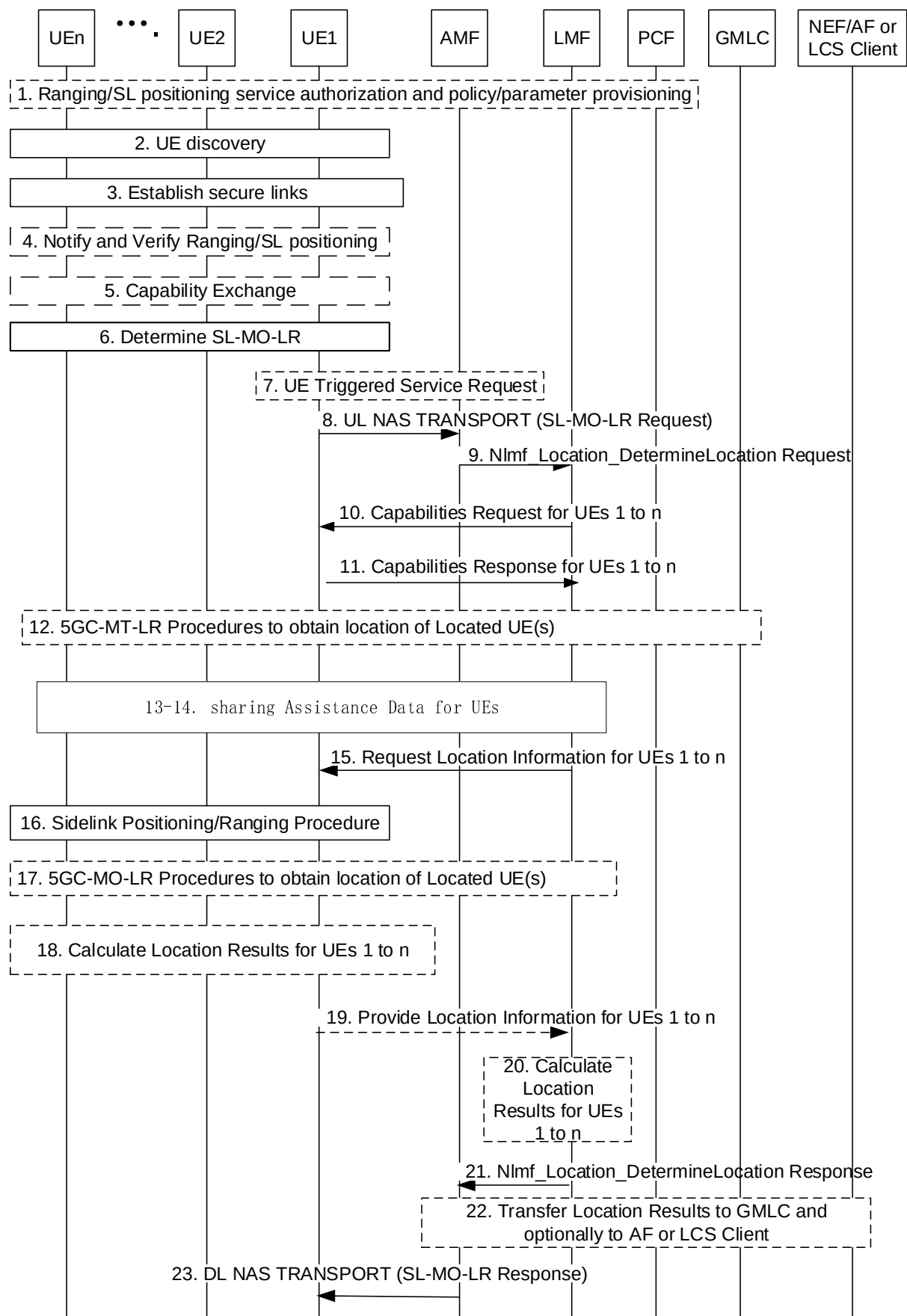
Figure 6.20.1-1: SL-MO-LR Procedure
