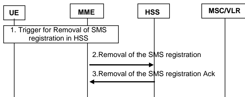
Figure C.8.2-2: Removal of MME registration for SMS in HSS
