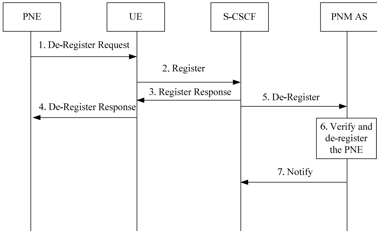
Figure 5.2.4-1: PN-deregistration procedure for PNE other than a PN UE
