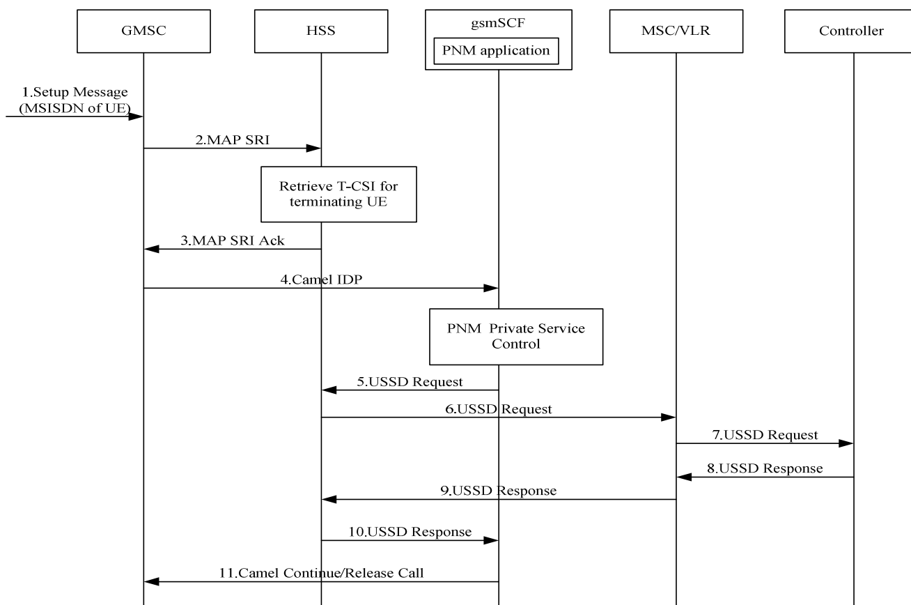
Figure 7.4.2-1: PN access control Procedure in CS domain
