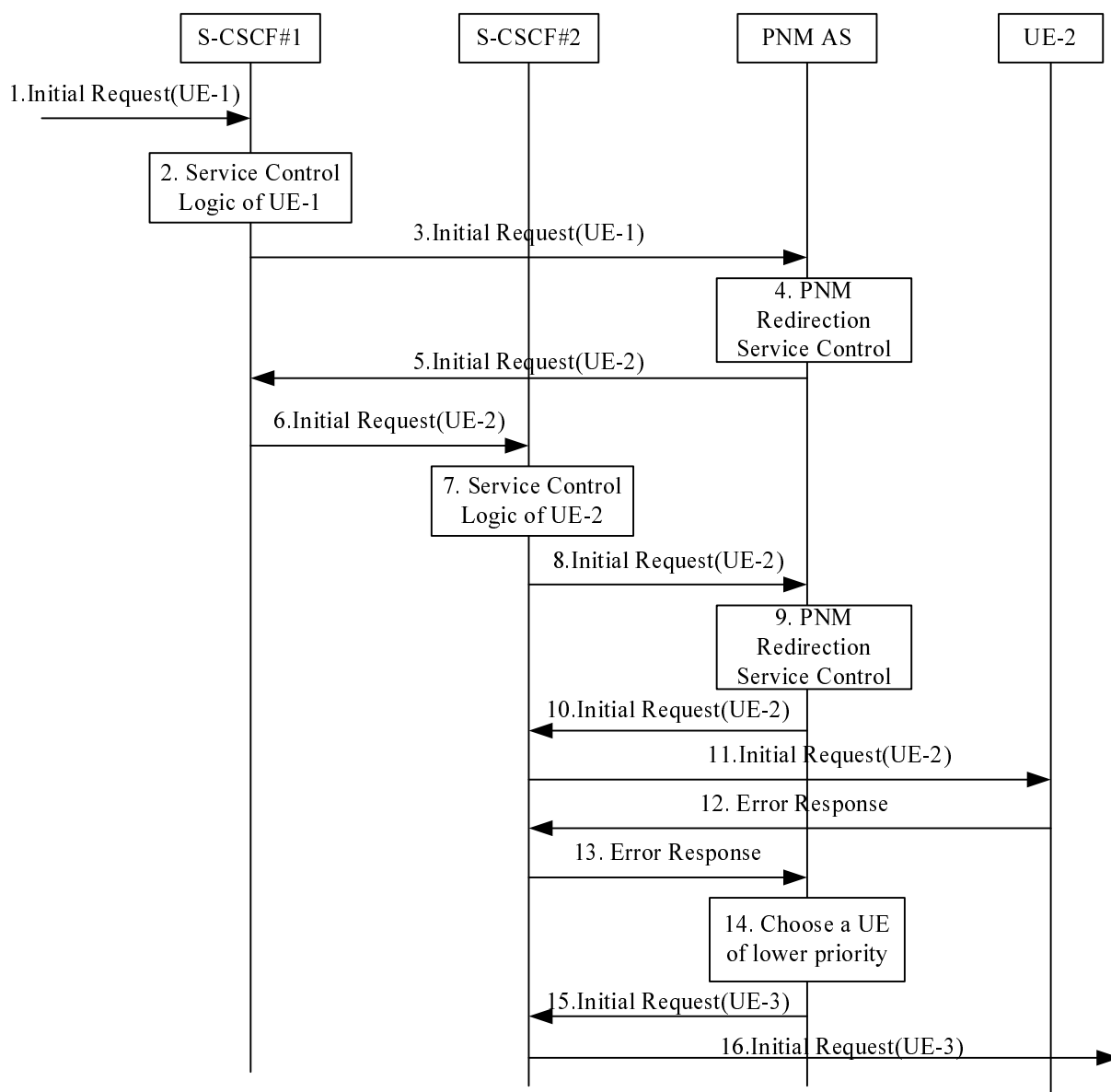
Figure 6.1.2-3: Initial request to UE-1 and redirected to UE-3 by the PNM AS in the IM CN subsystem when the initial request to UE-2 fails
