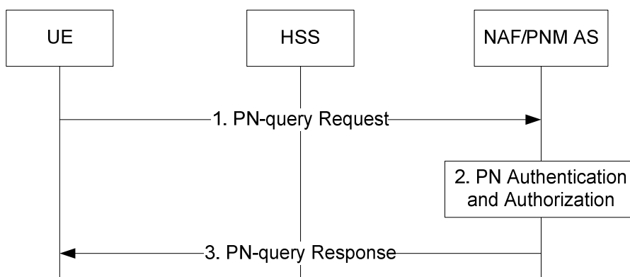
Figure 5.5.2-1: Successful PN query procedure in the IM CN subsystem
