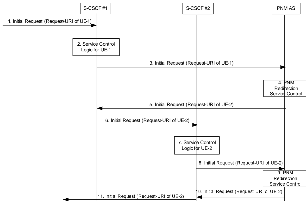
Figure 6.1.2-1: Initial request to UE-1 and redirected to UE-2 by the PNM AS in the IM CN subsystem
