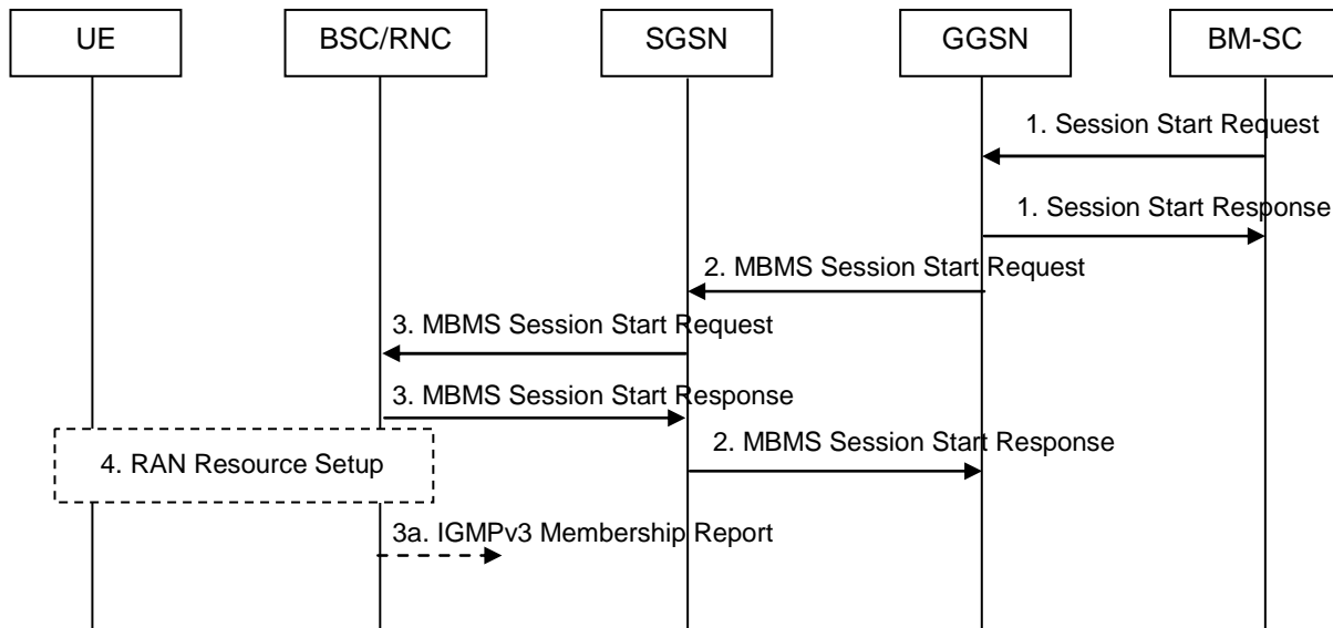
Figure 8: Session Start procedure for GERAN and UTRAN
