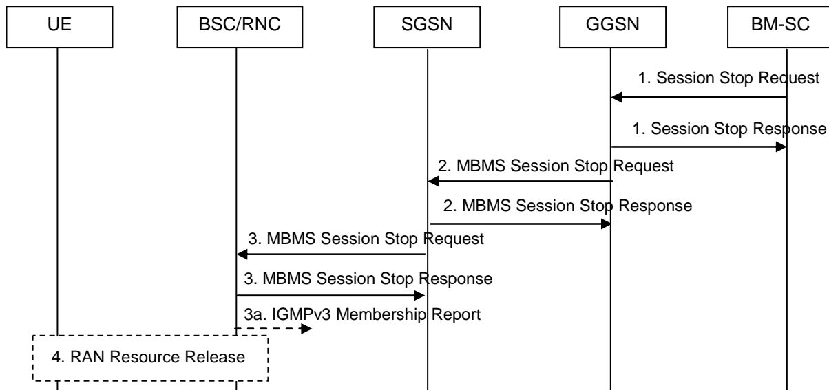
Figure 10: MBMS Session Stop procedure for GERAN and UTRAN
