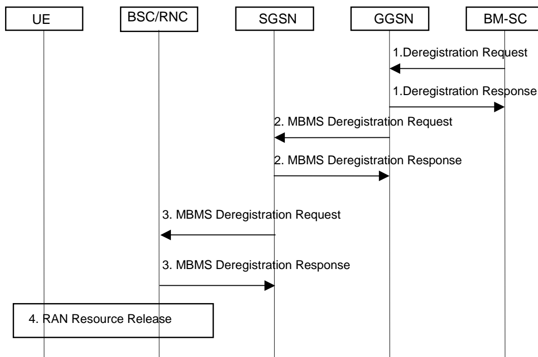
Figure 12: BM-SC initiated MBMS De-Registration Procedure
