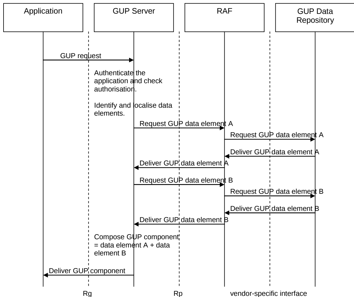
Figure 4.5: An Example of Application requesting GUP data component(s) message flow (Proxy mode)
