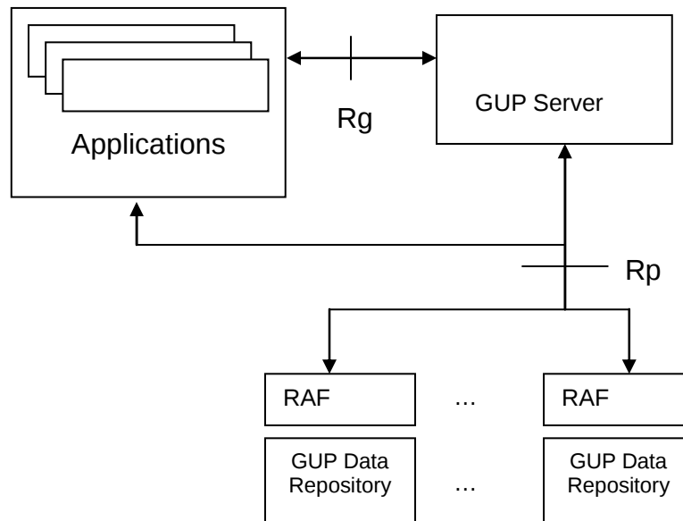
Figure 4.1: GUP reference architecture
