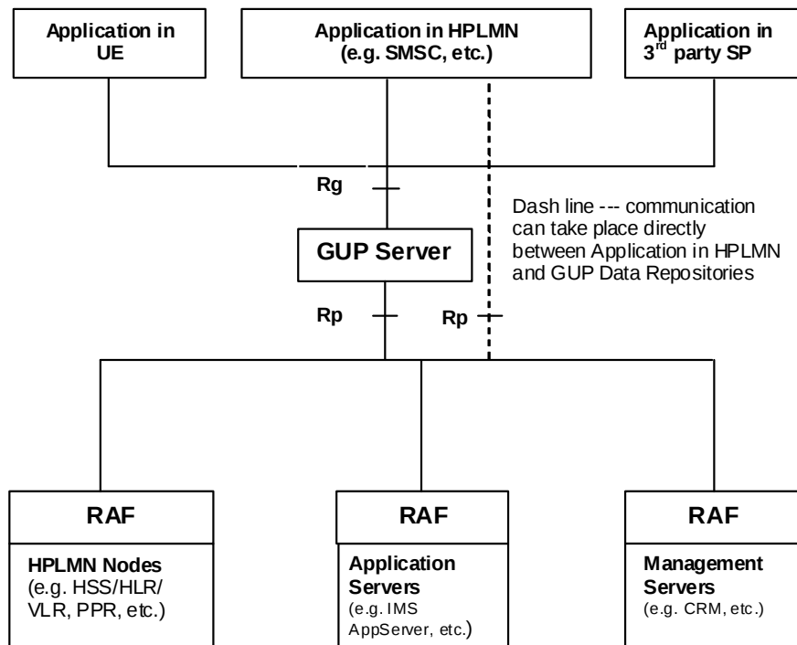
Figure 4.2: An example of mapping the GUP reference architecture to current infrastructure environment
