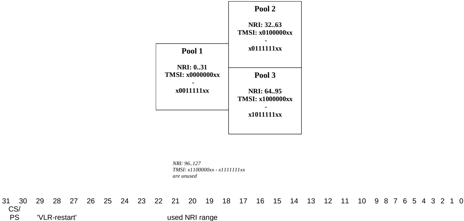
Figure 11: Modified TMSI structure 7 bits NRI-length; VLR-restart field must be reduced to 3 bit
