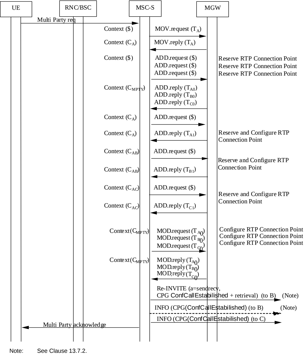
Figure 13.7.6.2: Information flow for multi party call, internal IP bearer (message sequence chart)
