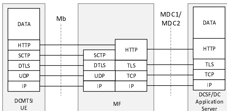
Figure AC.6-1: MF "HTTP Proxy" Media Configurations
