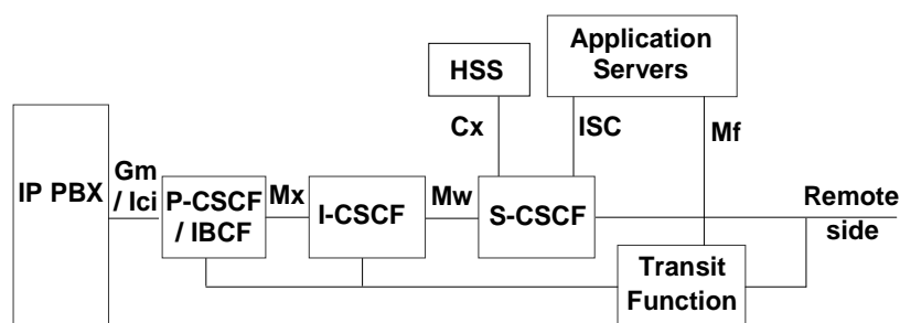
Figure S.2-1: High level Static mode business trunking Architecture
