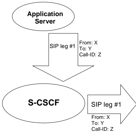
Figure 4.3b: Application Server acting as originating UA
