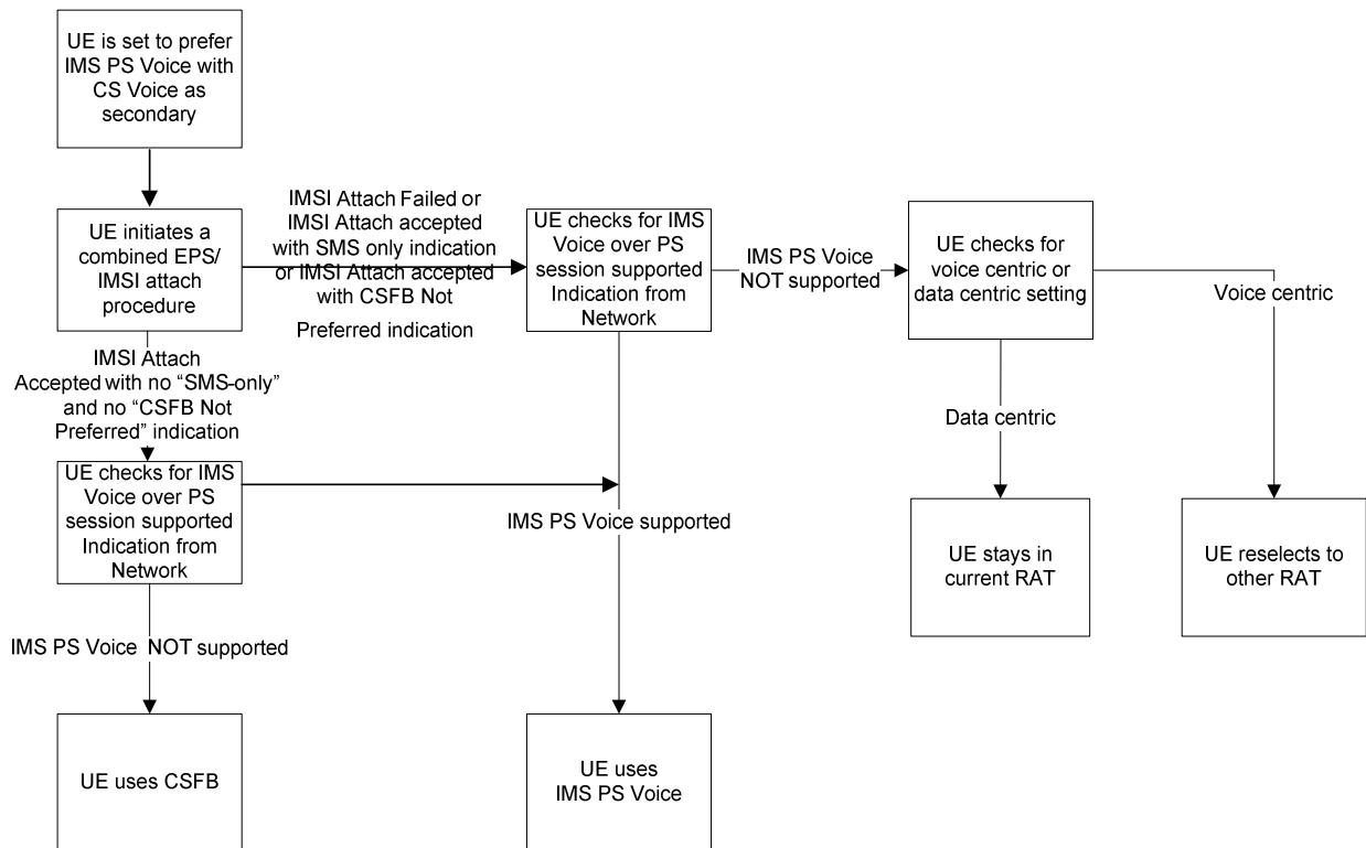
Figure A.2.2-1: UE behaviour for IMS PS Voice preferred with CS Voice as secondary, combined EPS/IMSI attach
