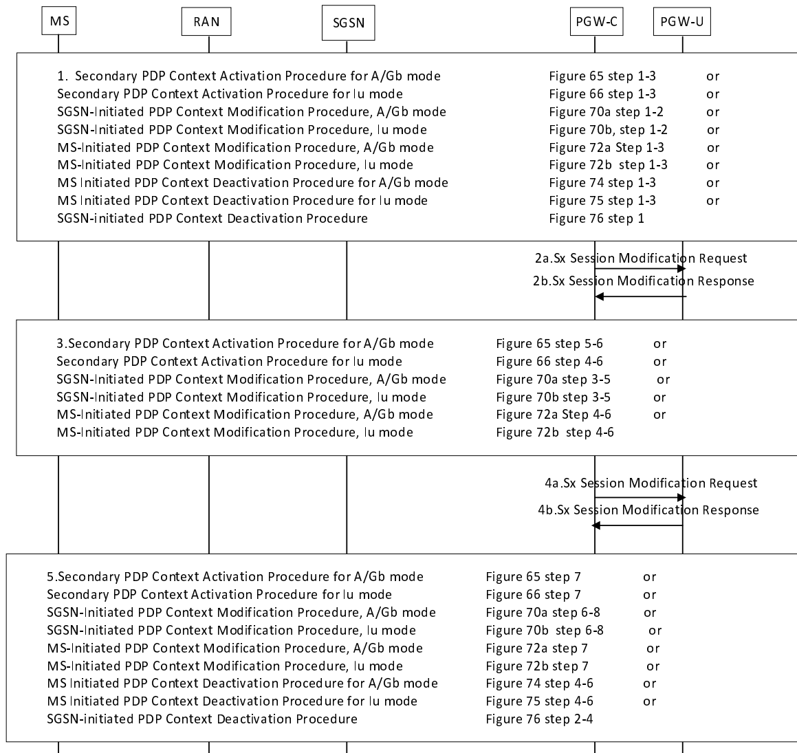
Figure 6.3.4.2.2-2: Interaction between CP and UP function with PDN connection modification, Group 2
