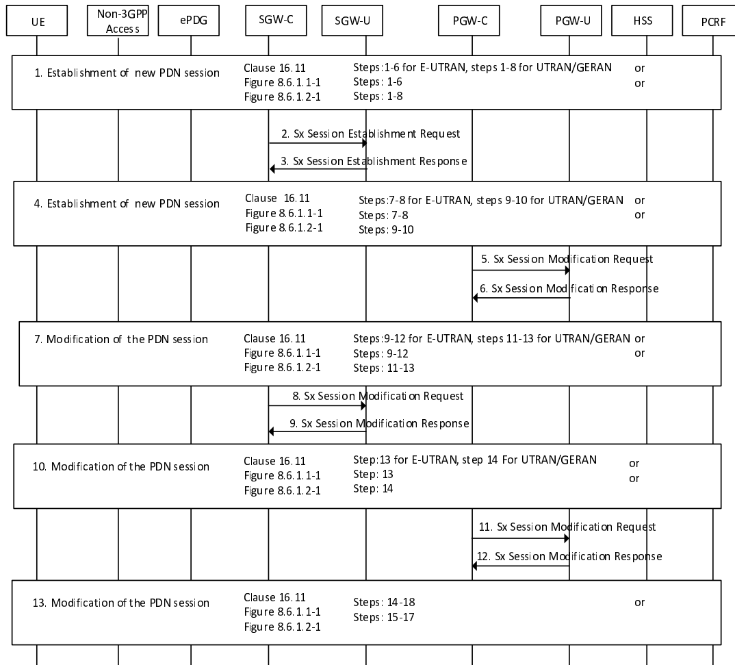
Figure 6.3.3.8-1: Interaction between CP and UP function with handover from non-3GPP access
