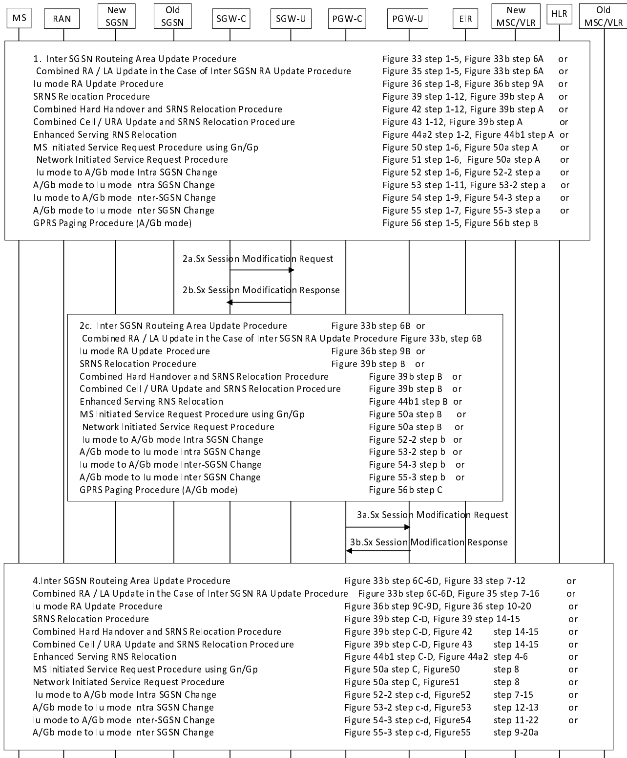
Figure 6.3.4.2.1-1: Interaction between CP and UP function with PDN connection modification, Group 1
