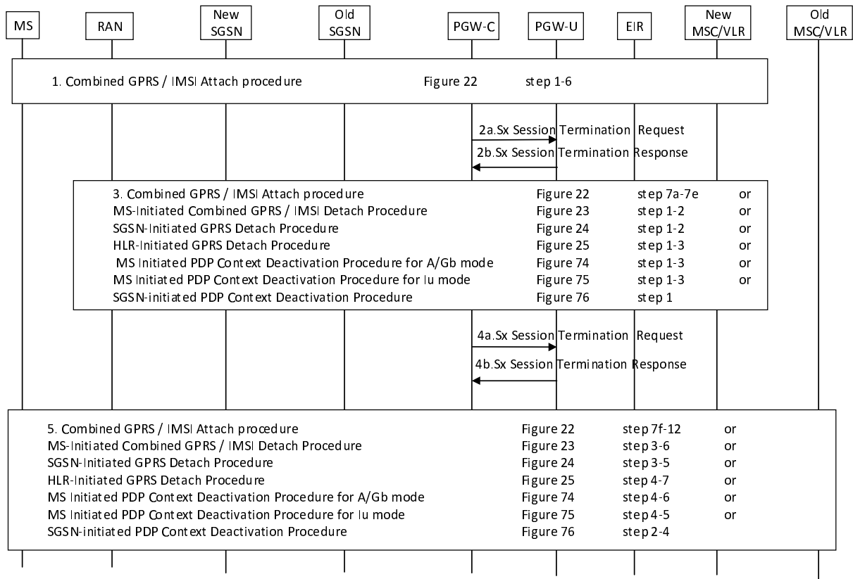
Figure 6.3.4.1.2-1: Interaction between CP and UP function with PDN connection deactivation Group 1
