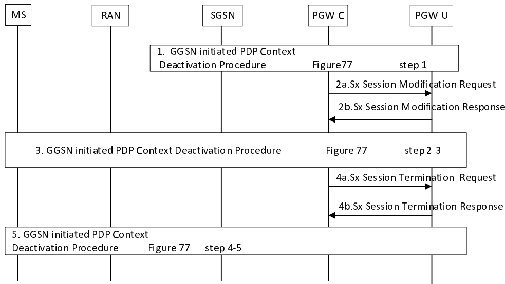
Figure 6.3.4.1.2-2: Interaction between CP and UP function with PDN connection deactivation Group 2
