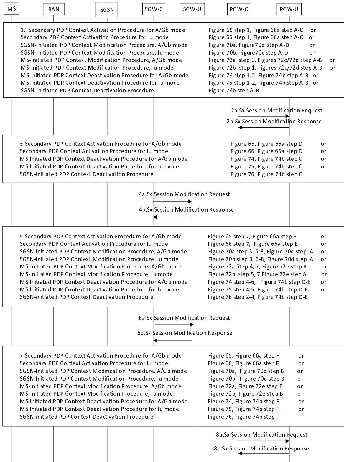
Figure 6.3.4.2.1-2: Interaction between CP and UP function with PDN connection modification, Group 2
