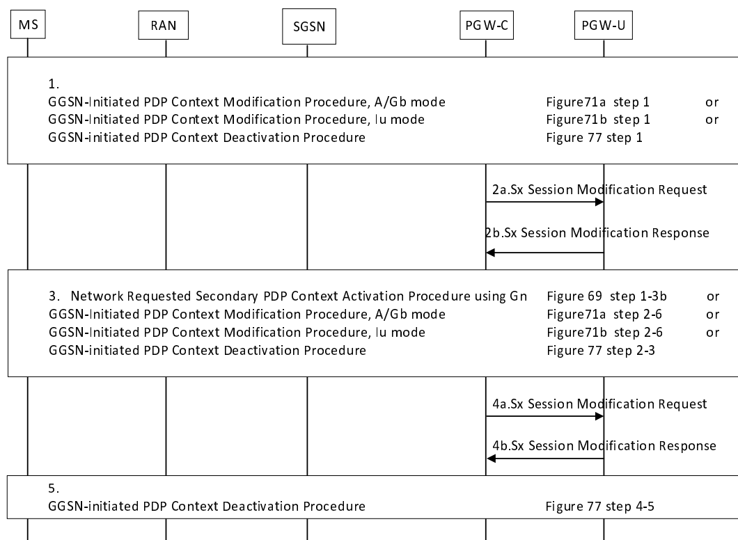
Figure 6.3.4.2.2-3: Interaction between CP and UP function with PDN connection modification, Group 3
