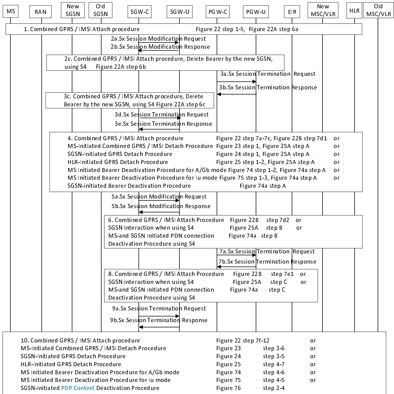
Figure 6.3.4.1.1-1: Interaction between CP and UP function with PDN connection deactivation Group 1
