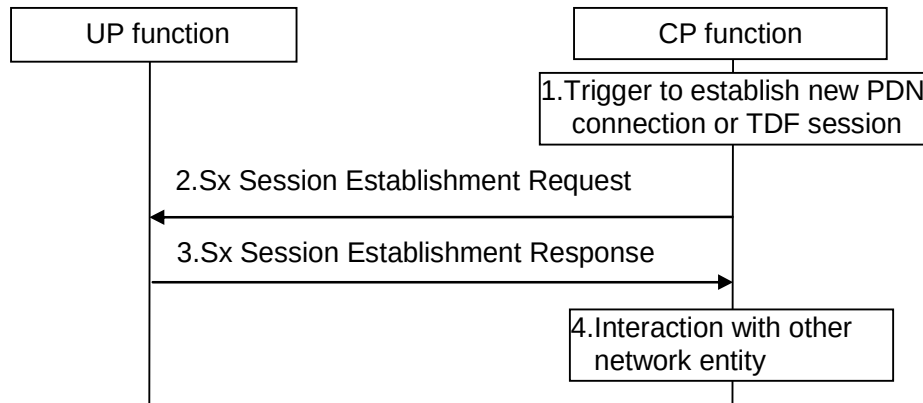
Figure 6.2.2-1 Sx session establishment procedure
