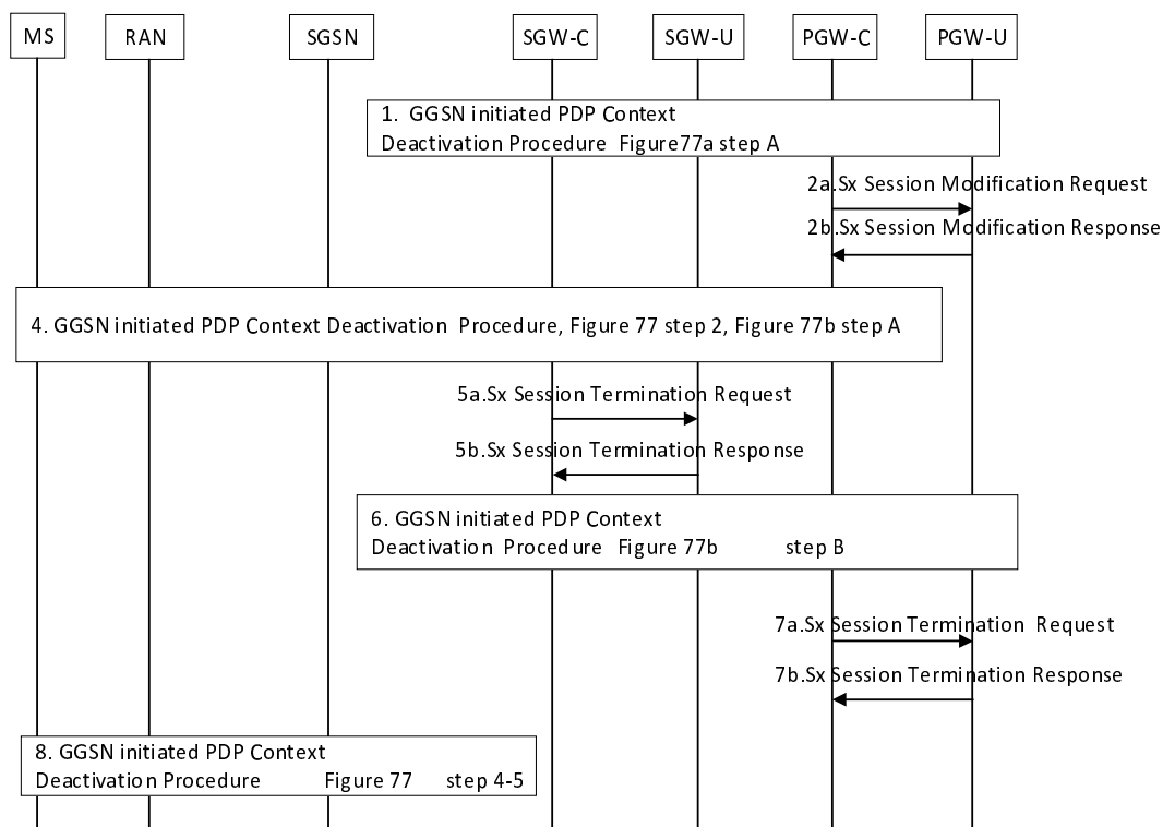
Figure 6.3.4.1.1-2: Interaction between CP and UP function with PDN connection deactivation Group 2
