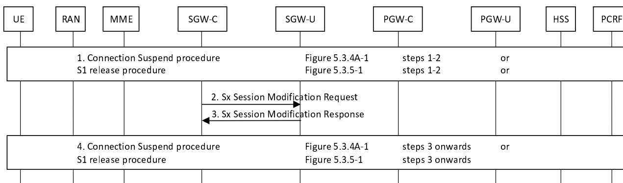
Figure 6.3.1.4-1: Interaction between CP and UP function during procedures with release of eNB F-TEIDu
