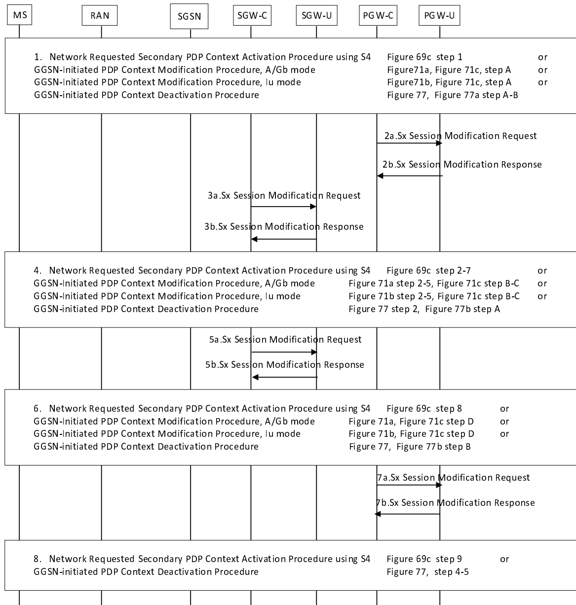
Figure 6.3.4.2.1-3: Interaction between CP and UP function with PDN connection modification, Group 3
