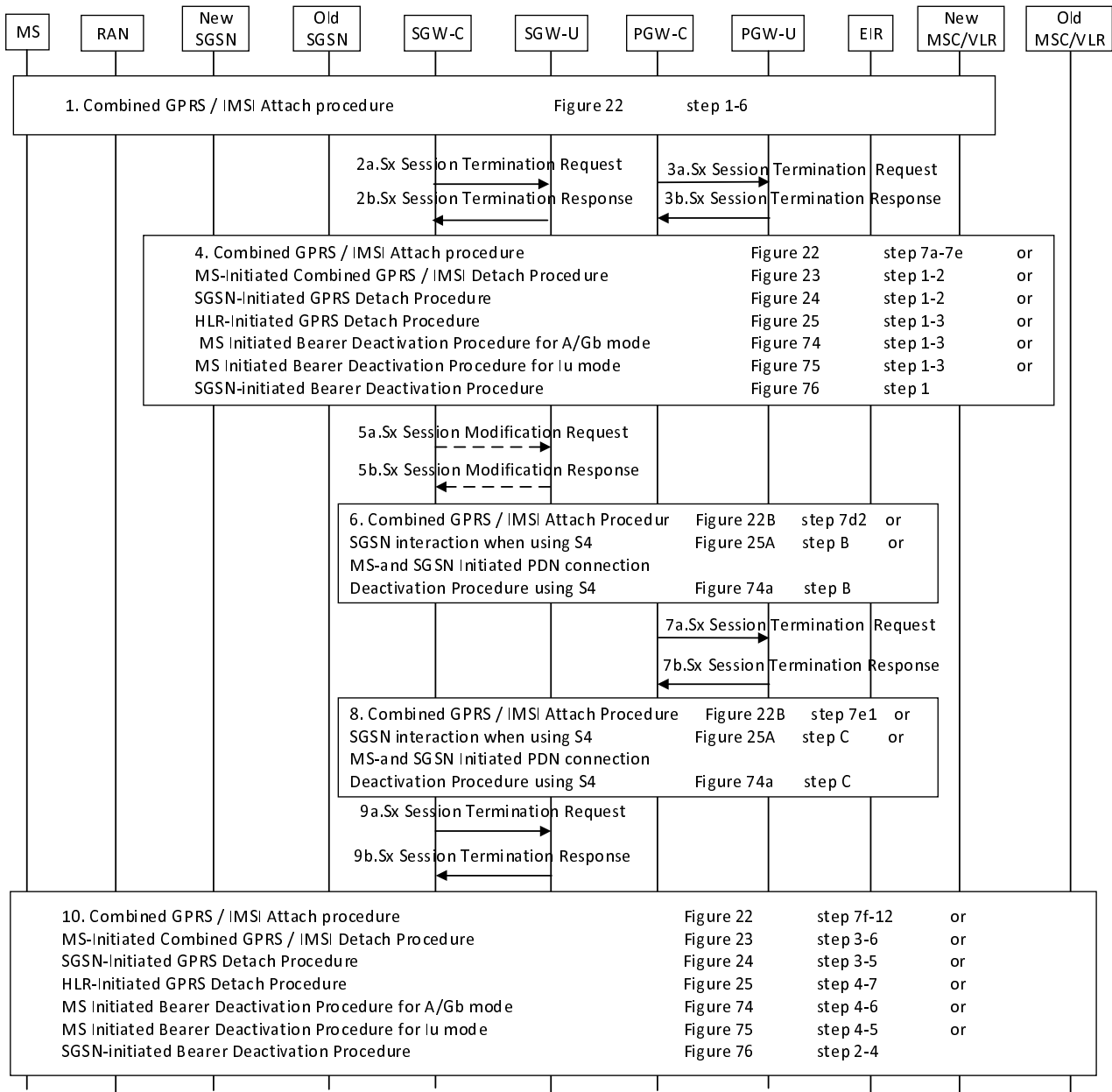
Figure 6.3.4.1.1-1: Interaction between CP and UP function with PDN connection deactivation part 1
