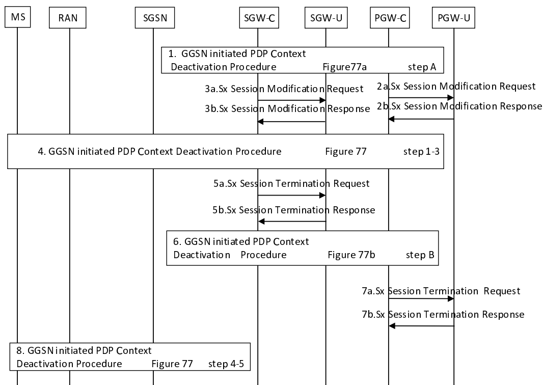
Figure 6.3.4.1.1-2: Interaction between CP and UP function with PDN connection deactivation part 2
