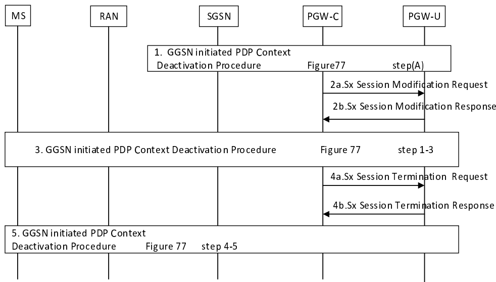
Figure 6.3.4.1.2-2: Interaction between CP and UP function with PDN connection deactivation part 2
