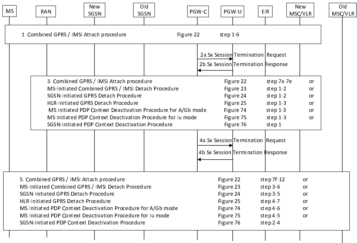
Figure 6.3.4.1.2-1: Interaction between CP and UP function with PDN connection deactivation part 1
