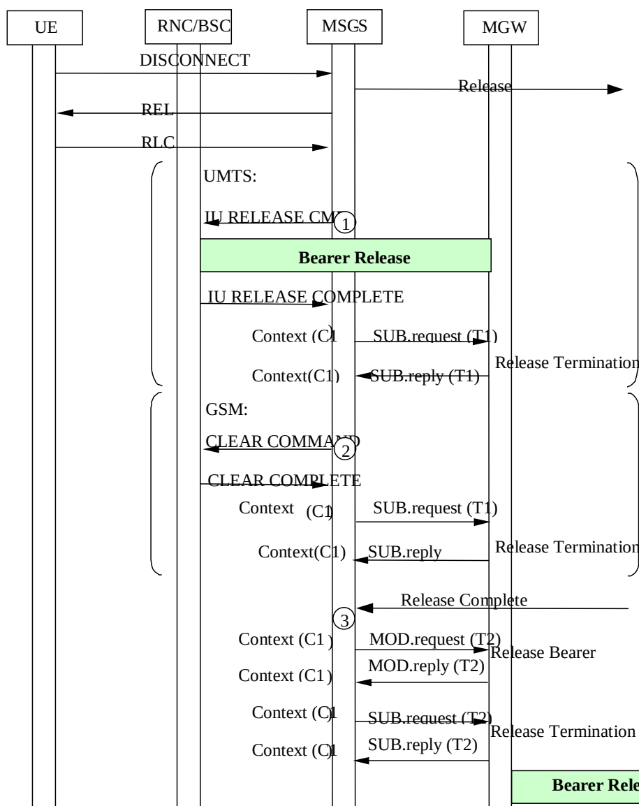
Figure 7.4: User Initiated Call Clearing (message sequence chart)
