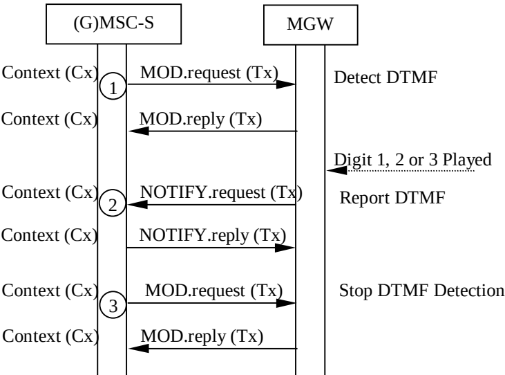
Figure 14.5: Inband DTMF detection (message sequence chart)
