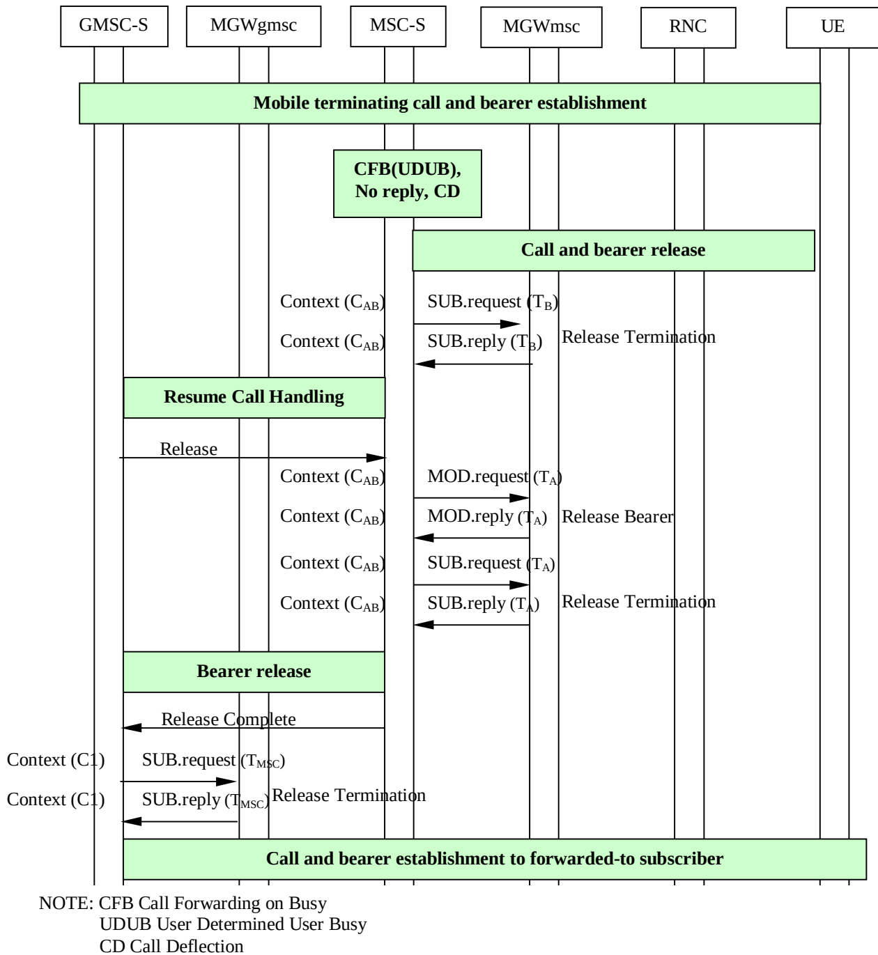
Figure 14.11: Optimal call routing; late call forwarding (CFB (UDUB), CFNRy, CD), backward bearer release (message sequence chart)
