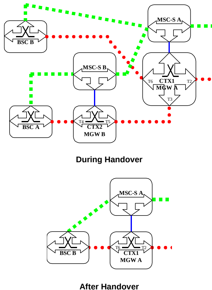
Figure 8.23: Subsequent Inter-MSC GSM to GSM Handover back to the Anchor MSC (network model)
