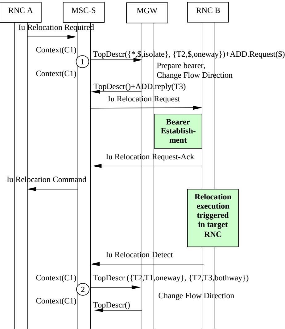
Figure 8.2/1: Intra-MSC SRNS Relocation (message sequence chart)
