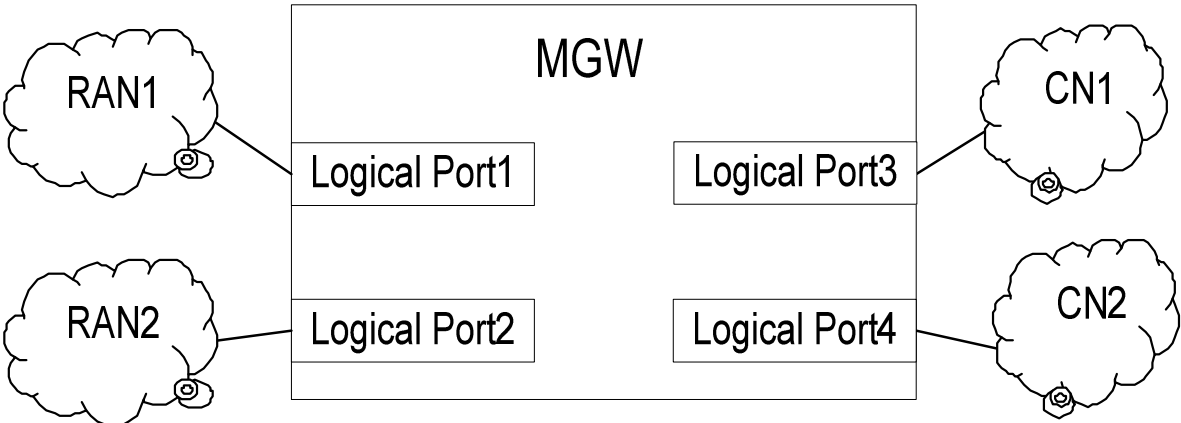
Figure 20/1 Multiple IP realms scenario for Iu or Nb interface
