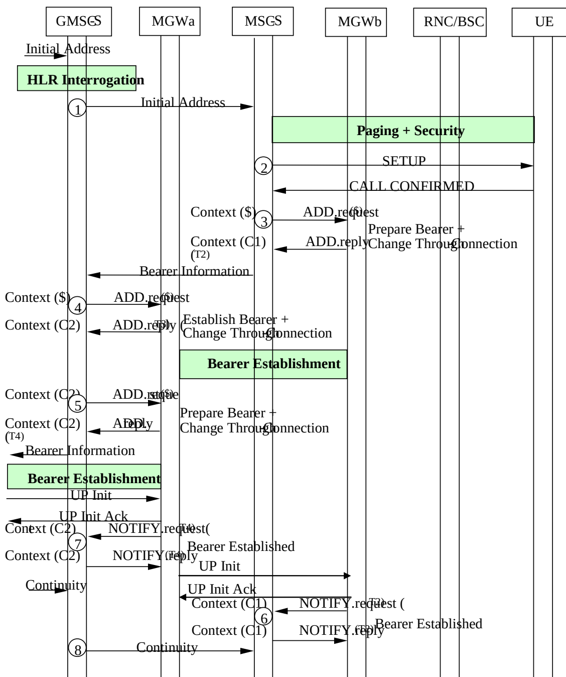
Figure 6.6/1: Basic Mobile Terminating Call, Forward Bearer Establishment (message sequence chart)
