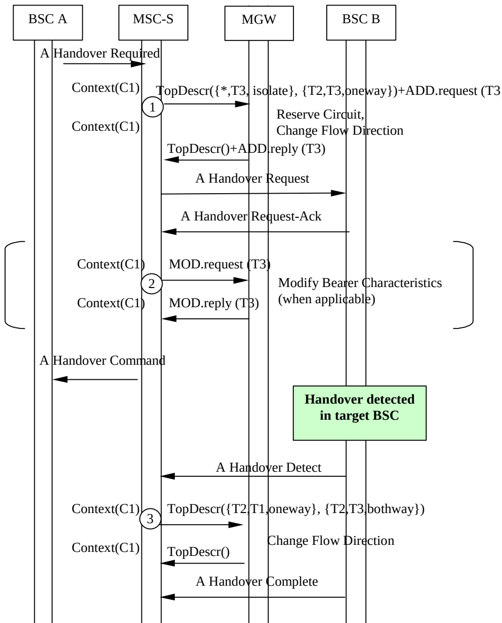
Figure 8.20/1: Intra-MSC GSM to GSM Handover (message sequence chart)
