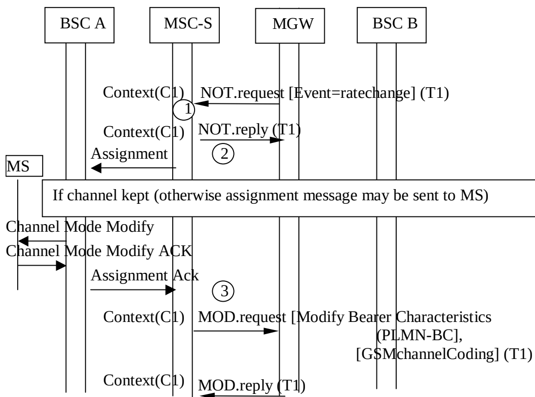
Figure 13.19/1: GSM access Channel Mode Modify message
