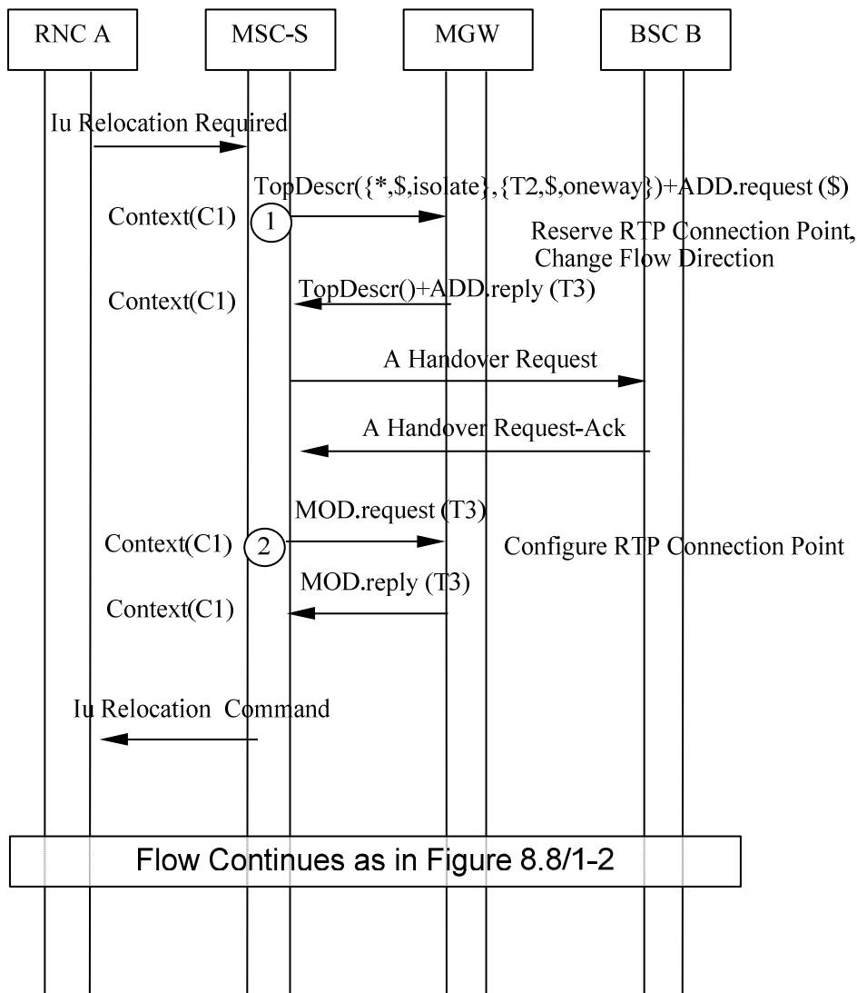
Figure 8.2.1.10/1: Intra-UMTS to GSM Handover for AoIP (message sequence chart)
