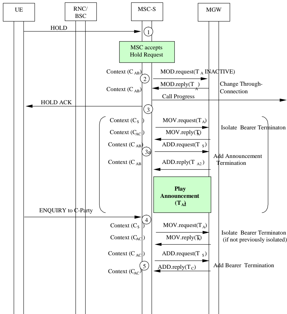
Figure 13.17: Hold request (message reply) sequence chart , example 1
