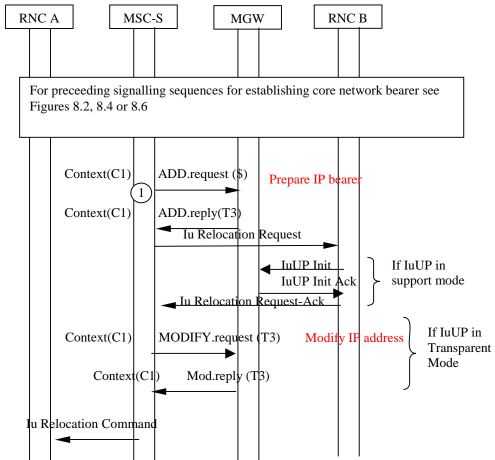
Figure 8.1.5/1 SRNS Relocation with lu on IP
