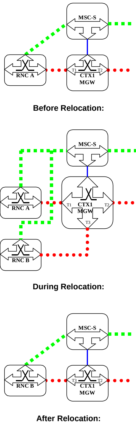
Figure 8.1: Intra-MSC SRNS Relocation (network model)
