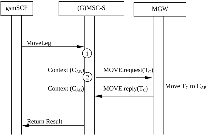
Figure 14. 1.3/4 Information flow for Move Leg (message sequence chart)
