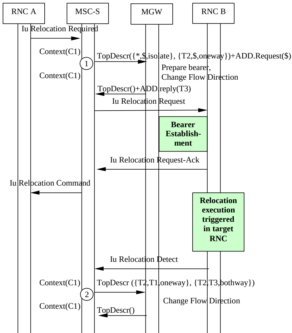
Figure 8.2/1: Intra-MSC SRNS Relocation (message sequence chart)
