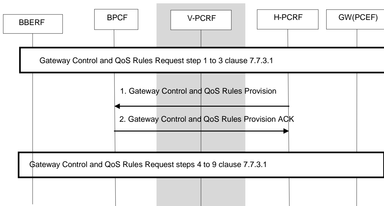
Figure P.7.5.3: Gateway Control and QoS Rule Request for EPC Routed Traffic
