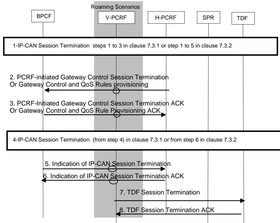
Figure P.7.3.2: IP-CAN Session Termination for either EPC routed or NSWO traffic
