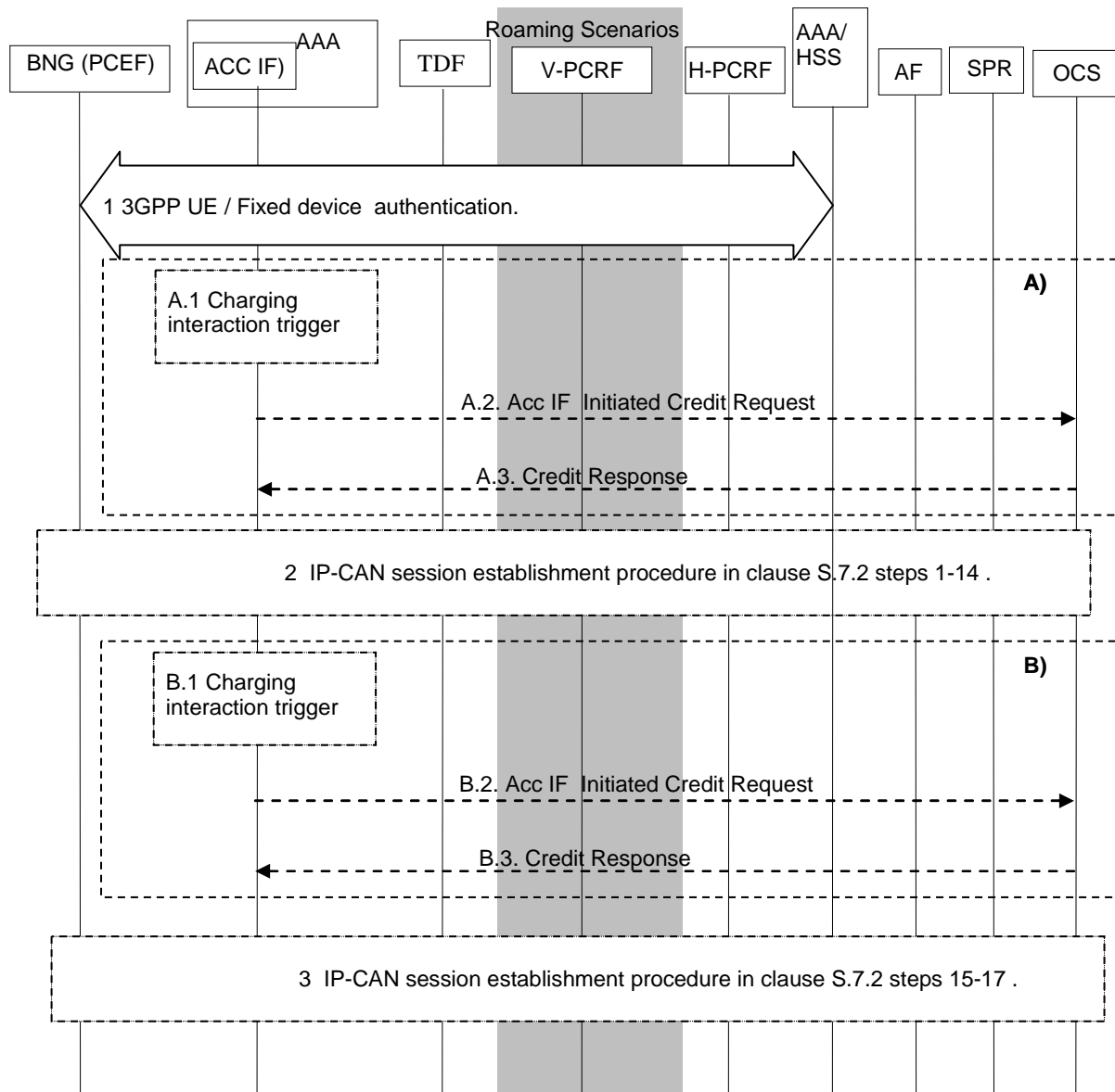
Figure S.8.8.1: AAA-based Charging Session Initiation
