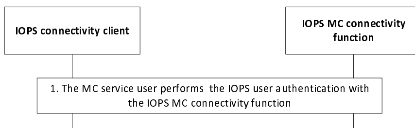
Figure 10.1.2-1 User authentication in the IOPS mode of operation
