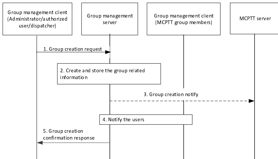
Figure 10.4.3-1: Group creation
