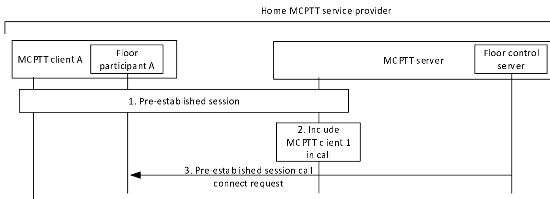
Figure 10.5.3.5.1-1: Connect procedure
