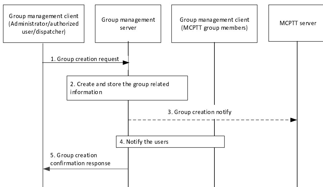
Figure 10.4.3-1: Group creation
