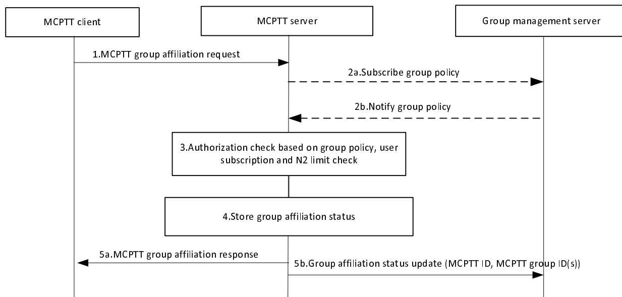
Figure 10.3.3.1-1: MCPTT group affiliation procedure
