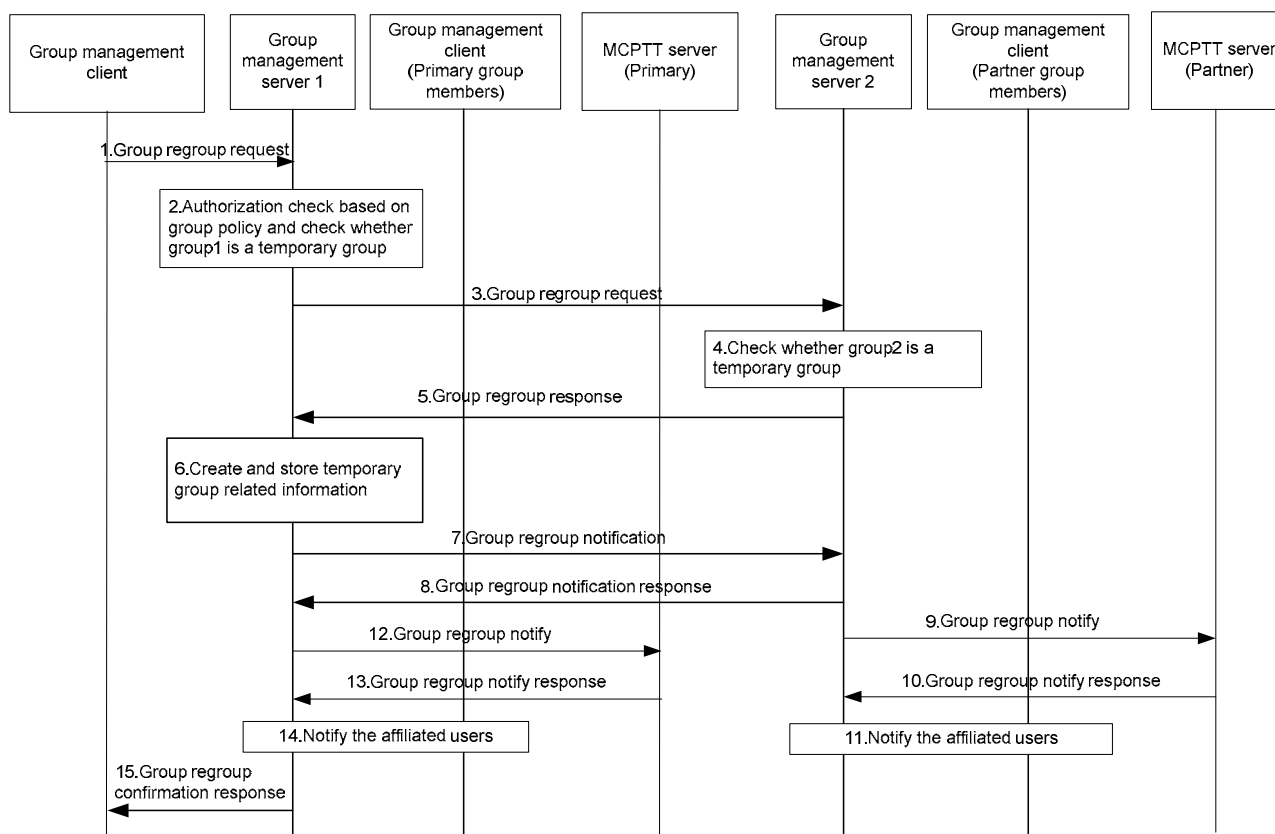
Figure 10.4.4.2-1: Temporary group formation - group regrouping involving multiple MCPTT systems
