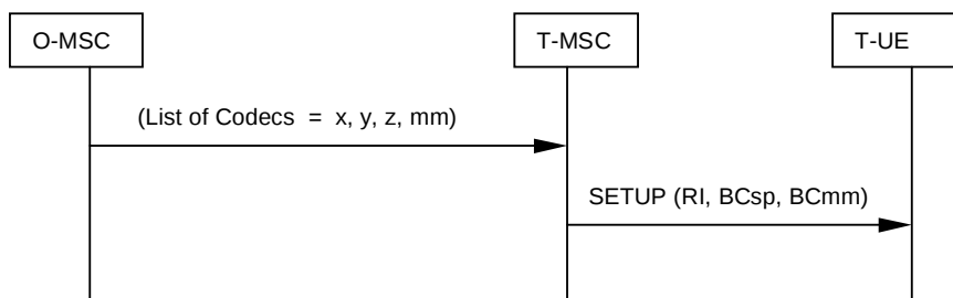
Figure 4.18: Speech codec first
