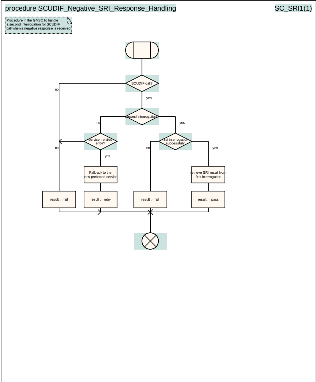
Figure 4.16l: Procedure SCUDIF_Negative_SRI_Response_Handling
