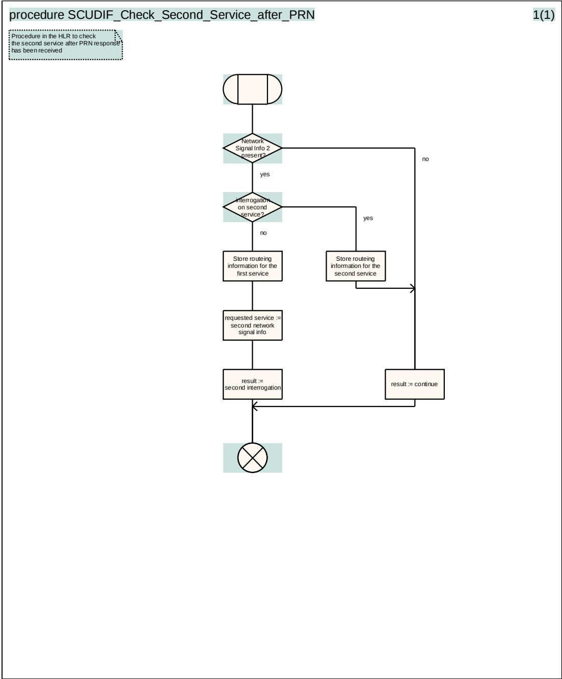
Figure 4.16G: Procedure SCUDIF_Check_Second_Service_after_PRN
