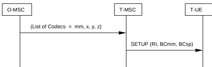
Figure 4.17: 3G-324M codec first
