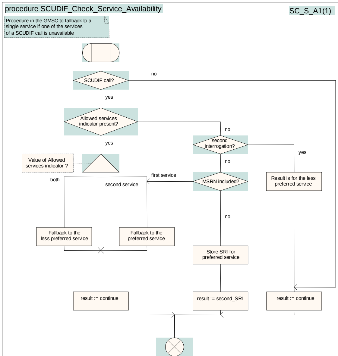
Figure 4.16J: Procedure SCUDIF_Check_Service_Availability
