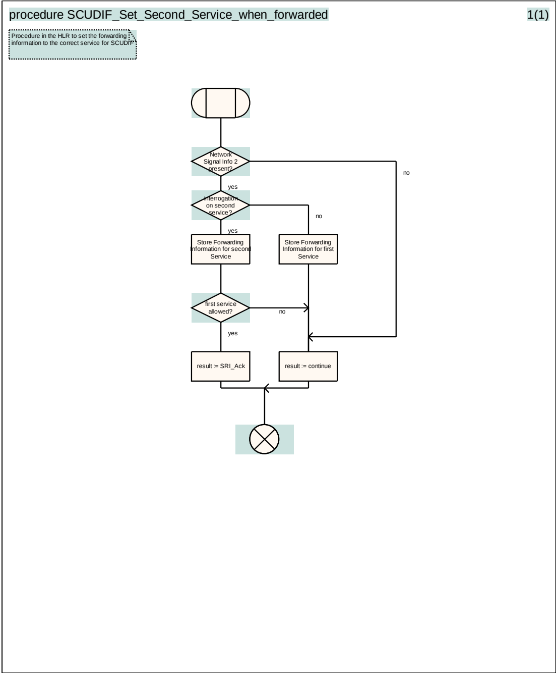
Figure 4.16D: Procedure SCUDIF_Set_Second_Service_when_Forwarded
