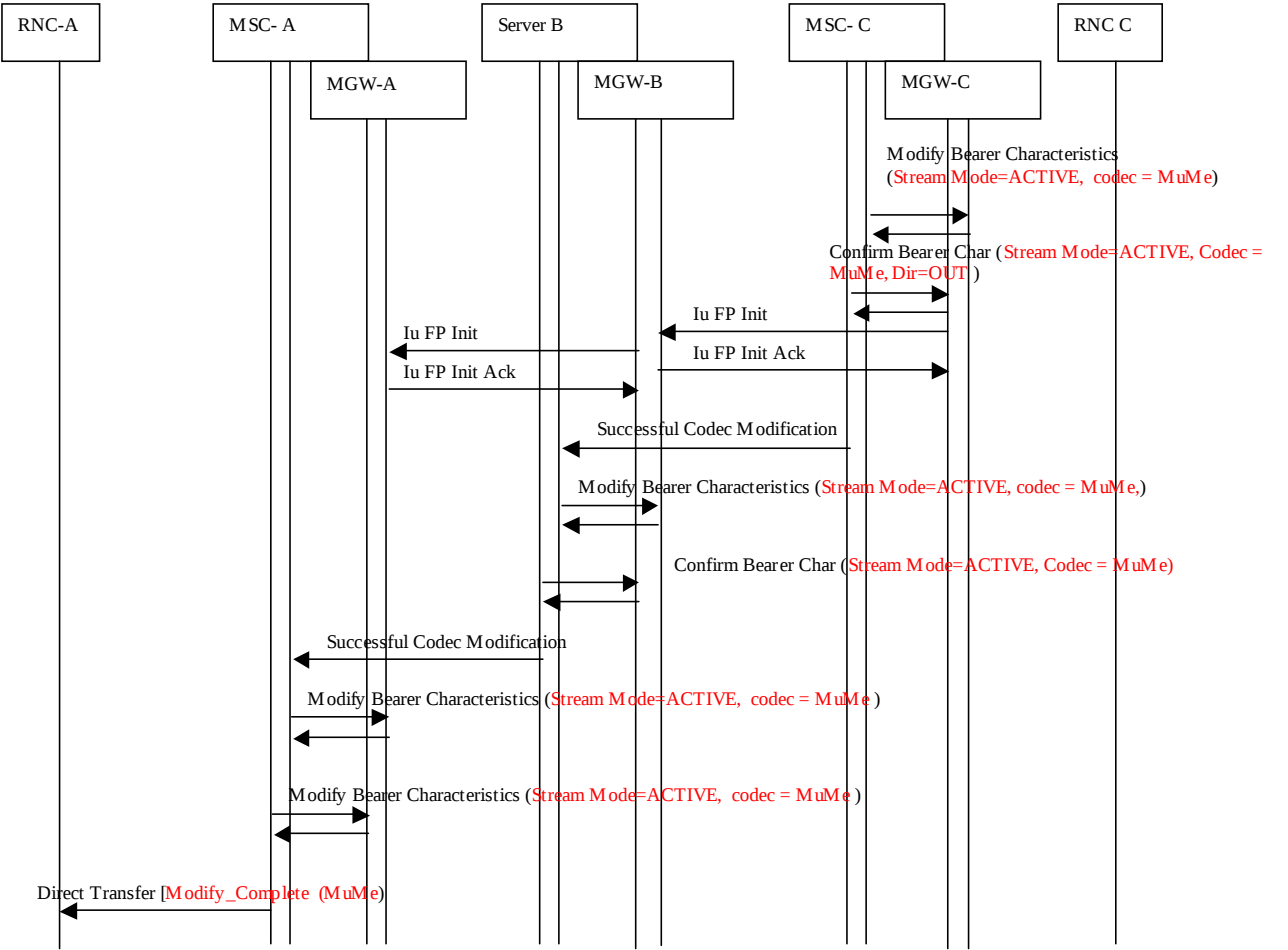
Figure 4.3.5.1/2: Service change speech to MuMe (continued)
