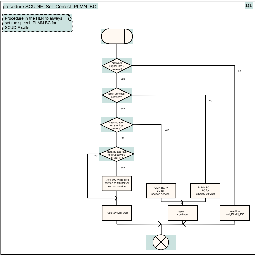
Figure 4.16E: Procedure SCUDIF_Set_Correct_PLMN_BC
