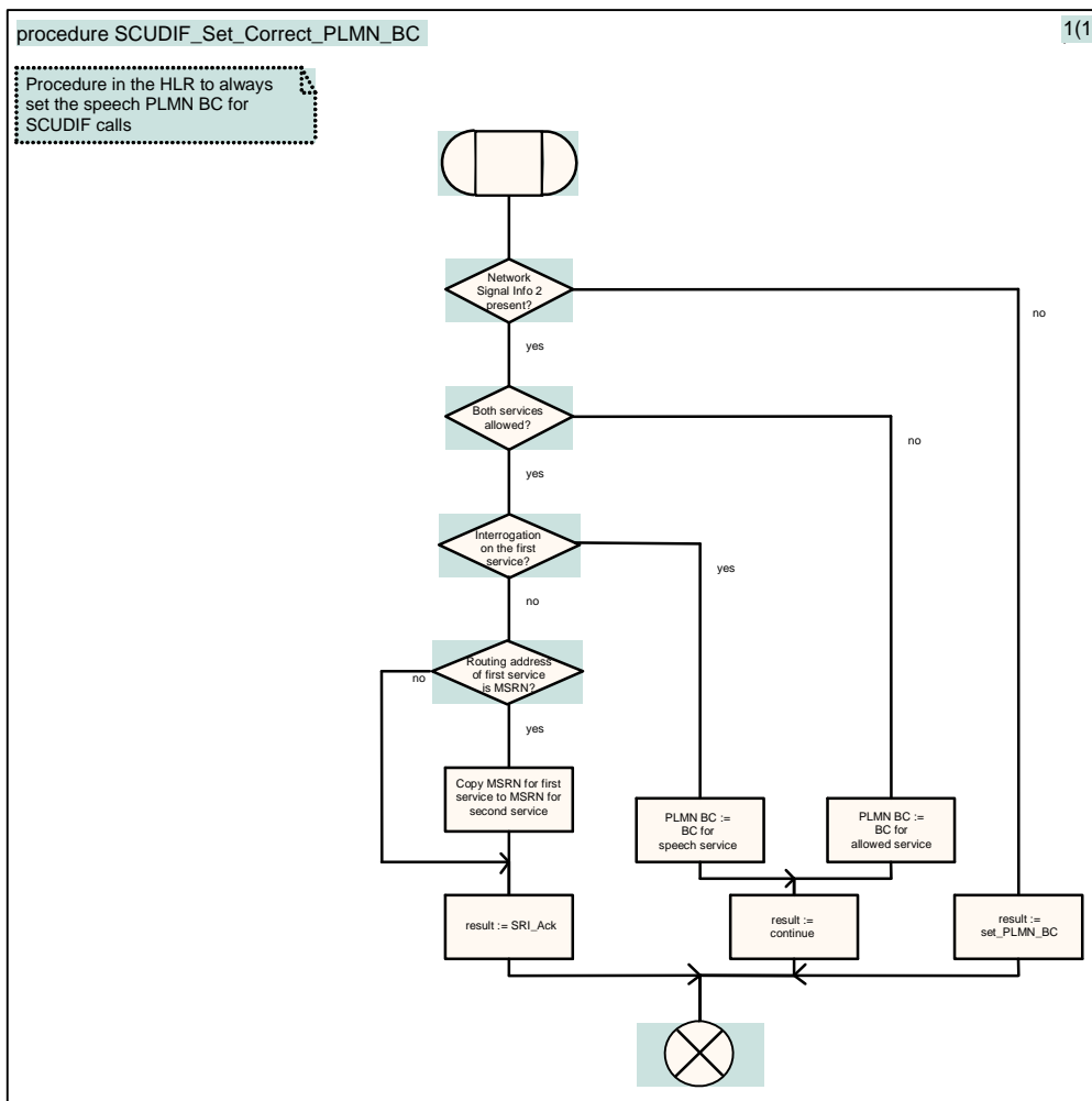
Figure 4.16E: Procedure SCUDIF_Set_Correct_PLMN_BC
