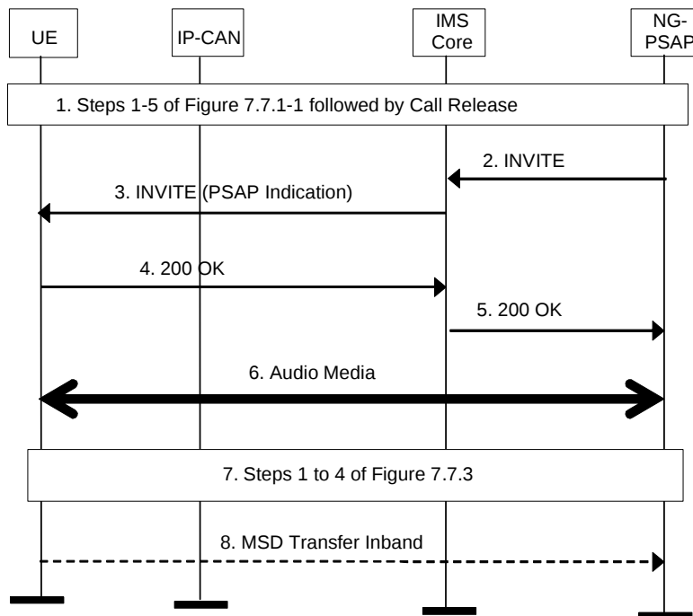
Figure 7.7.8-1: Callback from an NG capable PSAP with transfer of updated MSD
