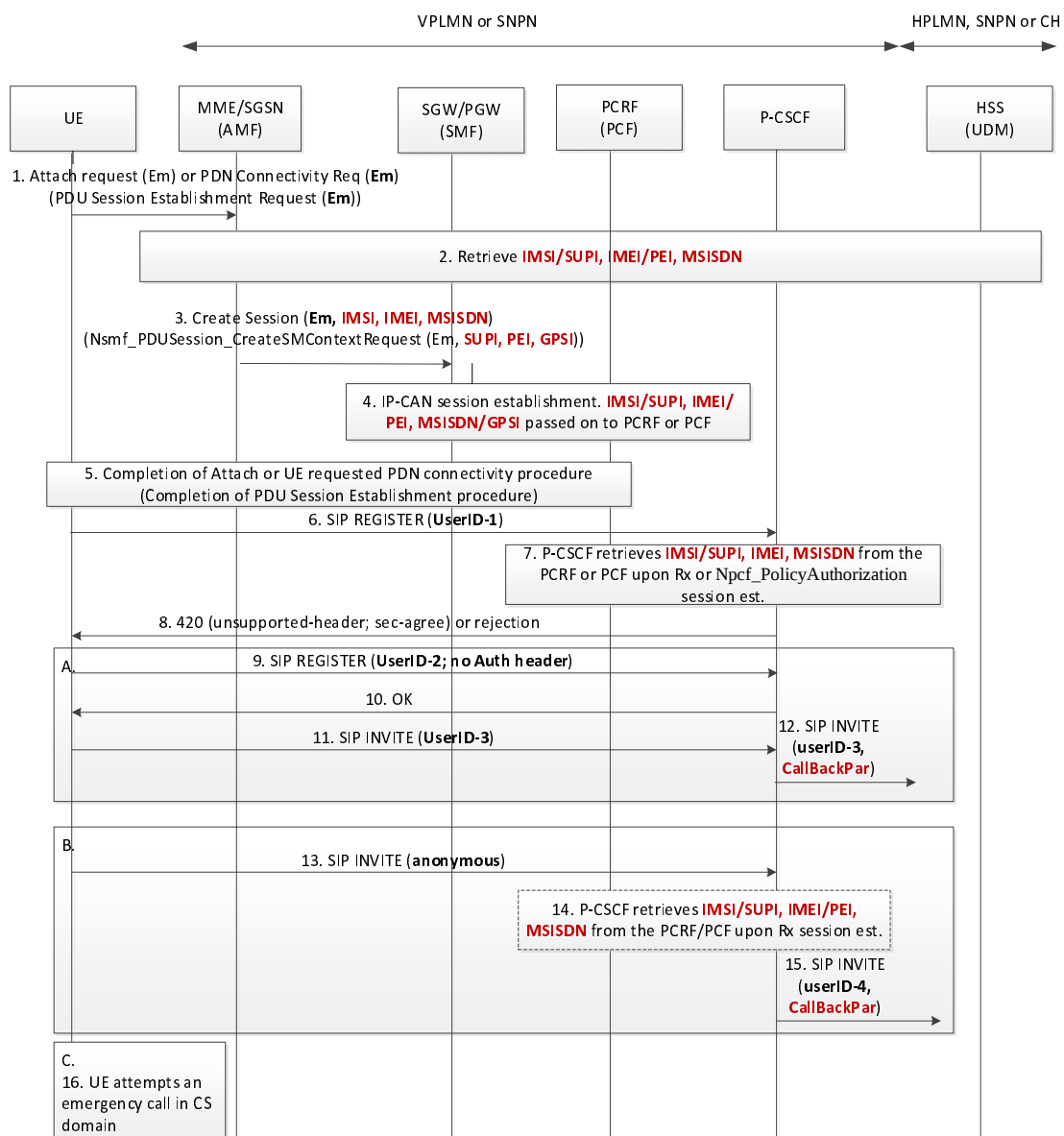
Figure K.3-1: IMS Emergency Session Establishment in deployments without IMS roaming interface between VPLMN and HPLMN
