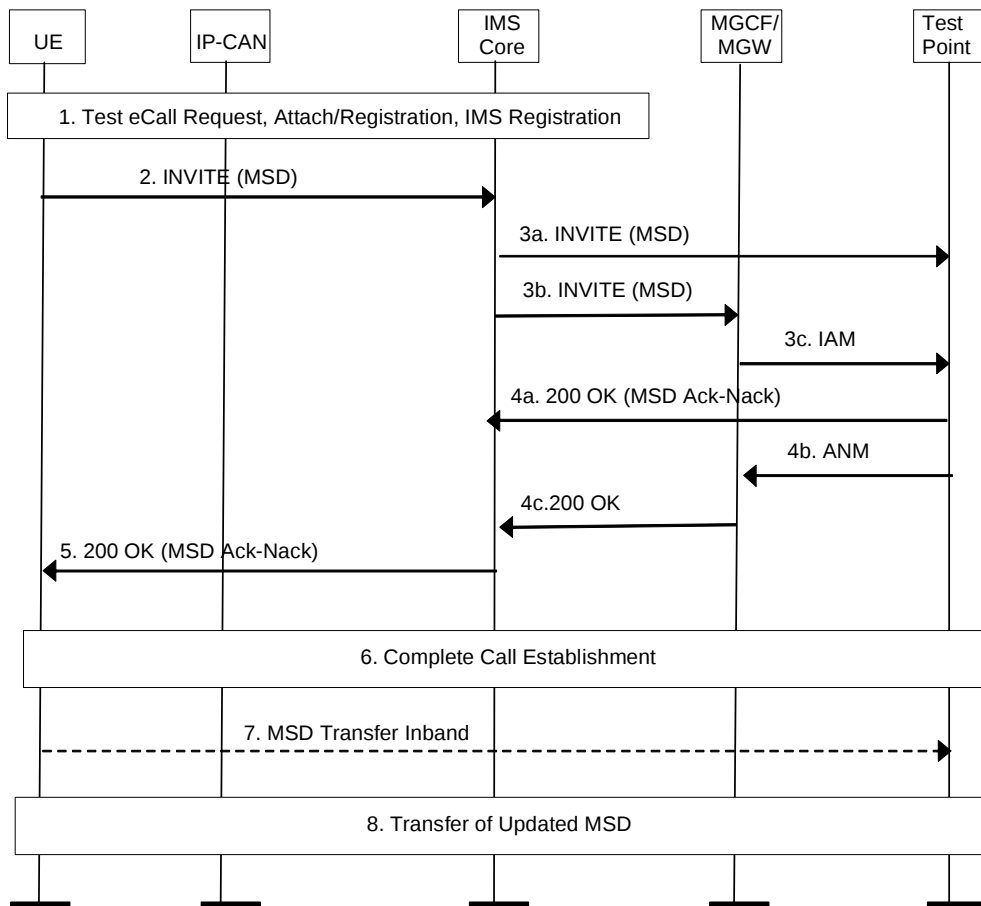
Figure N.2-1: Test eCall over IMS Session Establishment to a Test Point
