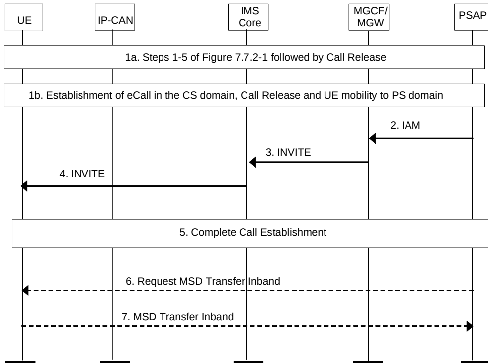
Figure 7.7.9-1: Callback from a PSAP in the CS domain with transfer of updated MSD
