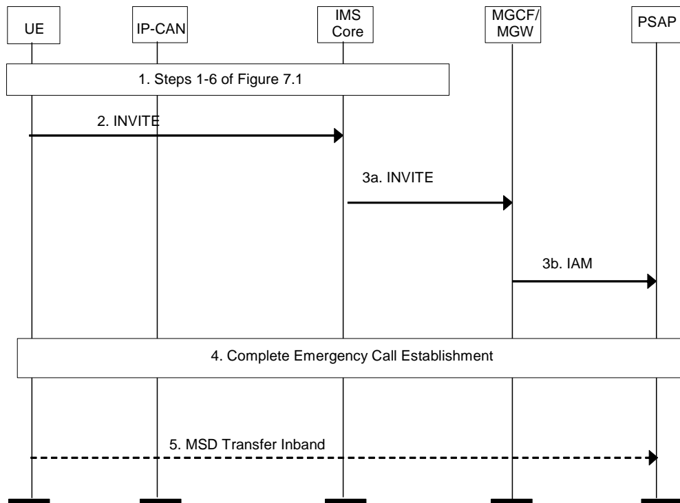
Figure 7.7.2-1: eCall Scenario with PSAP not supporting NG-eCall
