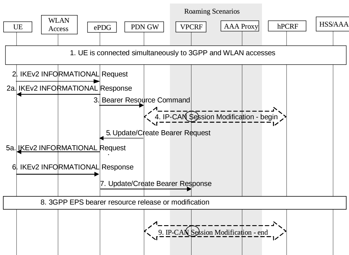
Figure 6.3.3-1: IP flow mobility within a PDN connection initiated over WLAN access
