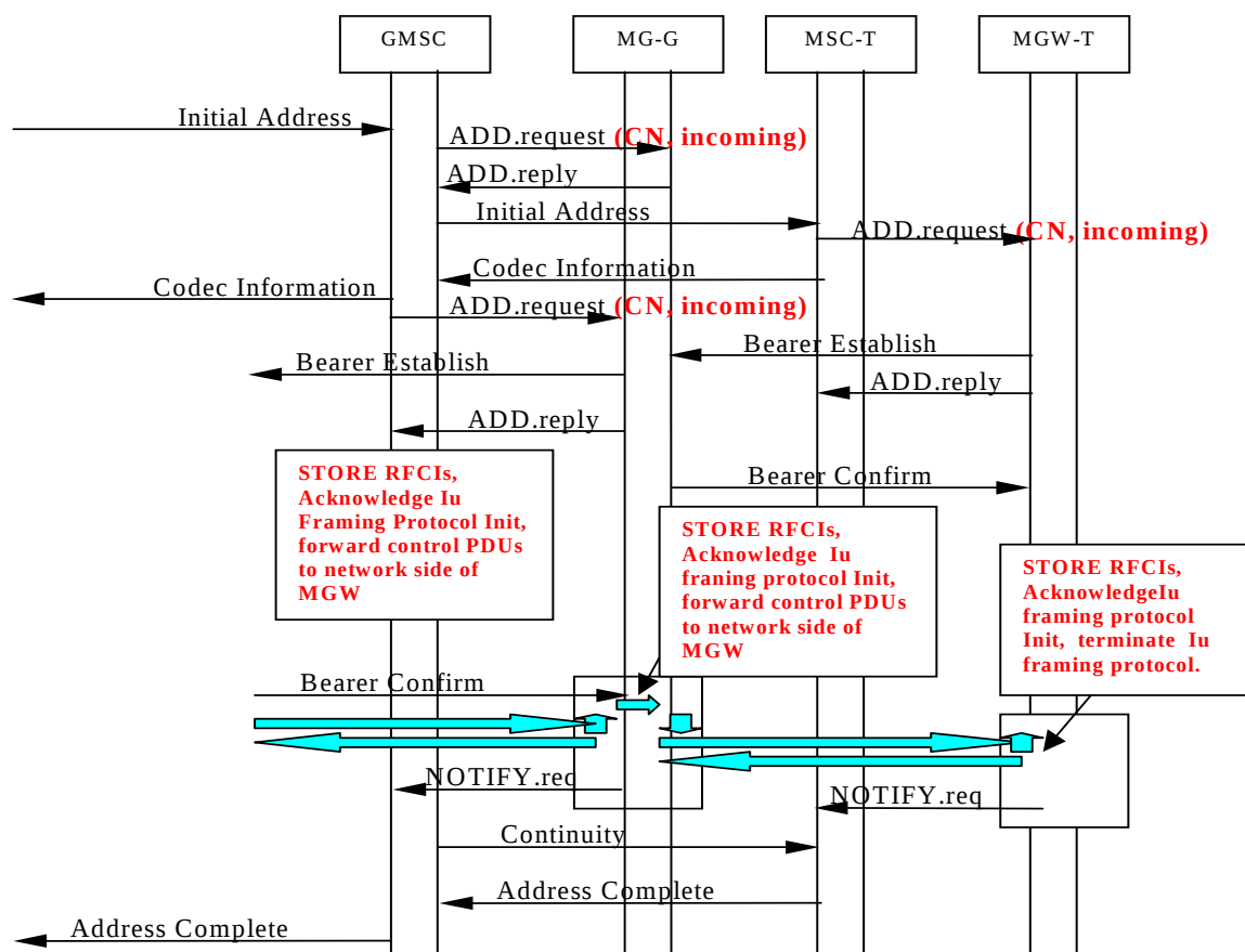
Figure 5.4.1/2: lu Framing Protocol Establishment, backward bearer.
