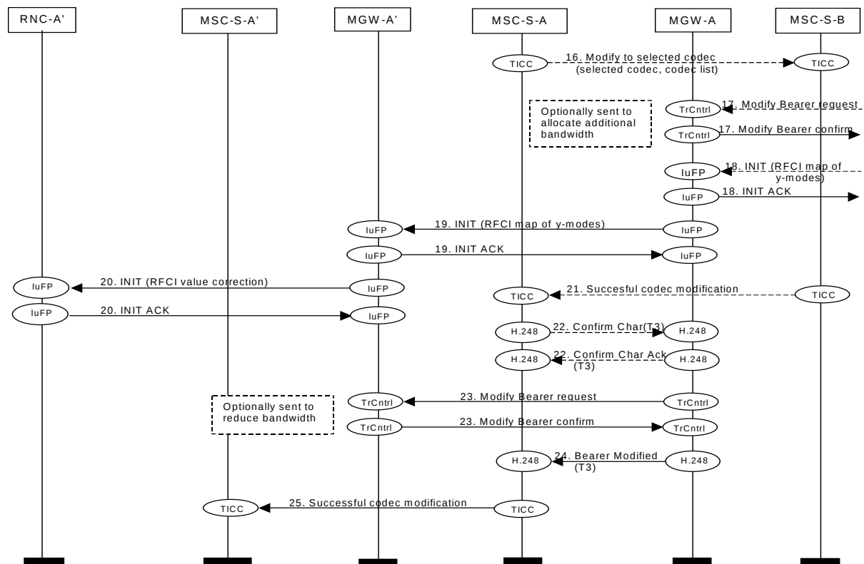
Figure 6.2/10: Mid-call codec negotiation after Inter-MSR SRNS Relocation. Flow Chart Part 2.
