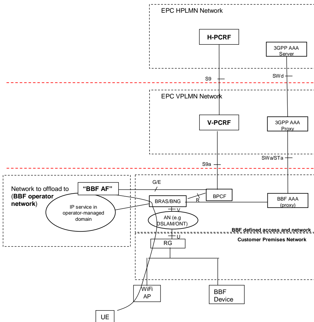
Figure 4.2.4-4: NSWO for 3GPP over BBF domain supporting the AF – roaming scenario
