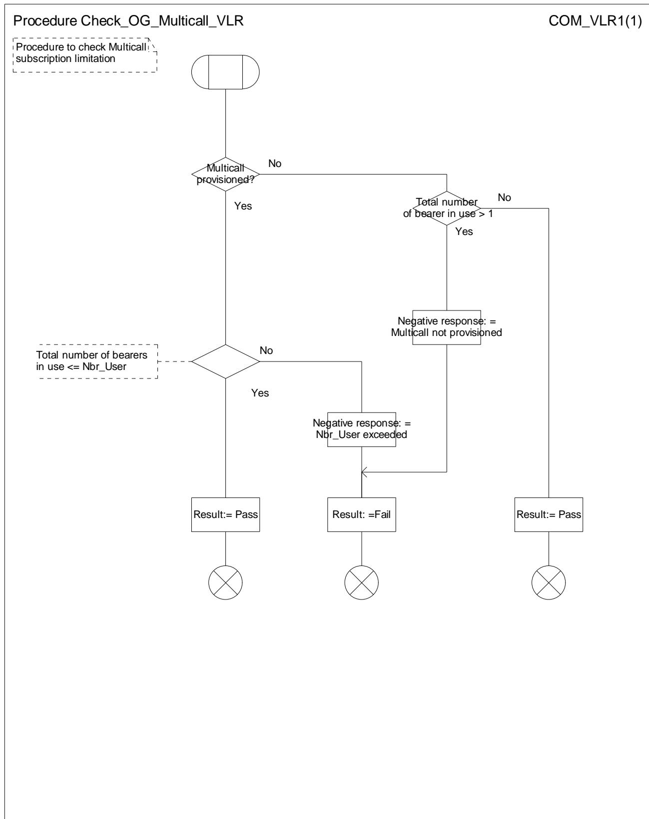
Figure 9: Procedure Check_OG_Multicall_VLR
