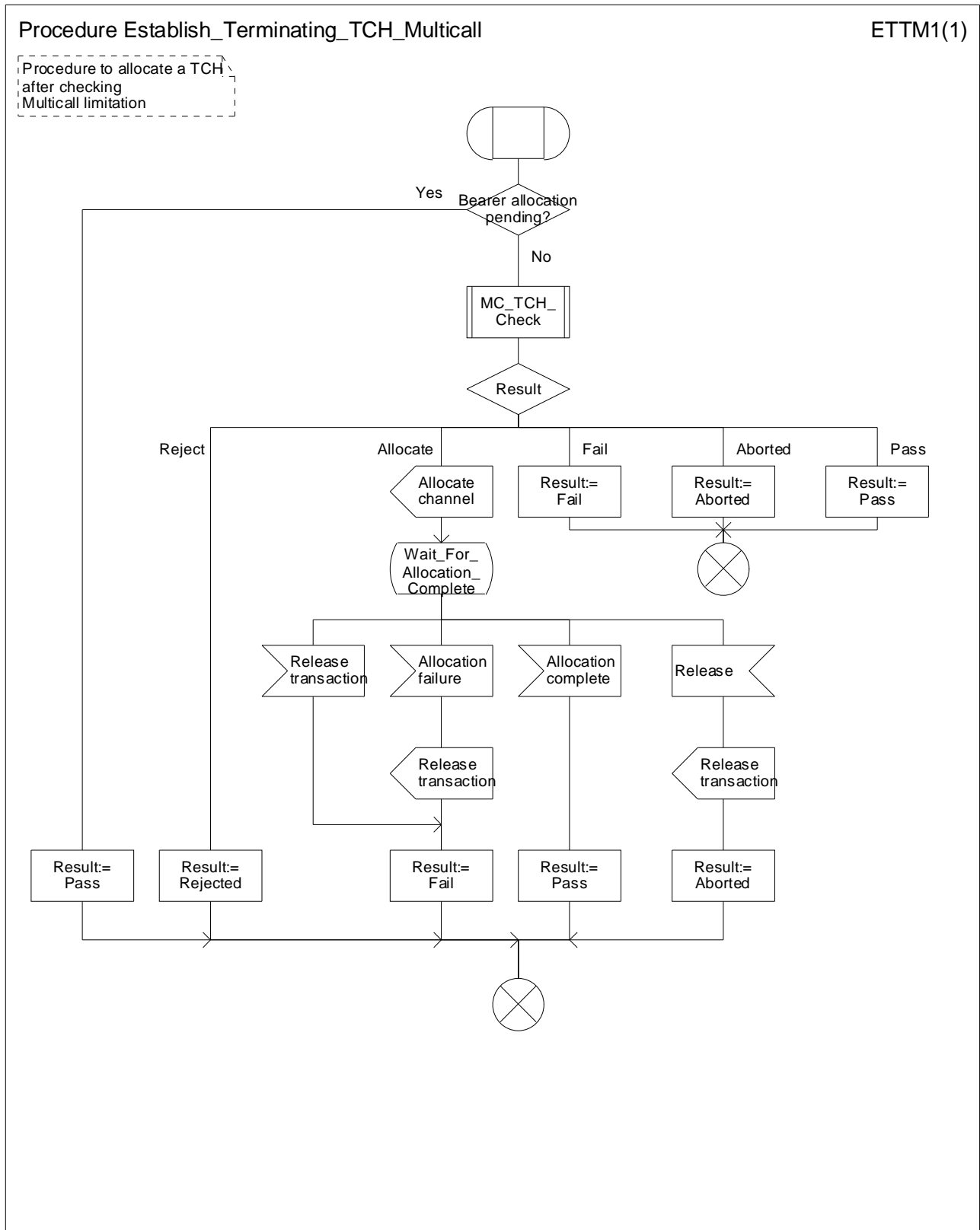
Figure 11: Procedure Establish_Terminating_TCH_Multicall
