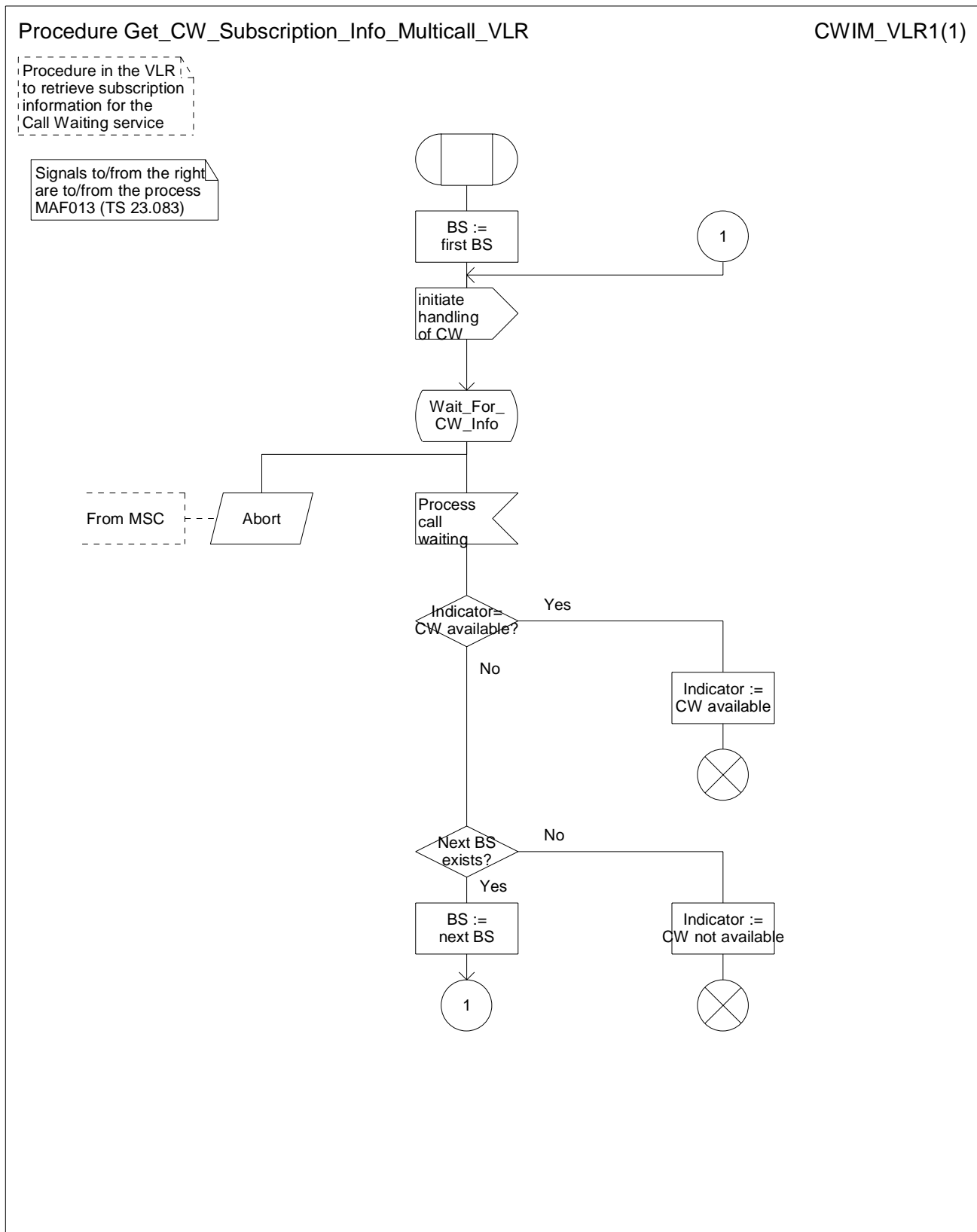
Figure 13: Procedure Get_CW_Subscription_Info_Multicall_VLR
