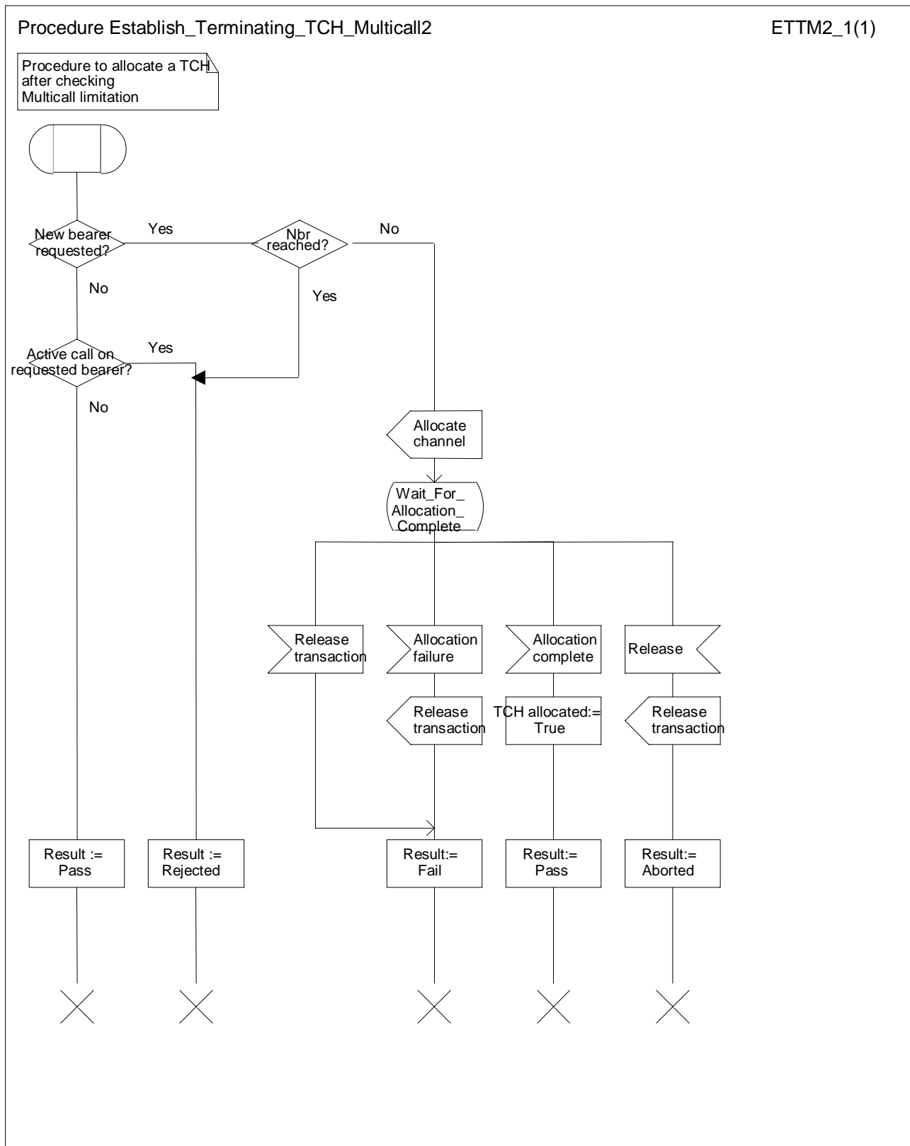
Figure 12: Procedure Establish_Terminating_TCH_Multicall2
