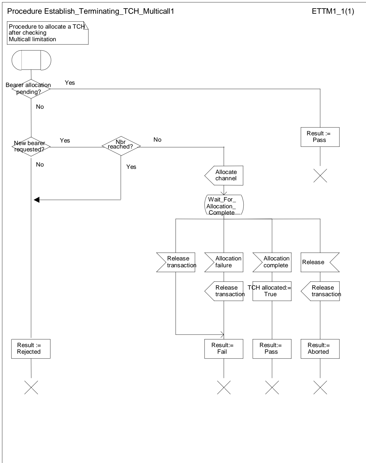
Figure 11: Procedure Establish_Terminating_TCH_Multicall1
