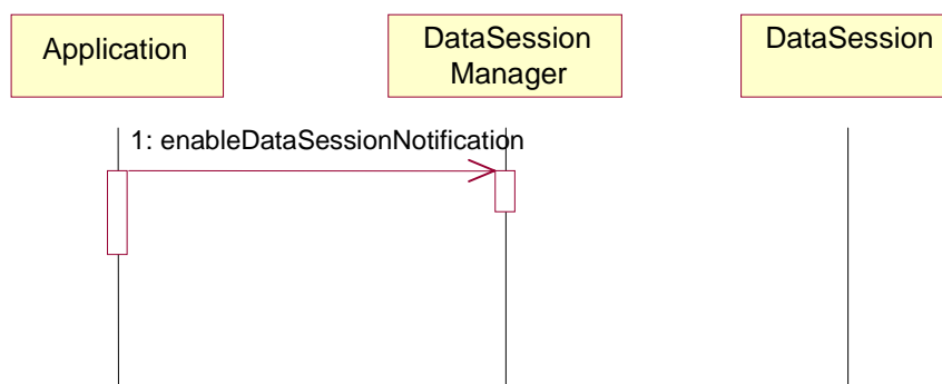
Figure 12: Enable Data Session Notification
