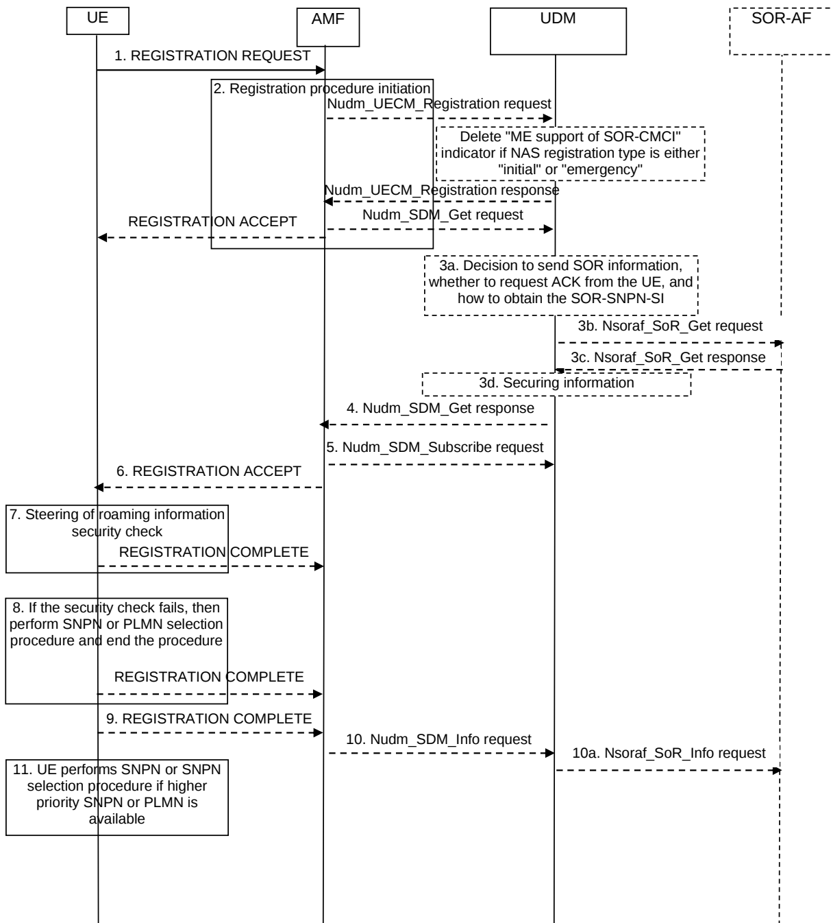
Figure C.5.1: Procedure for providing SOR-SNP-SI and SOR-SNP-SI-LS (if any) during registration
