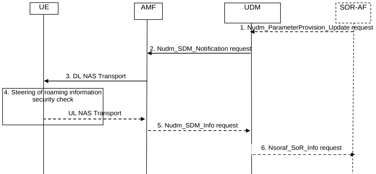
Figure C.6.1: Procedure for providing SOR-SNP-SI (if any) and SOR-SNP-SI-LS (if any) after registration
