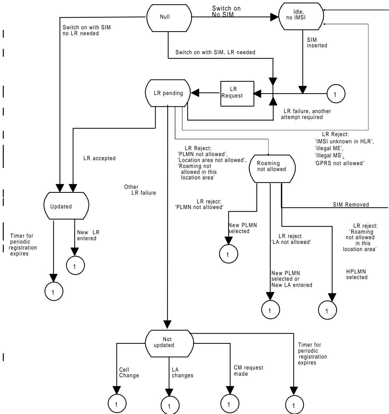
Figure 3: Location Registration Task State diagram
