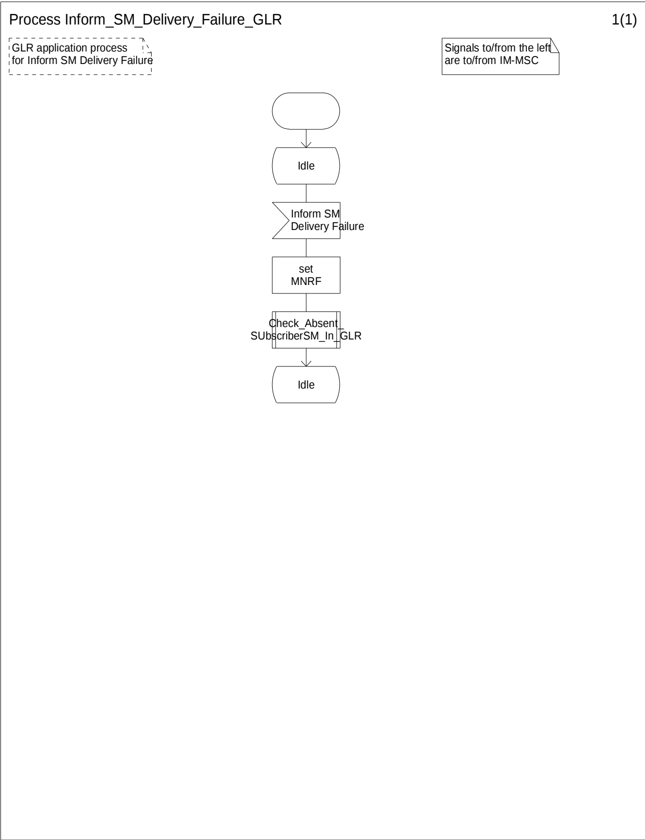
Figure 7.7/7: Process Inform_SM_Delivery_Failure_GLR
