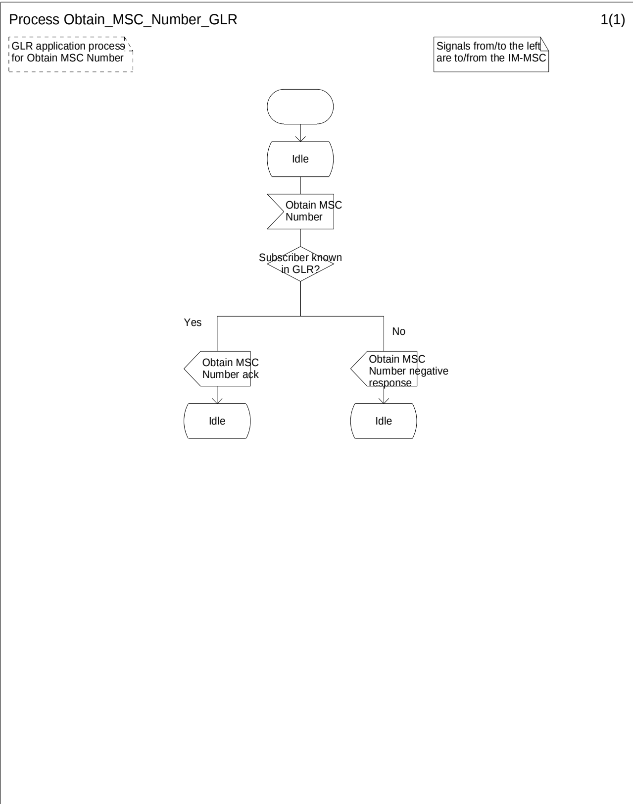
Figure 7.7/6: Process Obtain_MSC_Number_GLR
