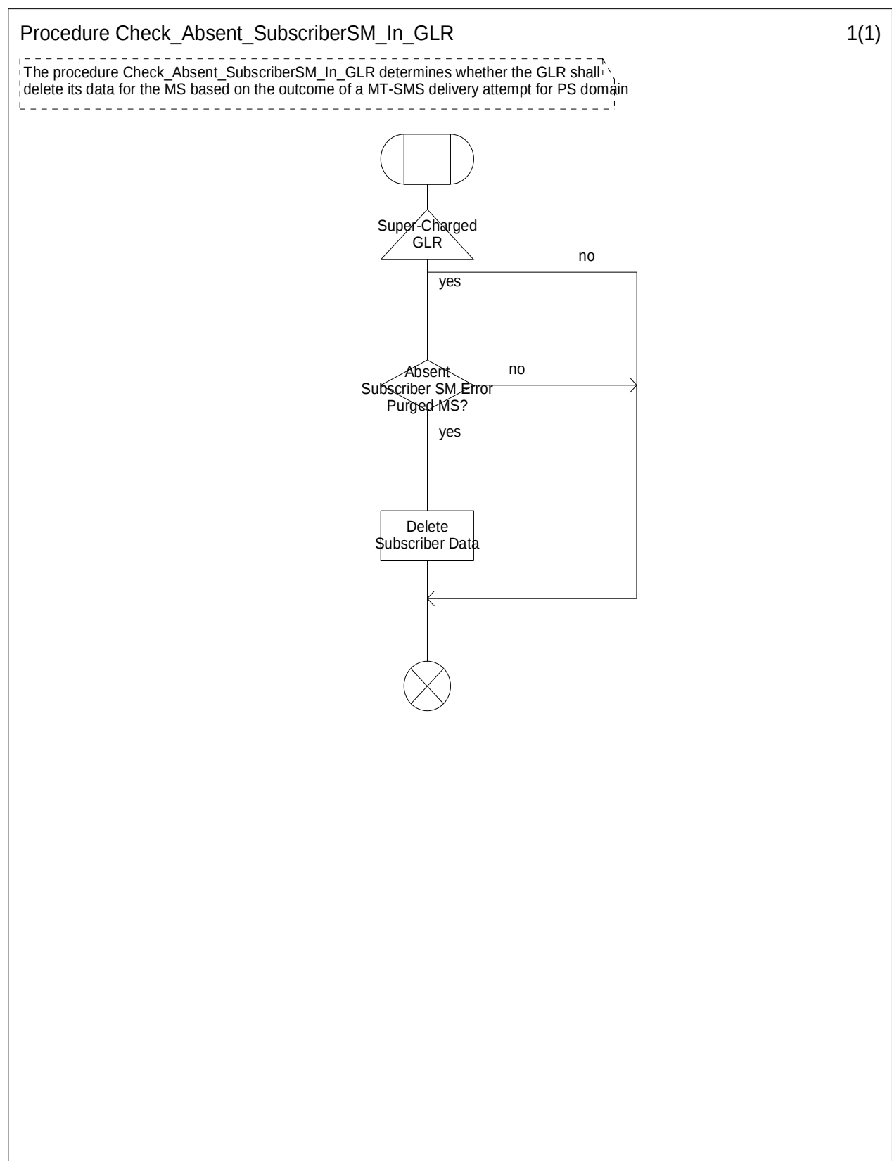
Figure 7.7/8: Procedure Check_Absent_SubscriberSM_In_GLR
