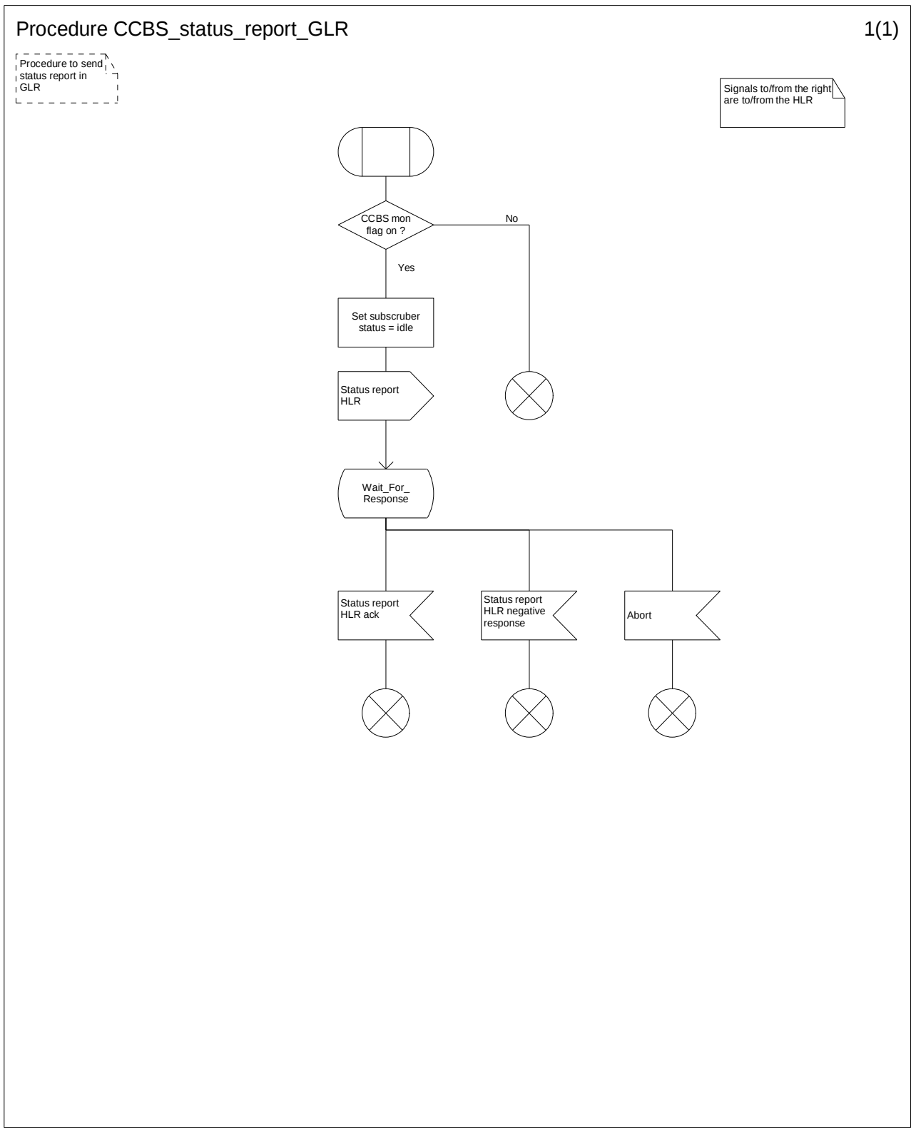
Figure 7.10/6: Procedure CCBS_Status_Report_GLR
