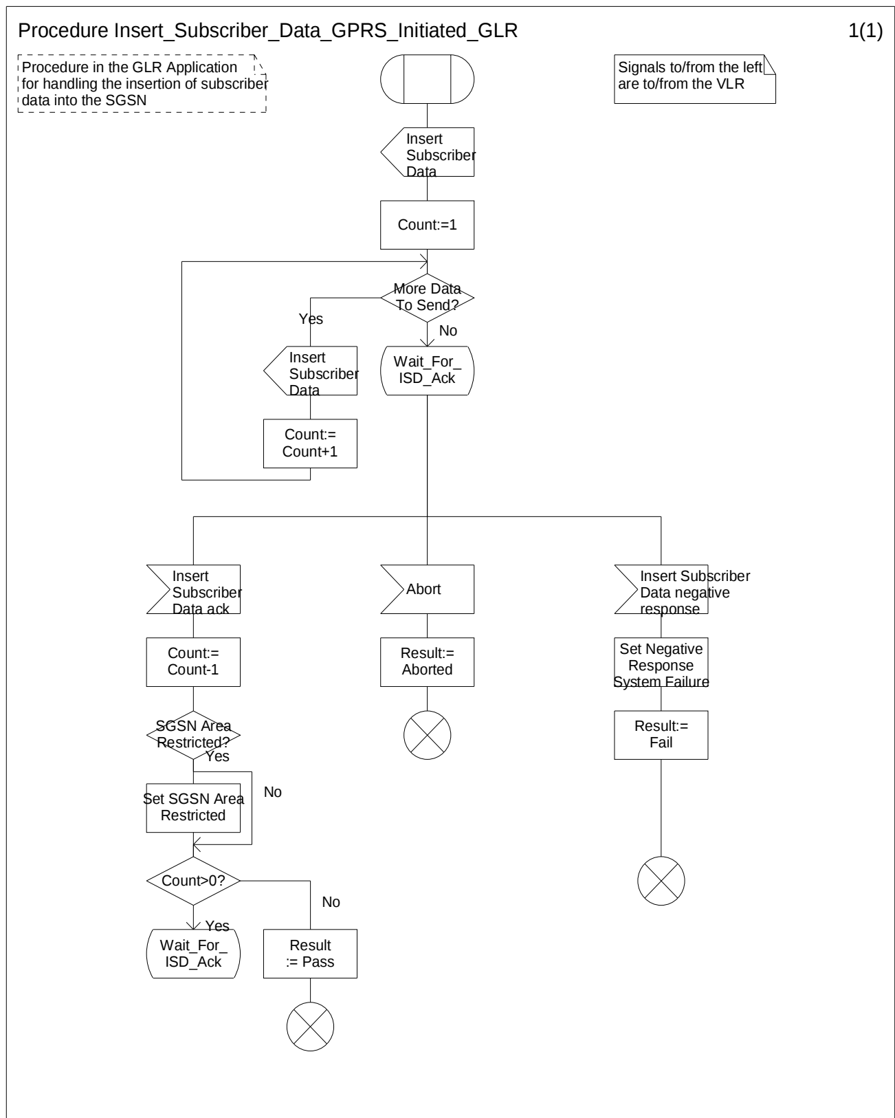
Figure 7.3/7: Procedure Insert_Subscriber_Data_GPRS_Initiated_GLR
