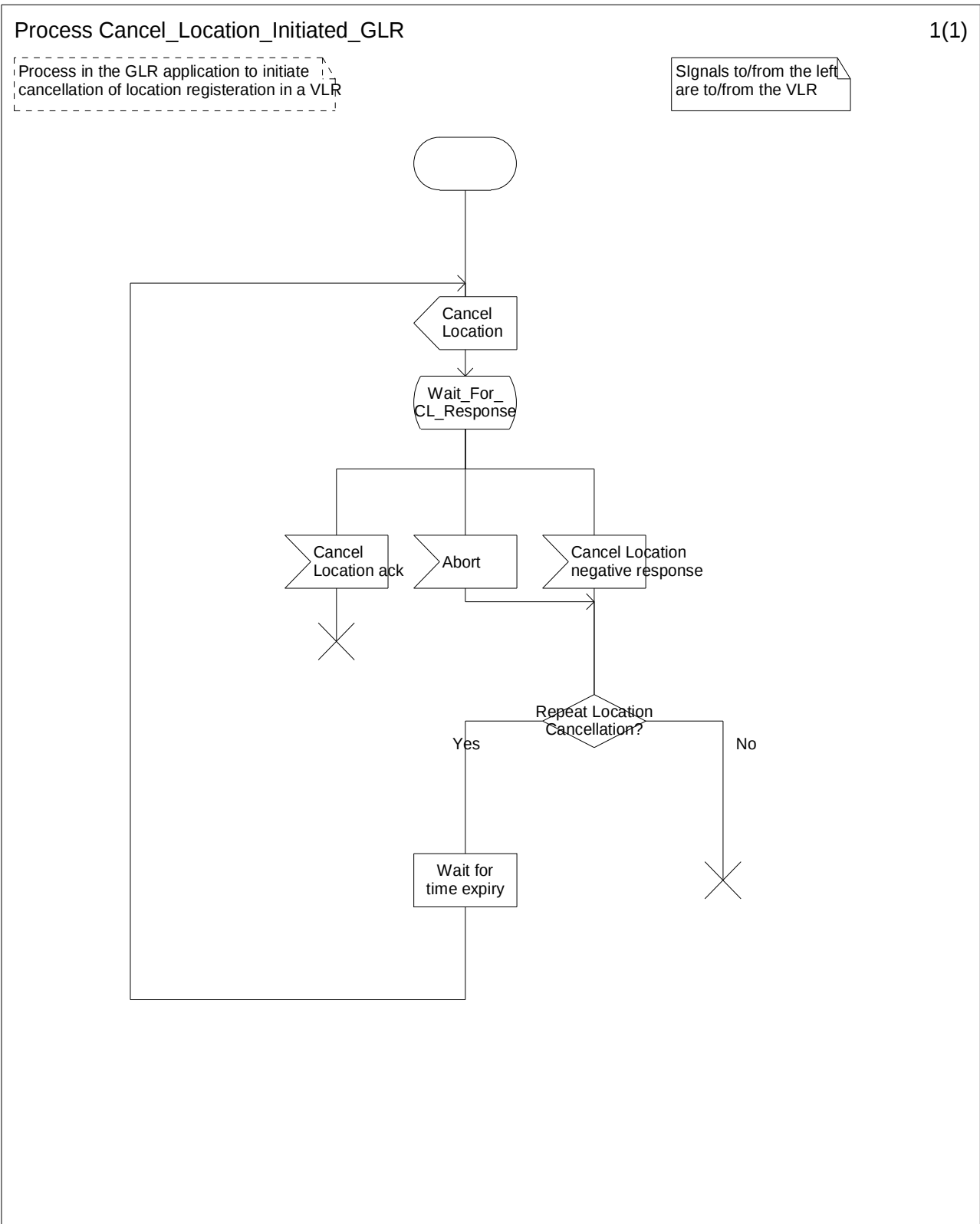
Figure7.2/9: Process Cancel_Location_Initiated_GLR
