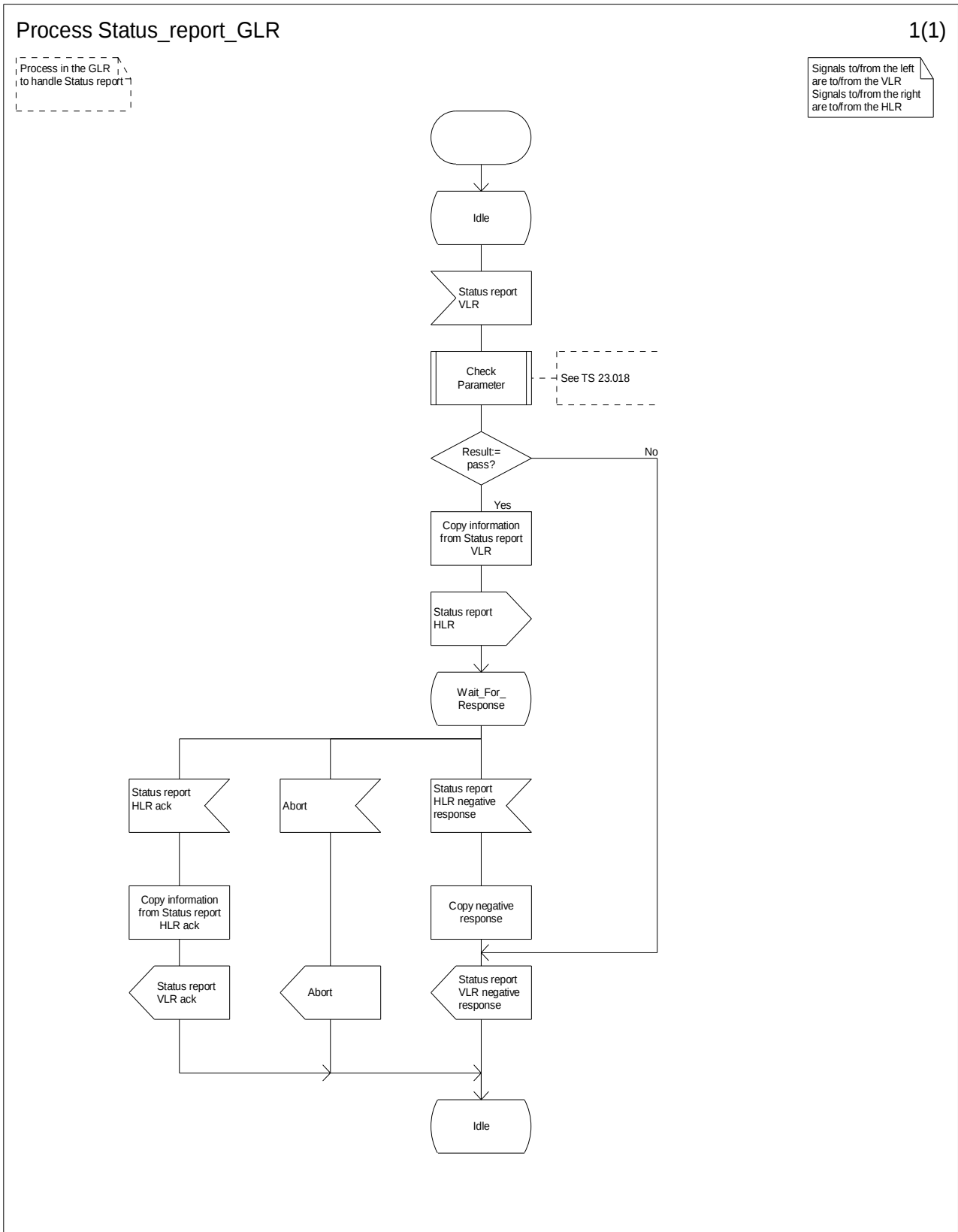
Figure 7.10/4: Process Status_report_GLR
