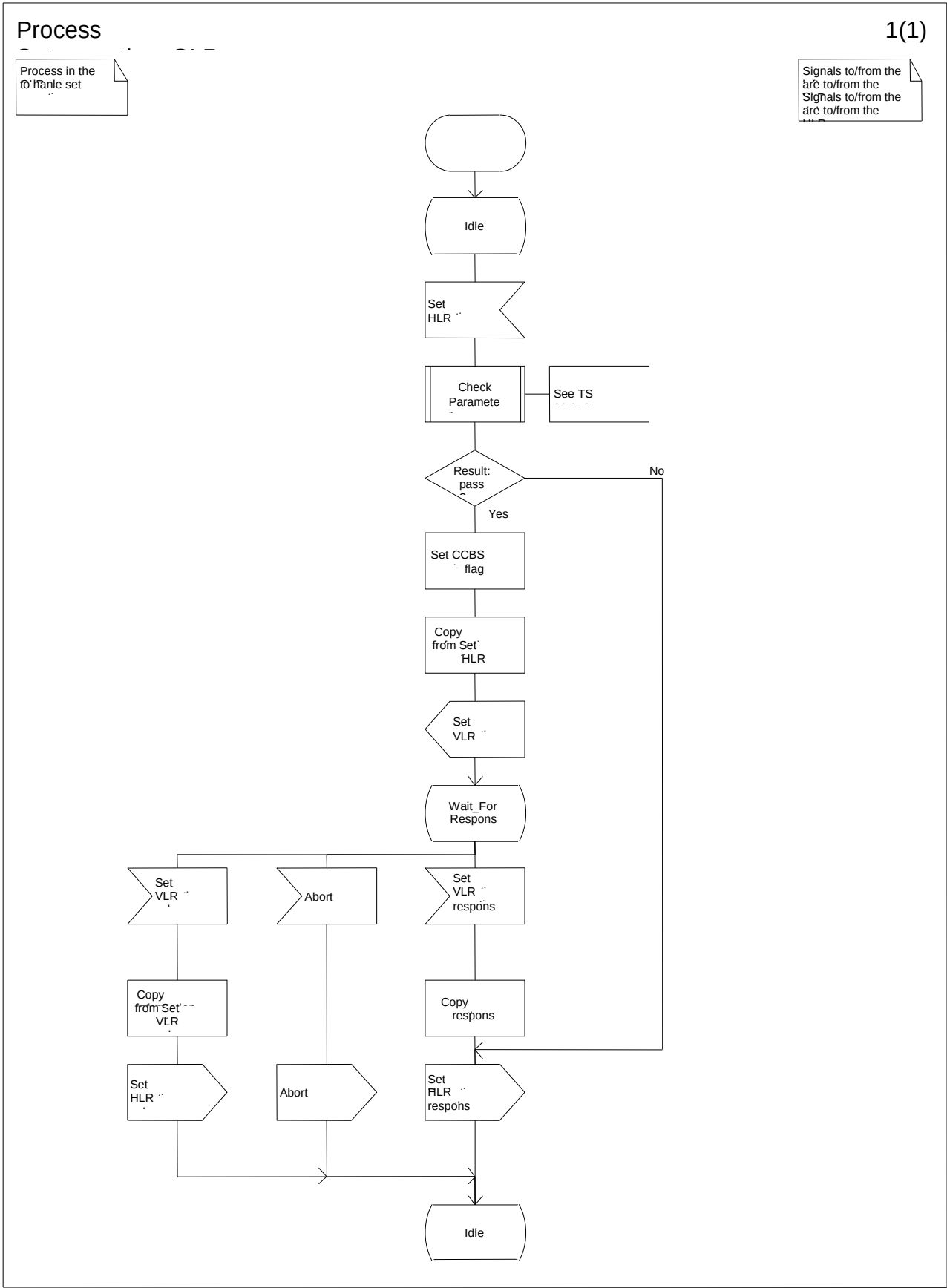
Figure 7.10/3: Process Set_reporting_GLR
