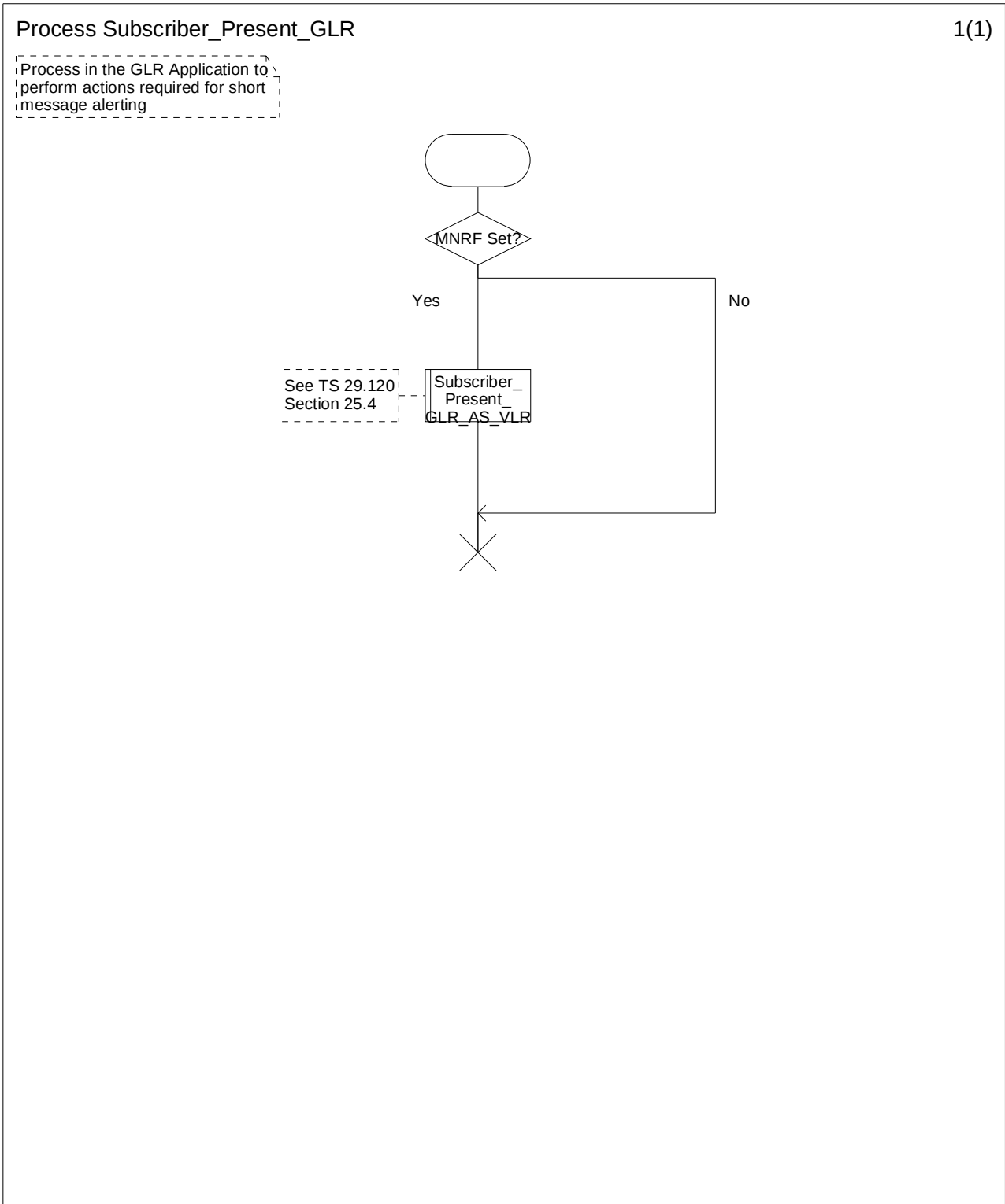
Figure7.2/4: Process Subscriber_Present_GLR
