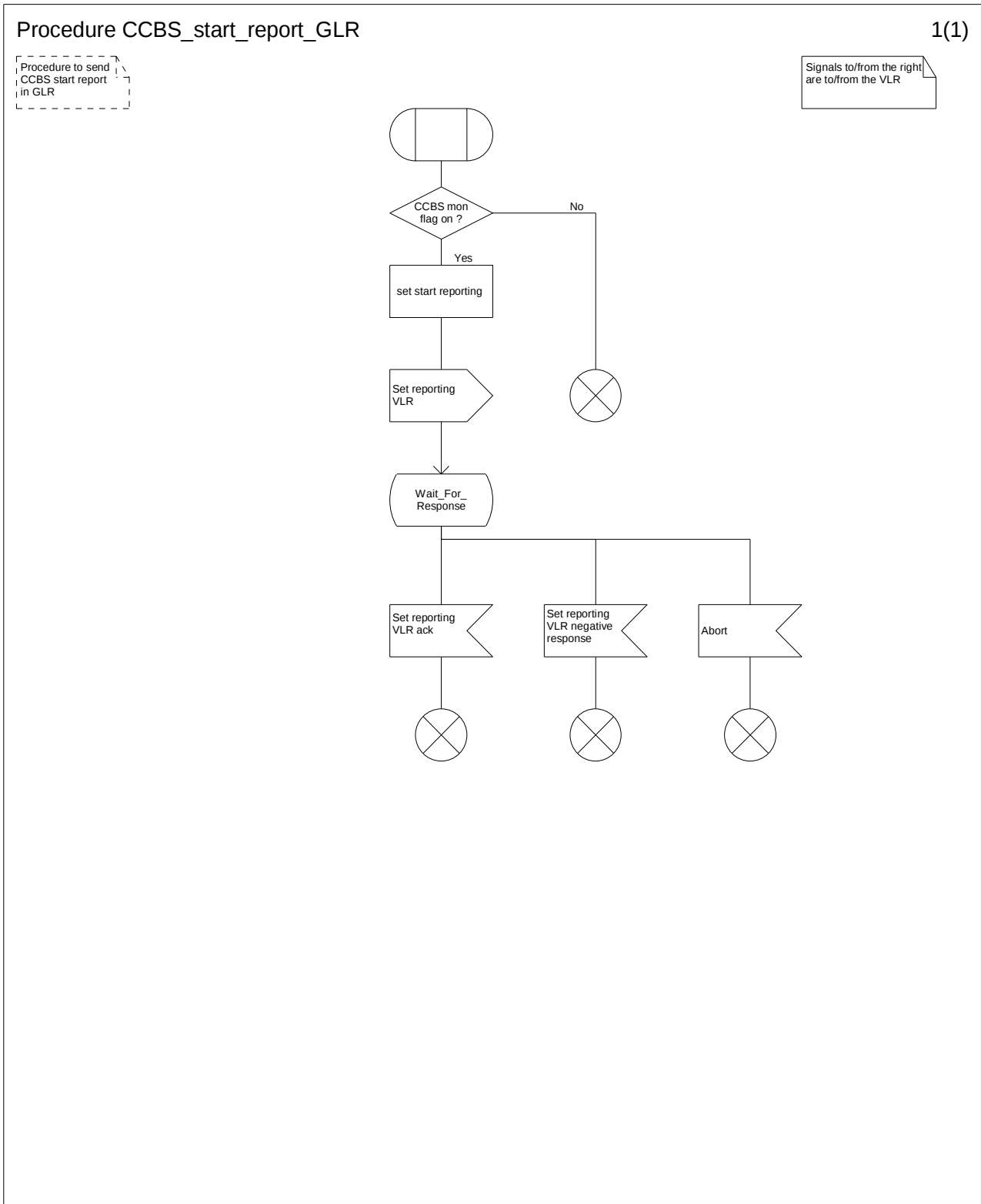
Figure 7.10/7: Procedure CCBS_Start_Report_GLR
