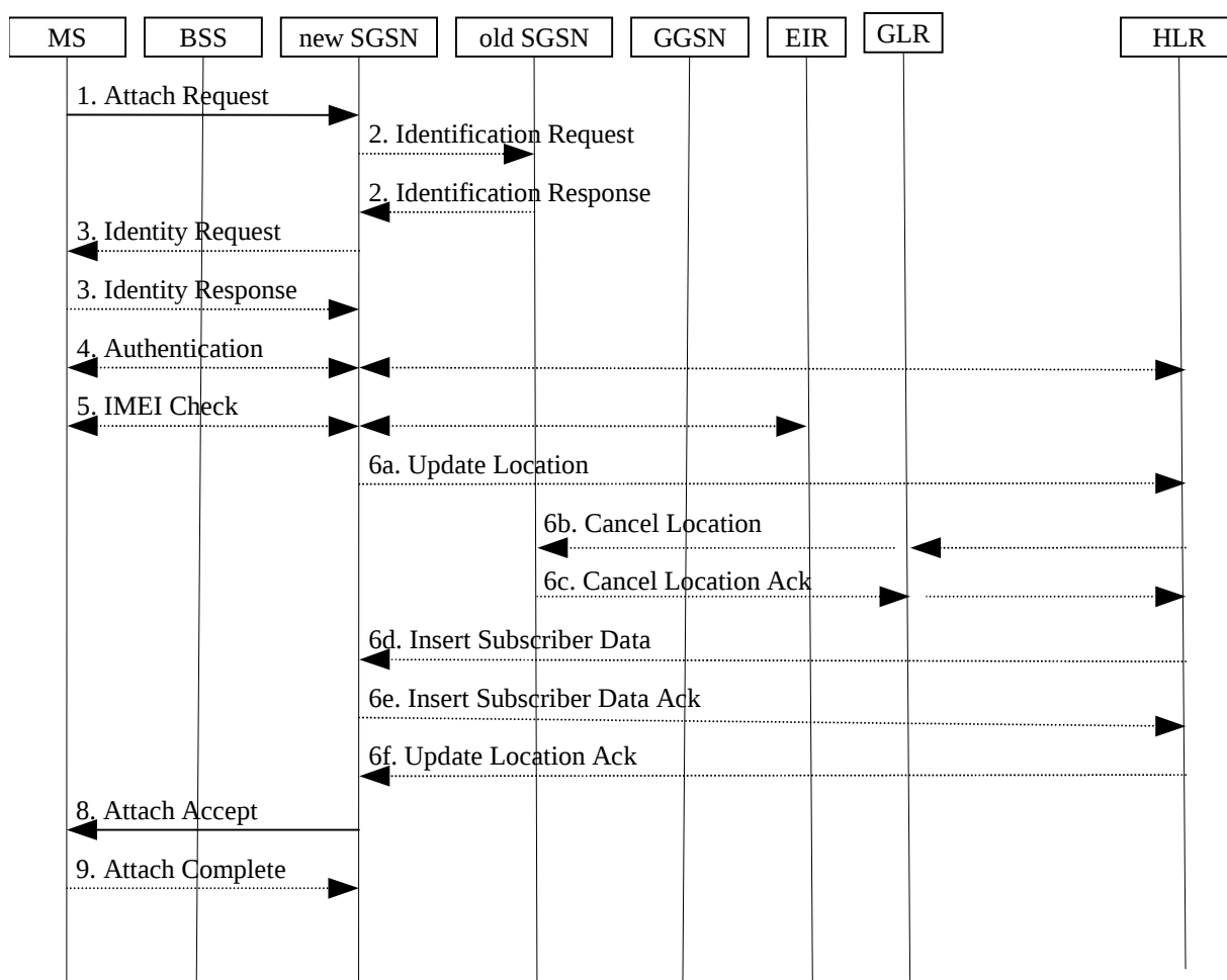
Figure 7.3/4: GPRS Attach Procedure involving GLR (new SGSN interfaces the HLR directly. Old SGSN is under the GLR)
