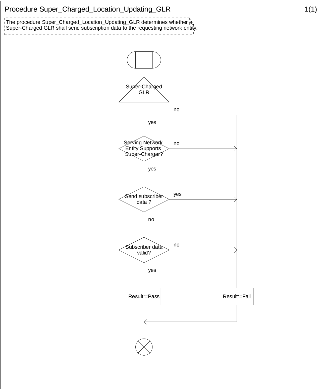
Figure 7.13/5: Procedure Super_Charged_Location_Updating_GLR
