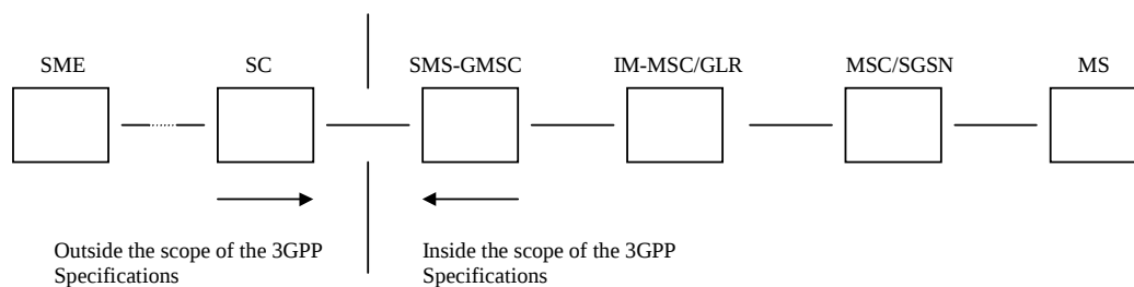
Figure 7.7/1: Entities involved in the provision of SM MT with GLR
