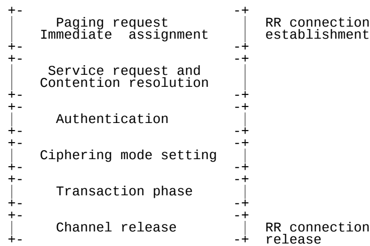
Figure 7.1/3GPP TS 23.108: Components of structured procedures
