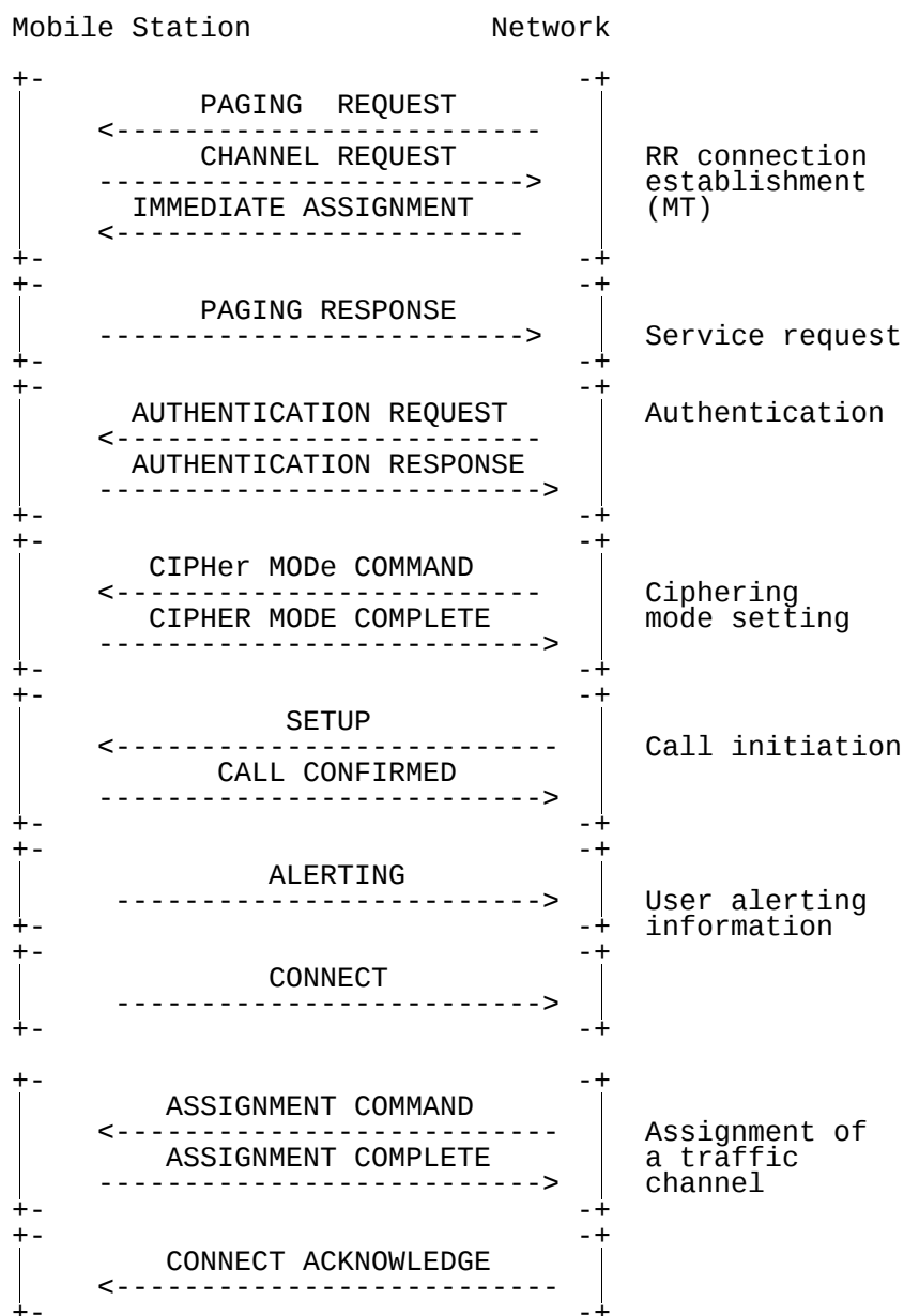
Figure 7.11b/3GPP TS 23.108: Mobile terminating: call establishment with OACSU (late assignment)
