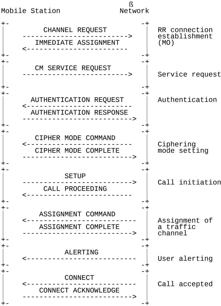
Figure 7.10a/3GPP TS 23.108: Mobile originating call establishment without OACSU (early assignment)
