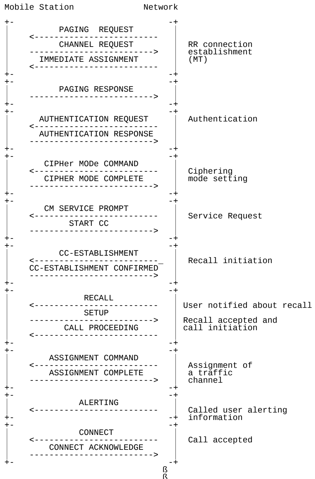
Figure 7.20/3GPP TS 23.108: Network initiated mobile originating call establishment with assignment before B party alerting
