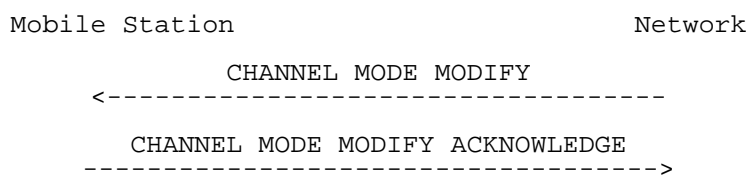
Figure 7.7/3GPP TS 23.108: Channel mode change
