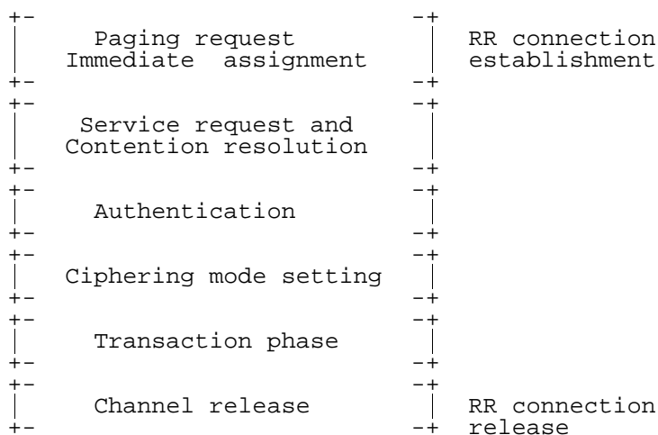
Figure 7.1/3GPP TS 23.108: Components of structured procedures
