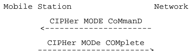
Figure 7.6/3GPP TS 23.108: Ciphering mode setting
