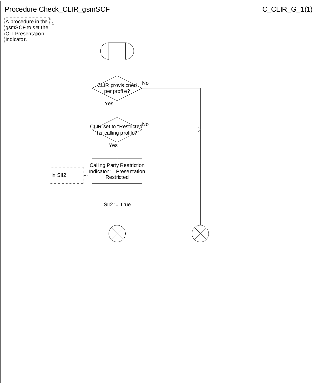
Figure 9: Procedure Check_CLIR_gsmSCF
