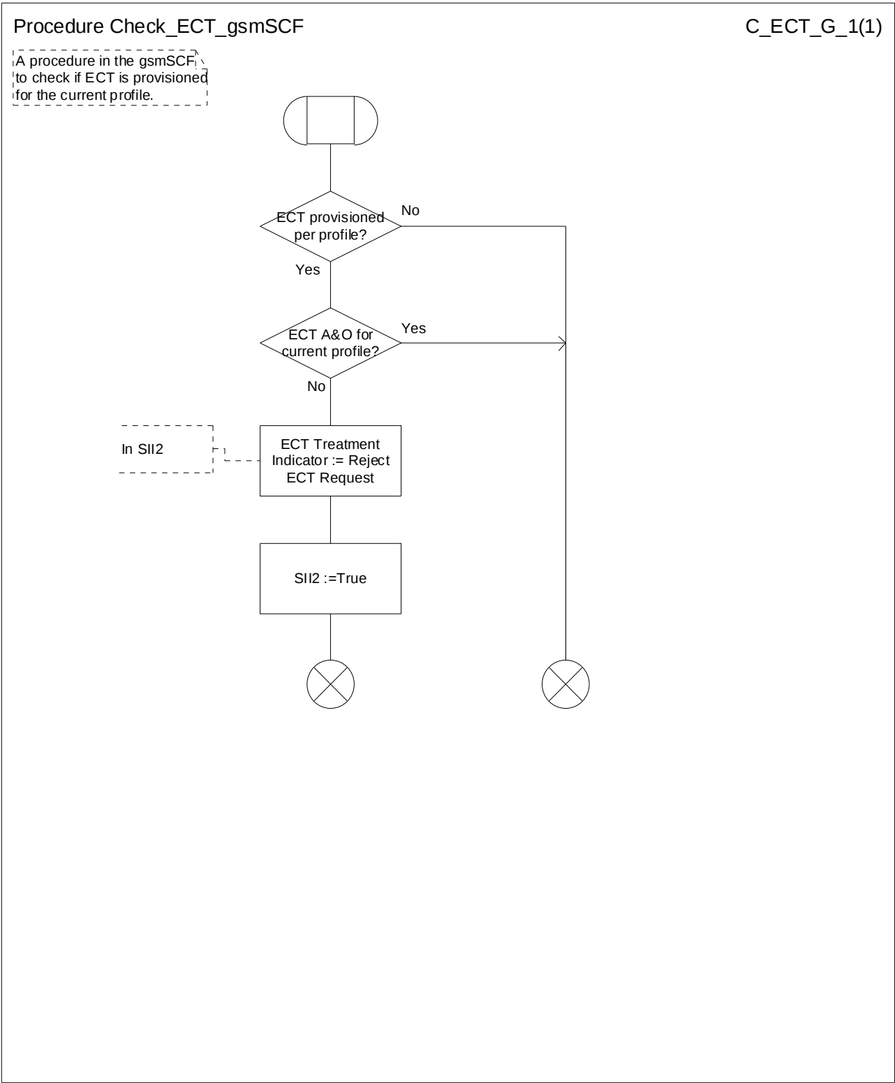
Figure 26: Procedure Check_ECT_gsmSCF
