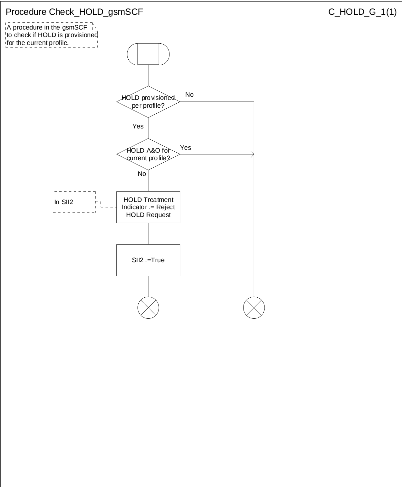
Figure 18: Procedure Check_HOLD_gsmSCF
