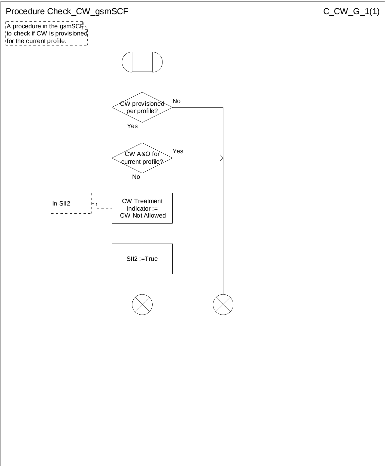
Figure 17: Procedure Check_CW_gsmSCF
