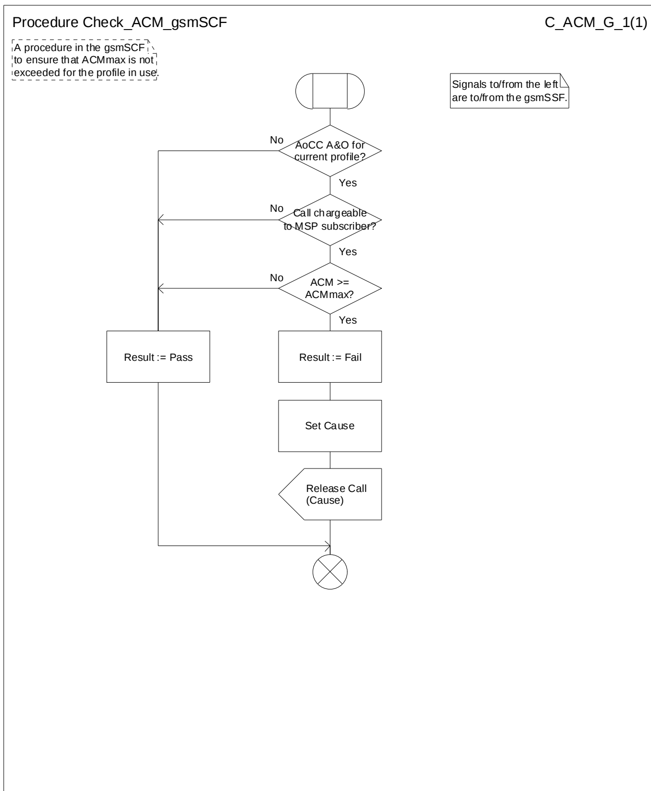
Figure 20: Procedure Check_ACM_gsmSCF
