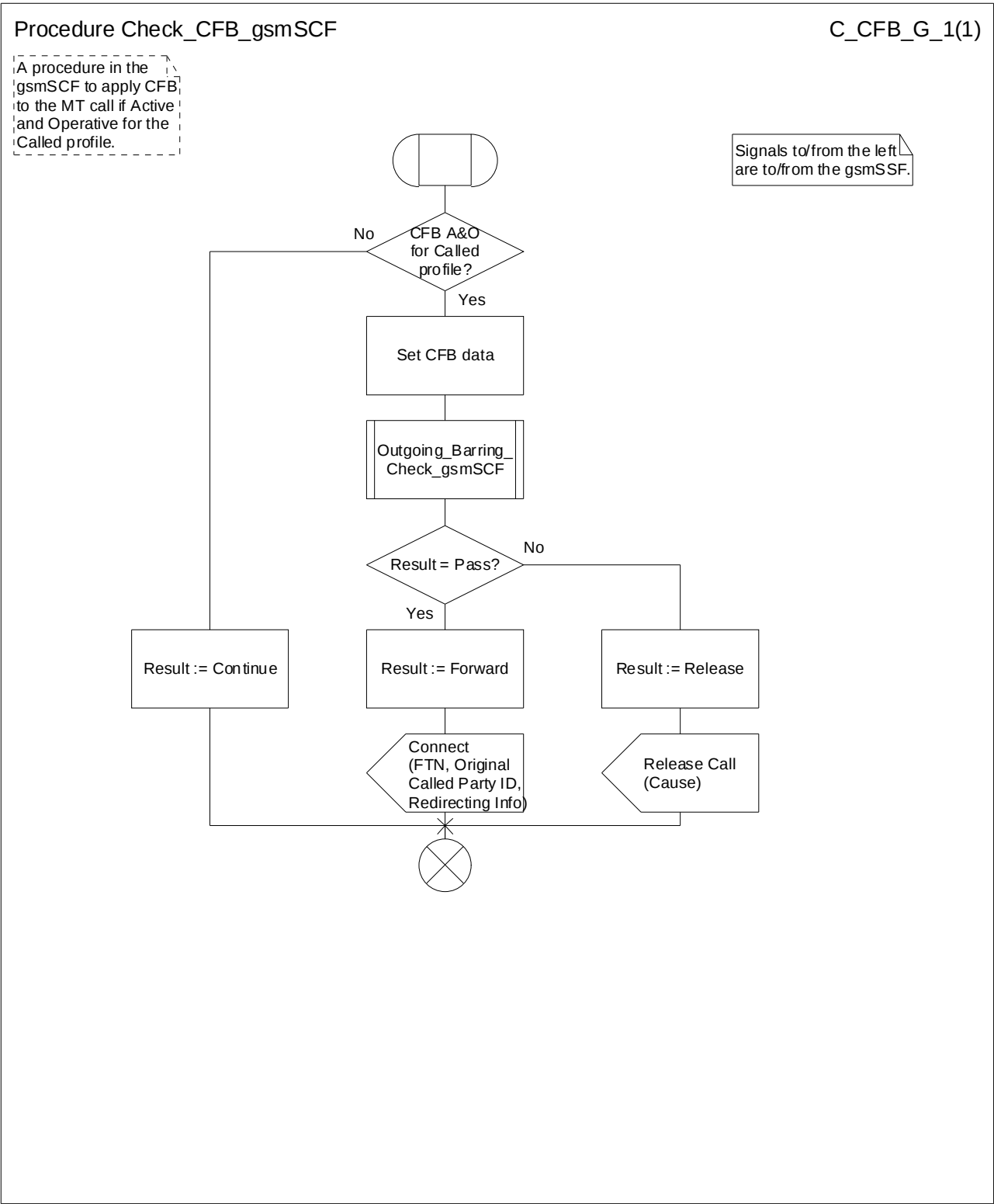
Figure 15: Procedure Check_CFB_gsmSCF
