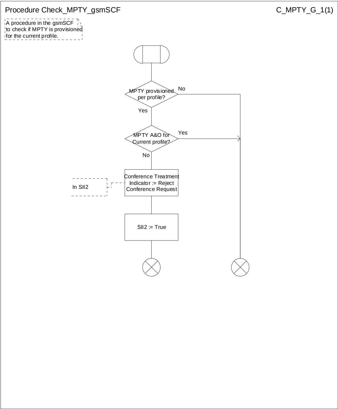
Figure 19: Procedure Check_MPTY_gsmSCF
