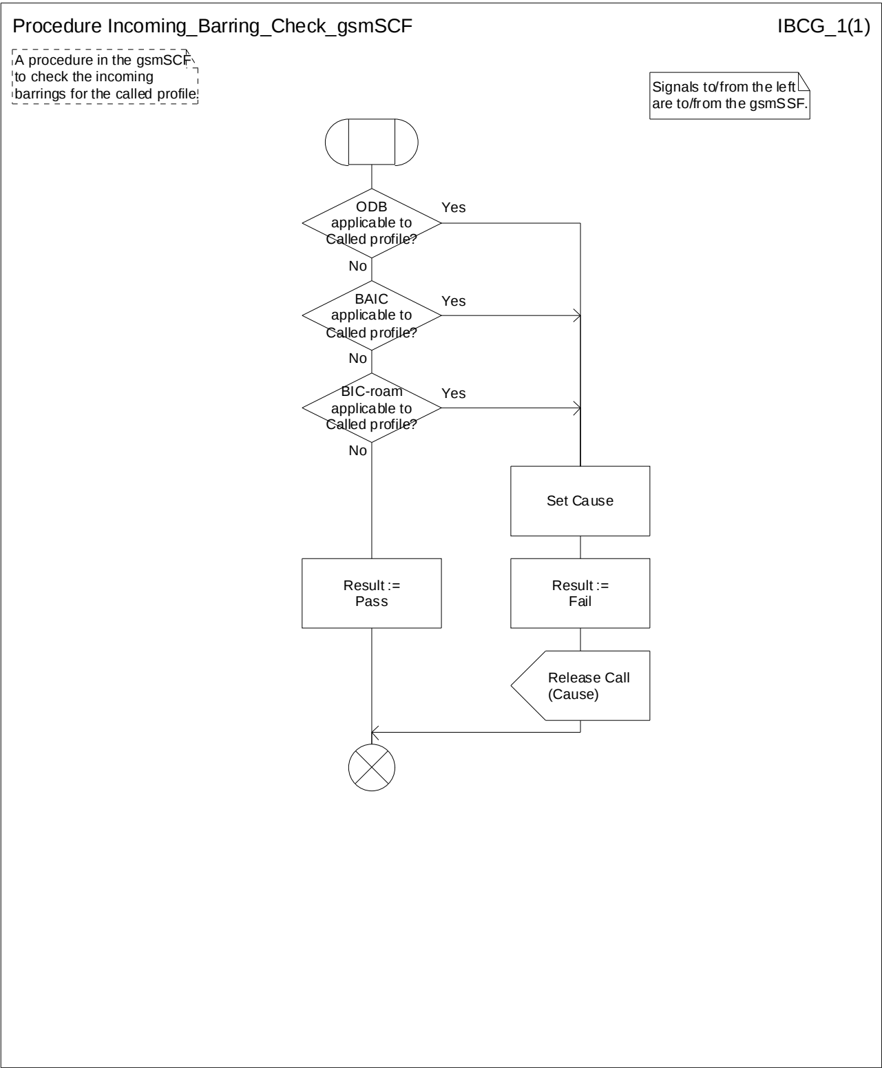
Figure 25: Procedure Incoming_Barring_Check_gsmSCF
