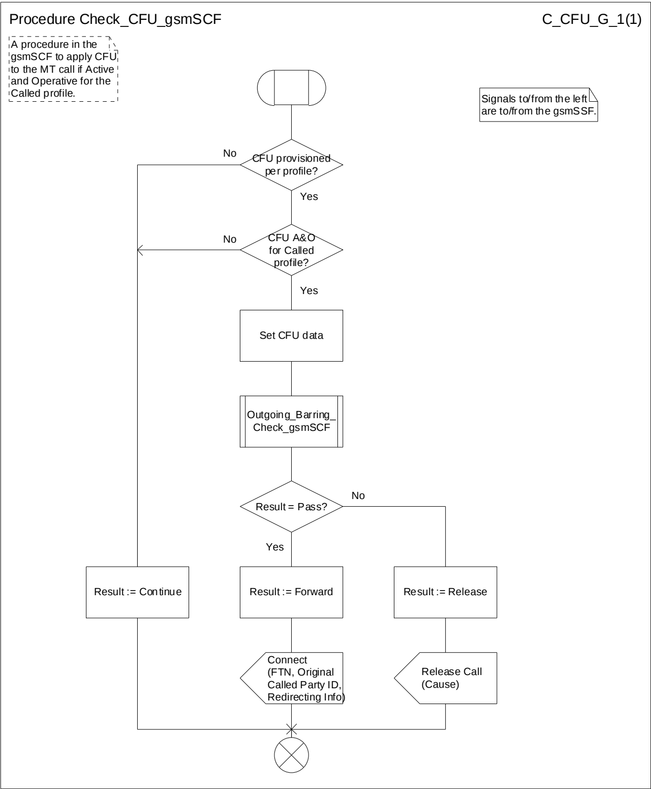
Figure 11: Procedure Check_CFU_gsmSCF
