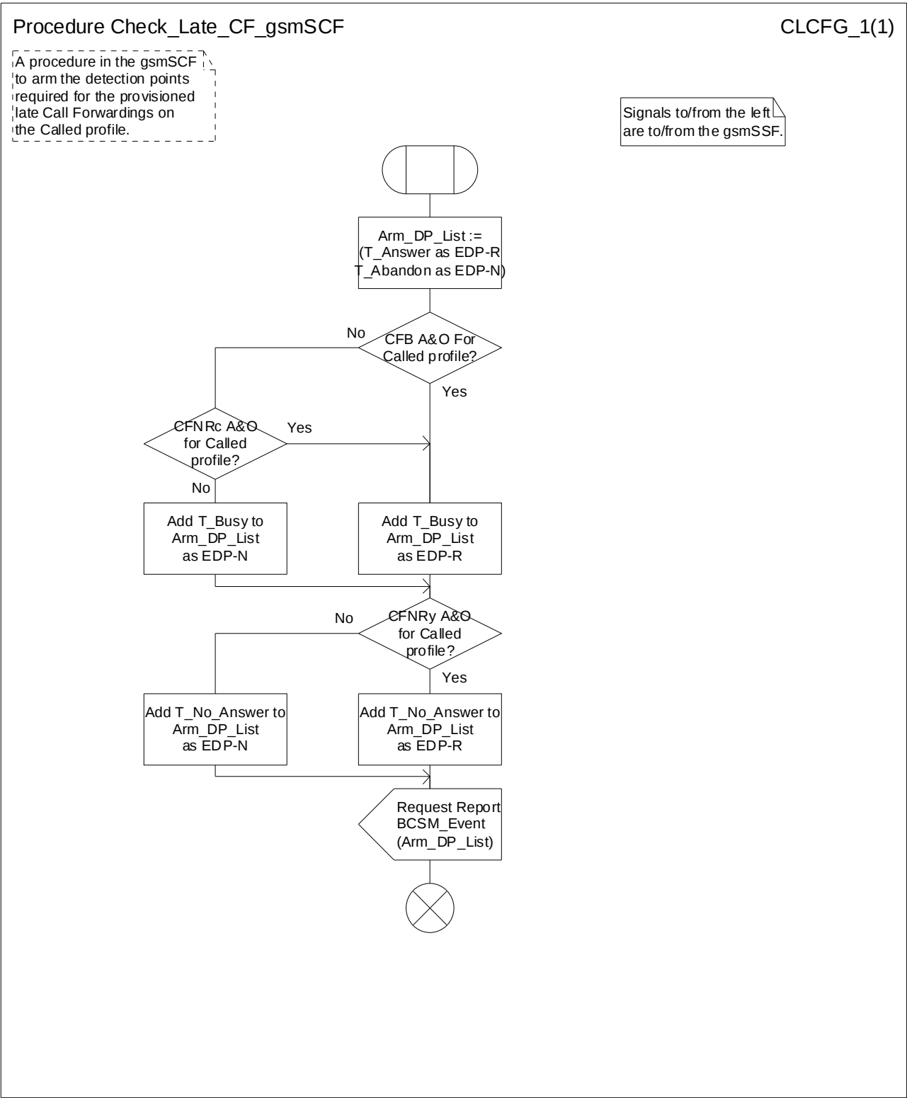
Figure 13: Procedure Check_Late_CF_gsmSCF
