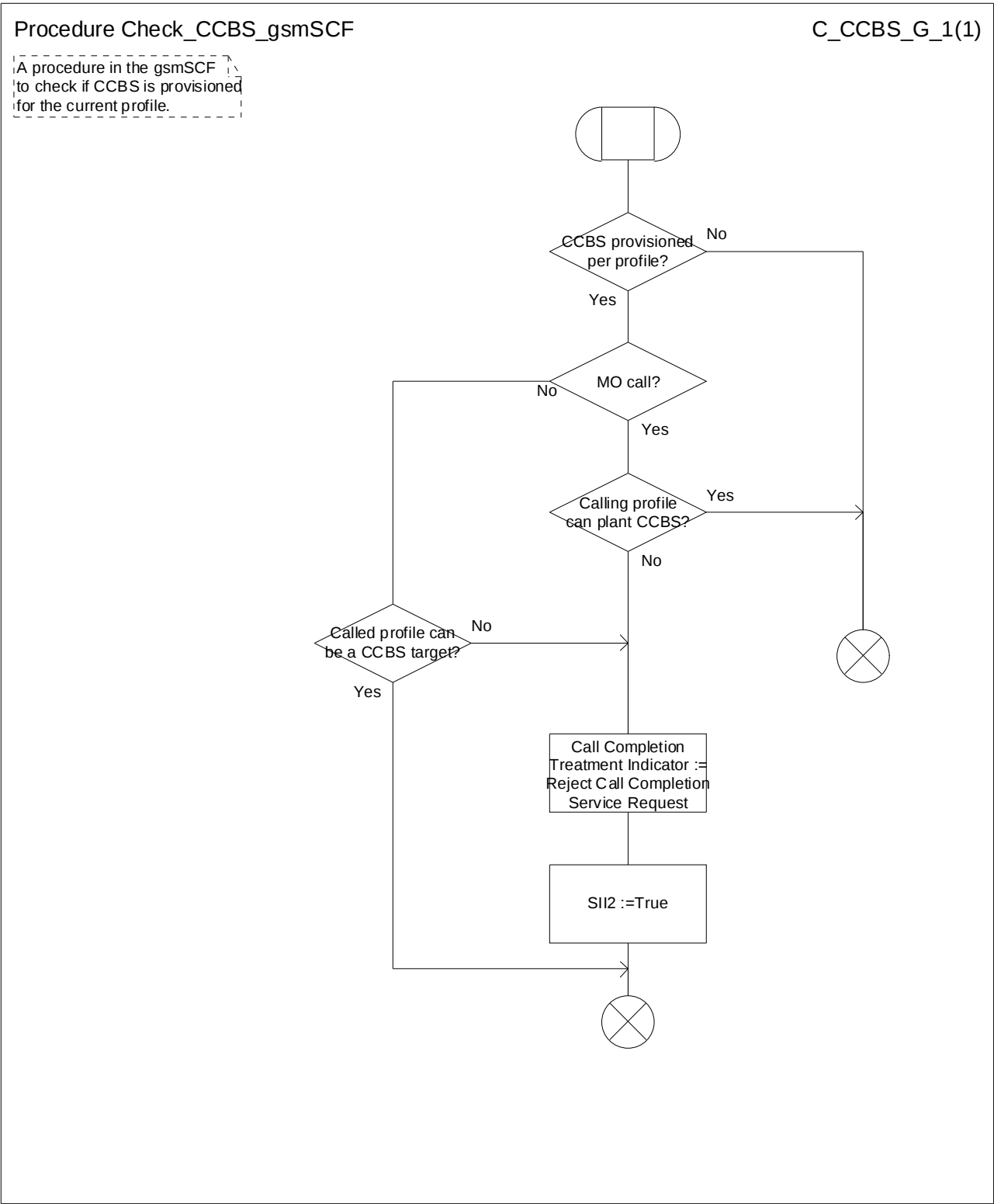
Figure 27: Procedure Check_CCBS_gsmSCF
