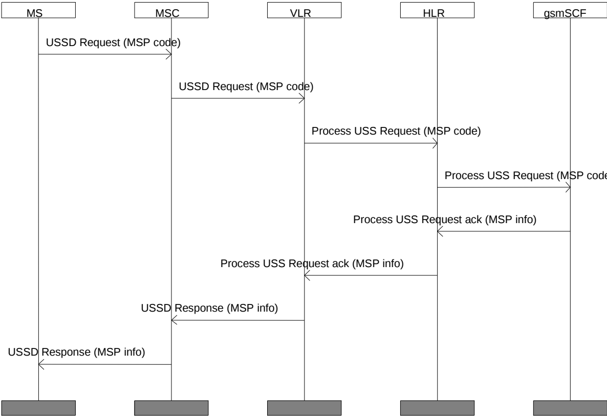
Figure 3: Interrogating MSP: information flow
