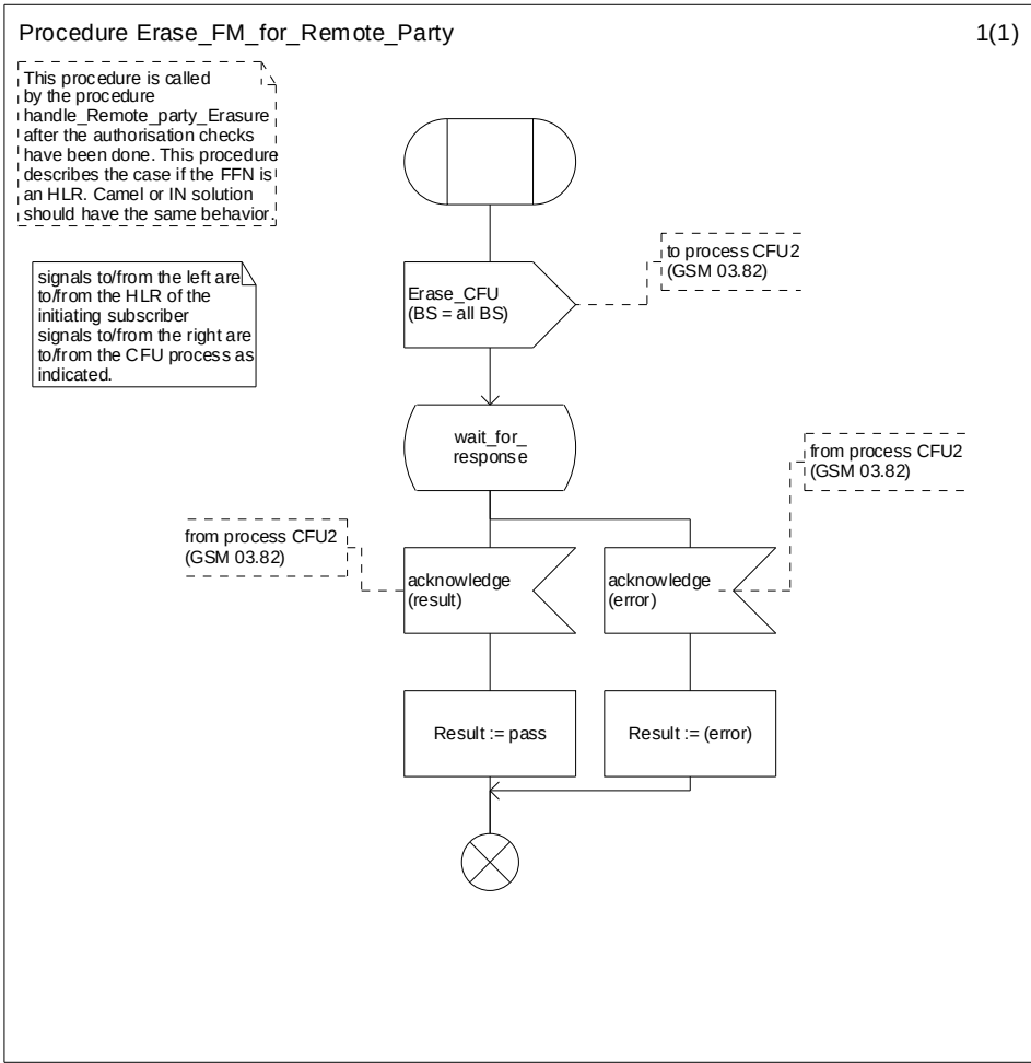
Figure 4.7a: Procedure Erase_FM_for_Remote_party
