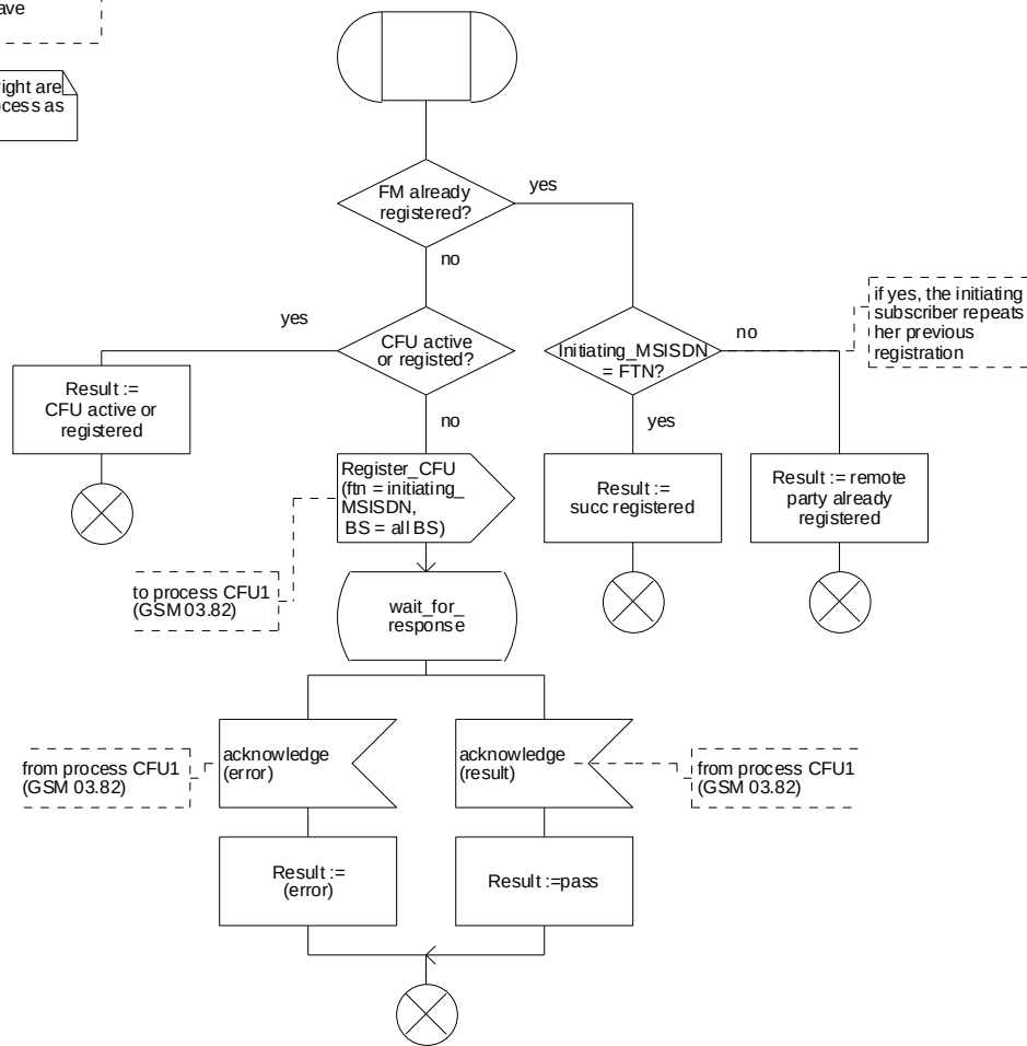
Figure 4.6a: Procedure Register_FM_for_Remote_Party
