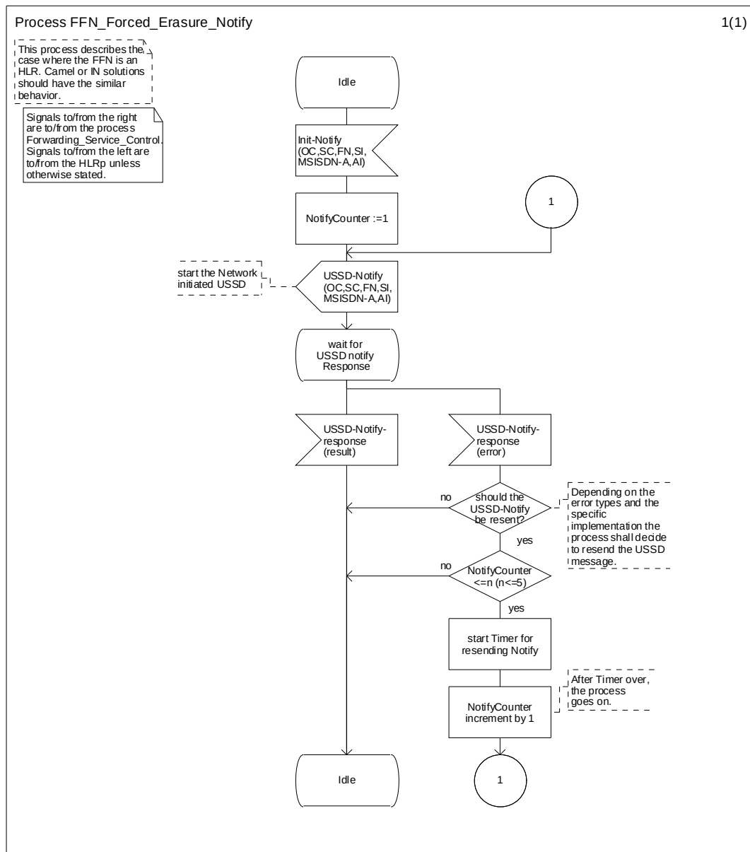
Figure 4.9: Process FFN_Forced_Erasure_Notify
