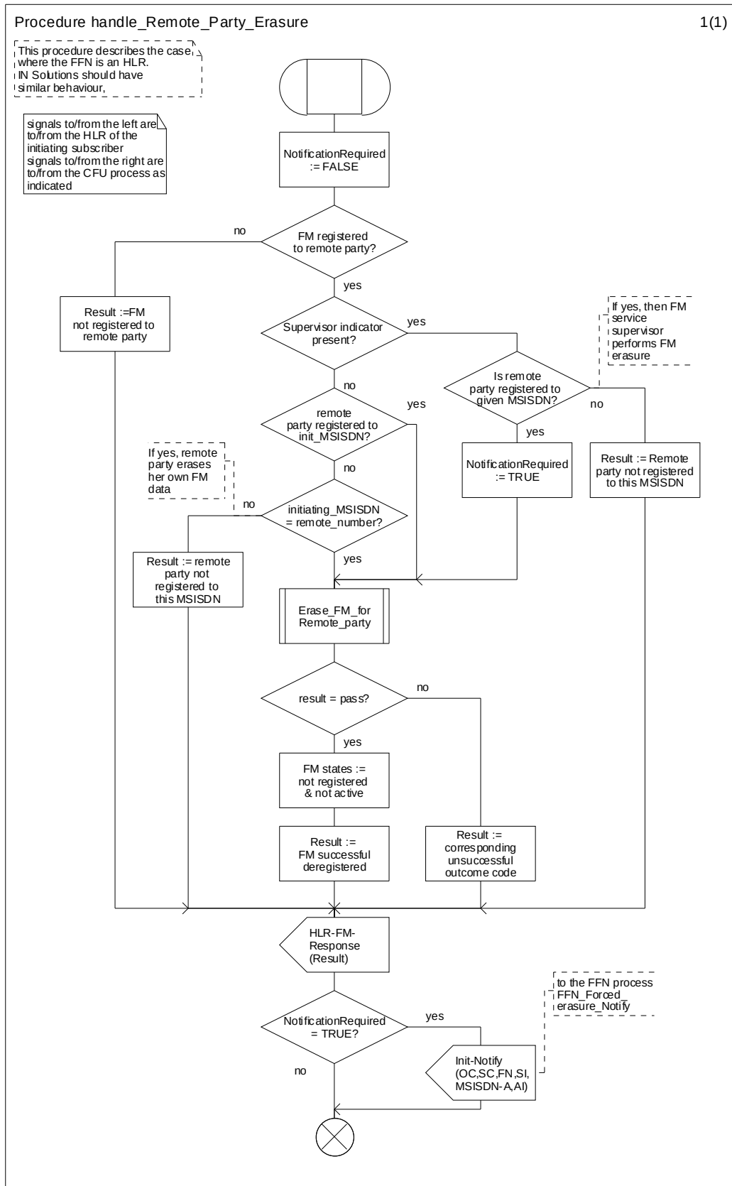
Figure 4.7: Procedure: Handle_Remote_Party_Erasure
