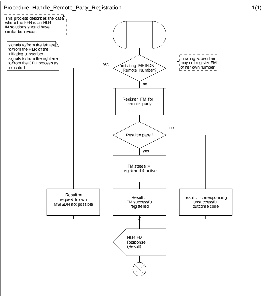
Figure 4.6: Procedure: Handle_Remote_Party_Registration
