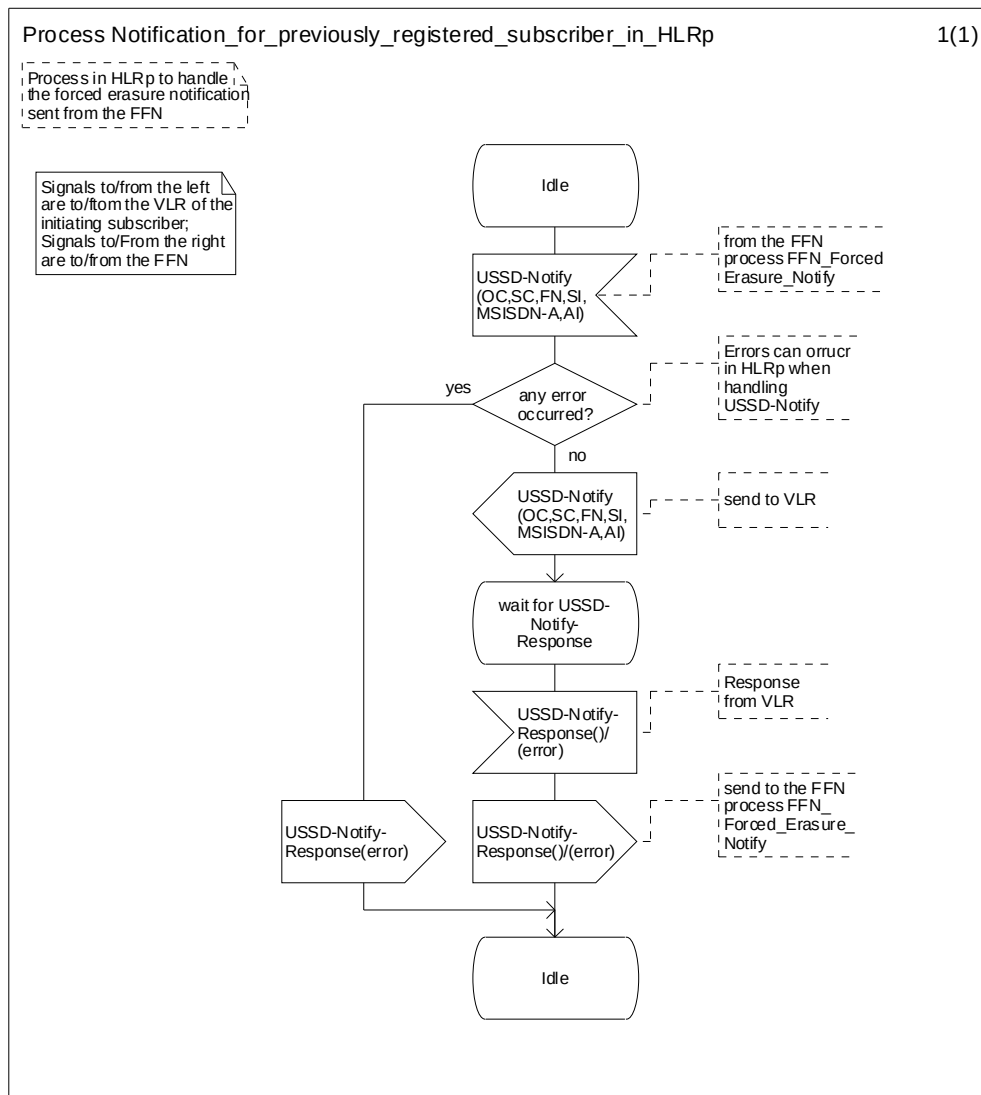
Figure 4.2a: Process Notification_for_previously_registered_subscriber_in_HLRp
