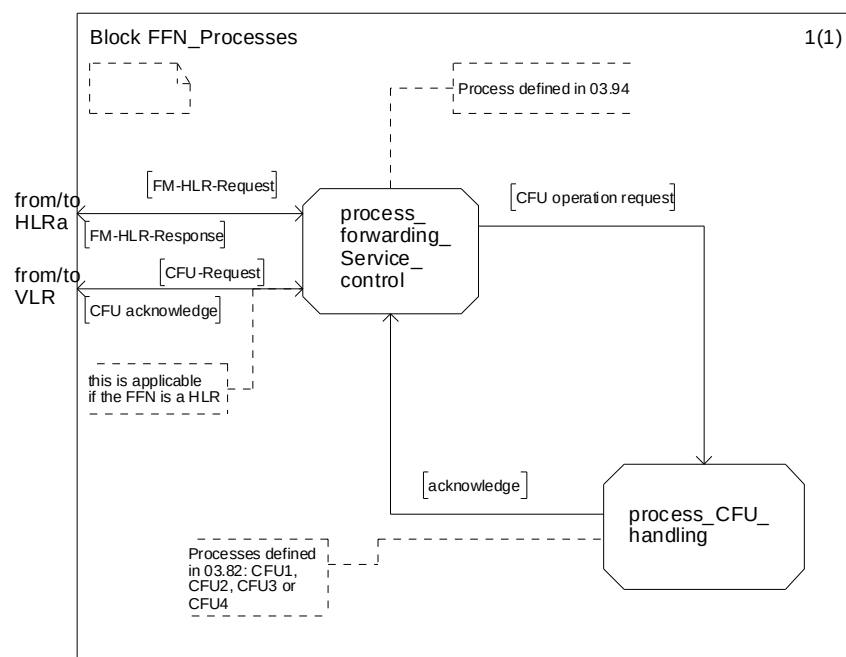
Figure 4.3: FFN_processes
