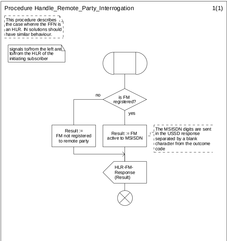
Figure 4.8: Procedure Handle_Remote_Party_Interrogation
