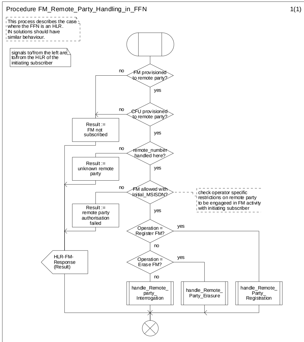
Figure 4.5: Procedure: FM_Remote_Party_Handling_in_FFN
