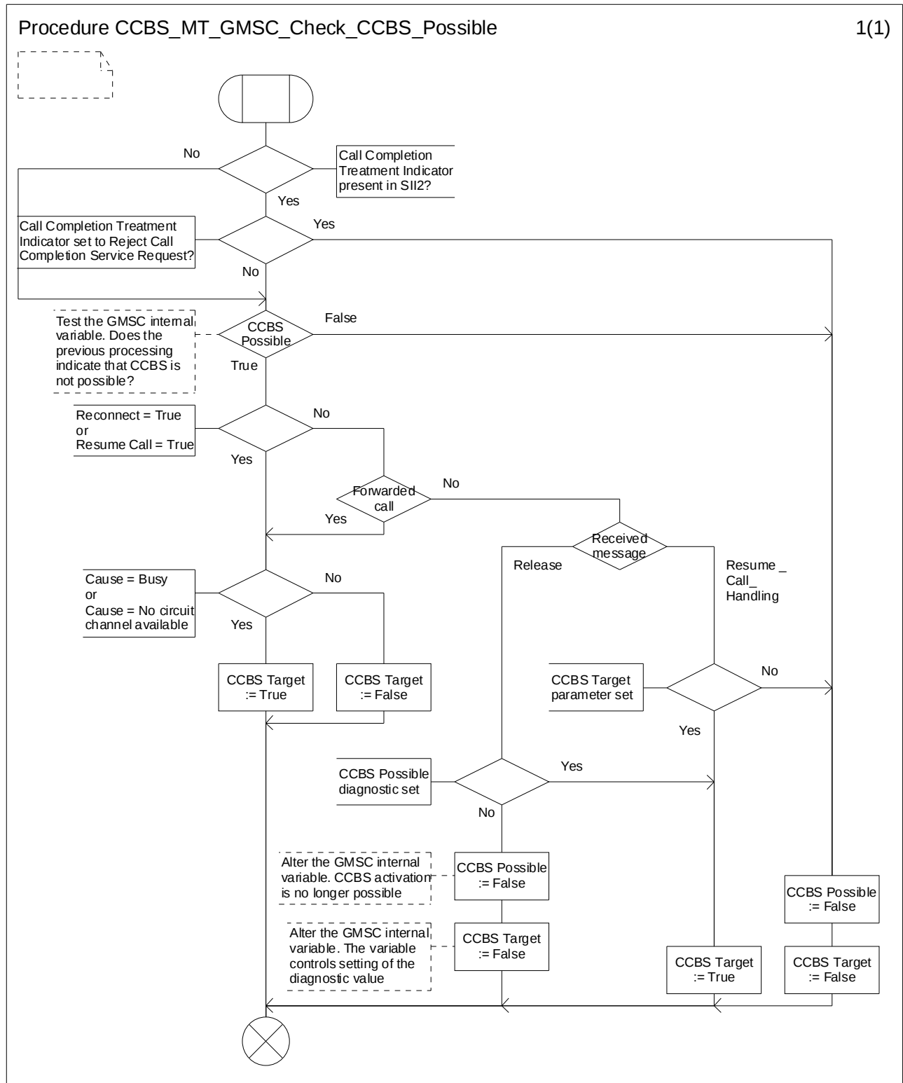
Figure 11.2.1.5: Procedure CCBS_MT_GMSC_Check_CCBS_Possible
