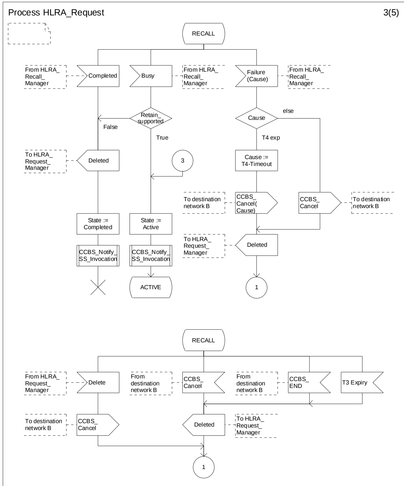
Figure 11.1.2.3: Process HLRA_Request (sheet 3 of 5)
