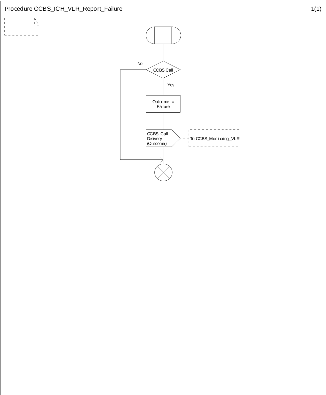
Figure 11.2.3.5: Procedure CCBS_ICH_VLR_Report_Failure
