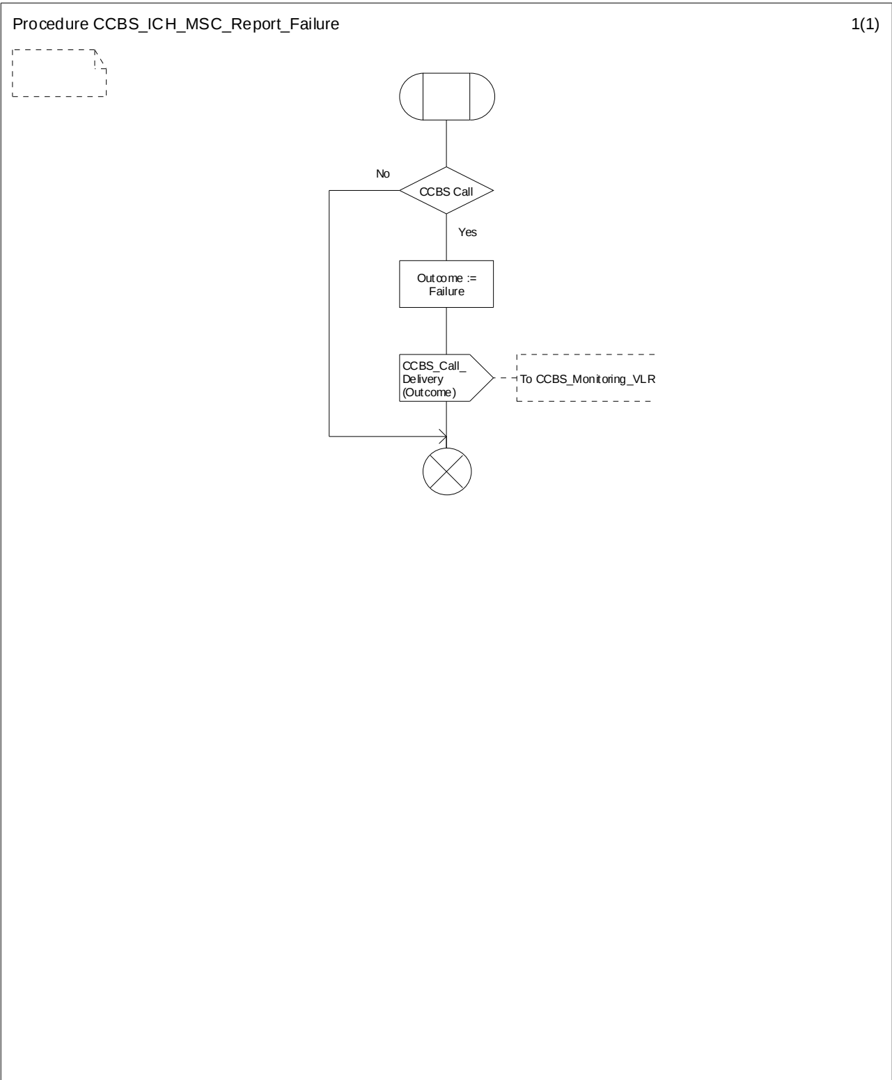
Figure 11.2.3.4: Procedure CCBS_ICH_MSC_Report_Failure
