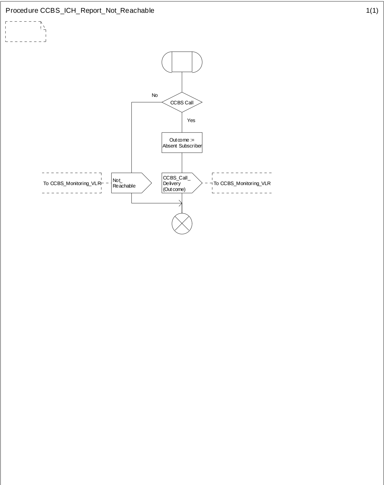
Figure 11.2.3.6: Procedure CCBS_ICH_Report_Not_Reachable
