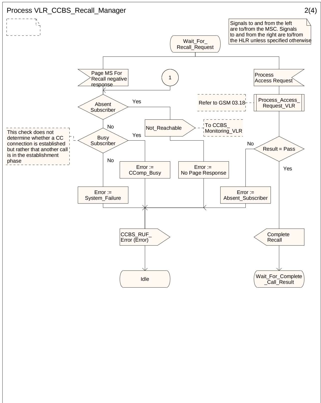
Figure 11.1.1.2: Process VLR_CCBS_Recall_Manager (sheet 2 of 4)
