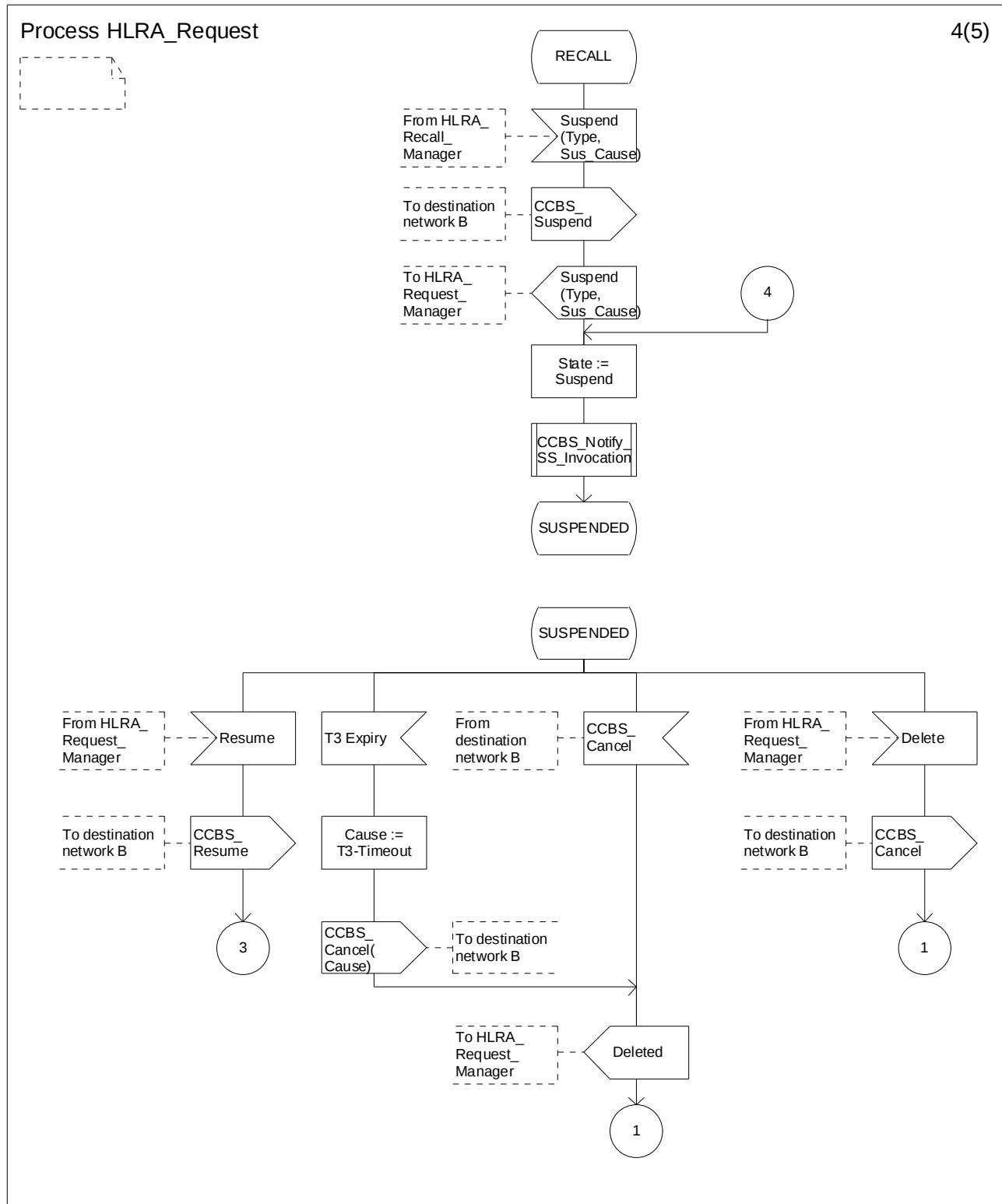
Figure 11.1.2.3: Process HLRA_Request (sheet 4 of 5)
