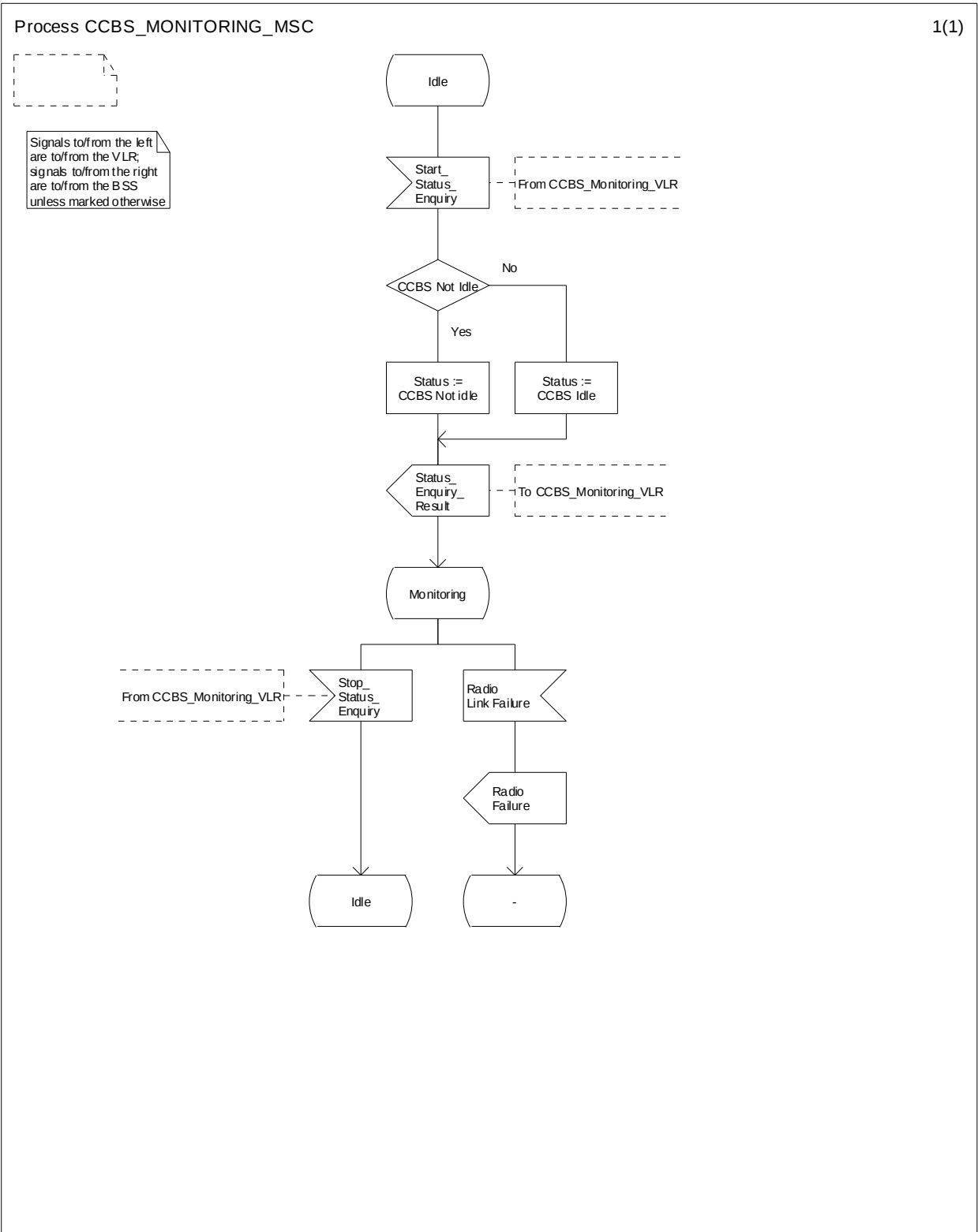
Figure 11.3.2: Process CCBS_Monitoring_MSC
