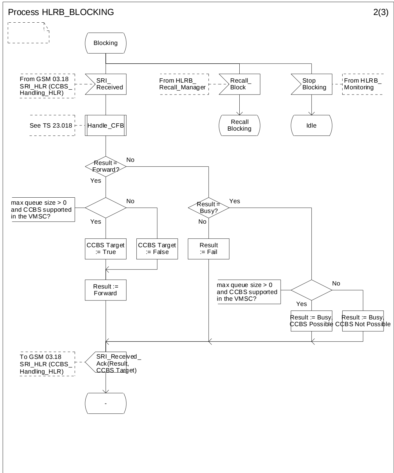
Figure 11.2.2.6: Process HLRB_BLOCKING (sheet 2 of 3)
