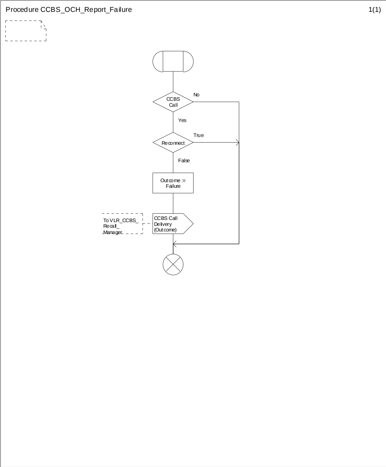
Figure 11.1.1.12: Procedure CCBS_OCH_Report_Failure
