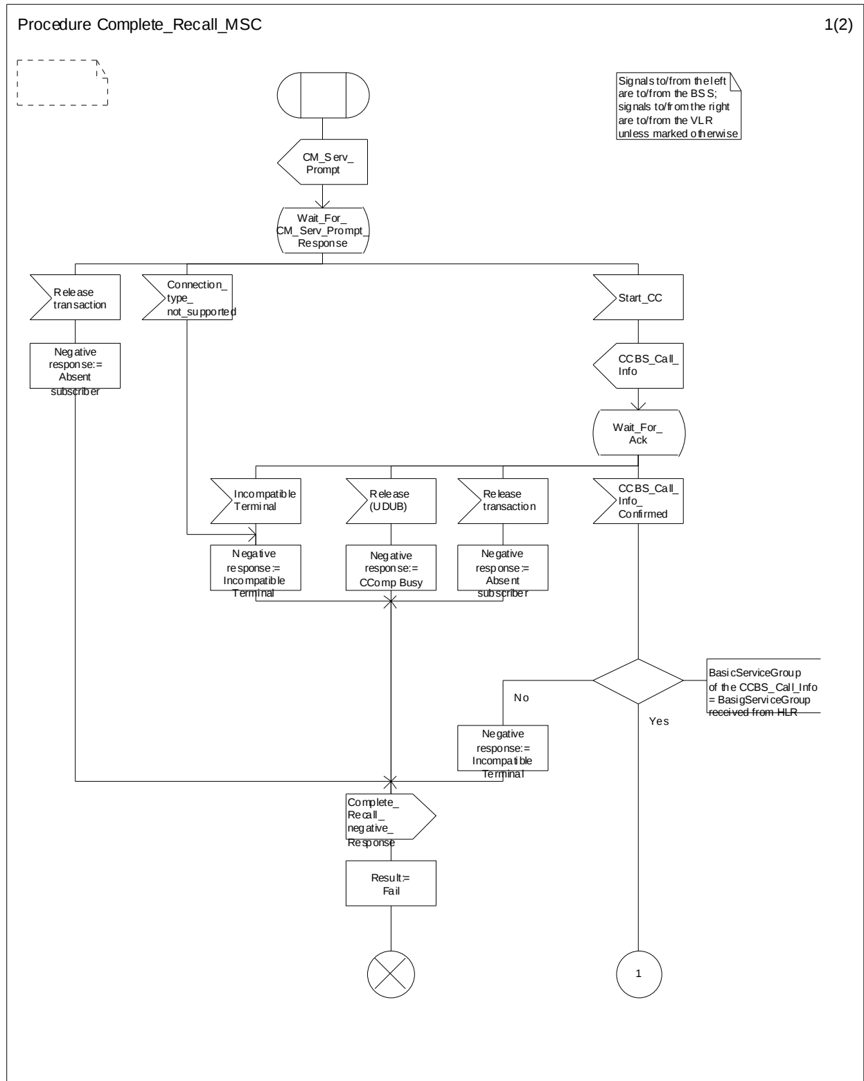
Figure 11.1.1.10: Procedure Complete_Recall_MSC (sheet 1 of 2)
