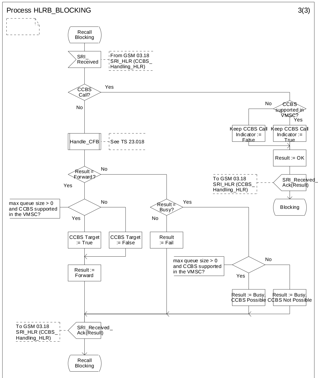
Figure 11.2.2.6: Process HLRB_BLOCKING (sheet 3 of 3)
