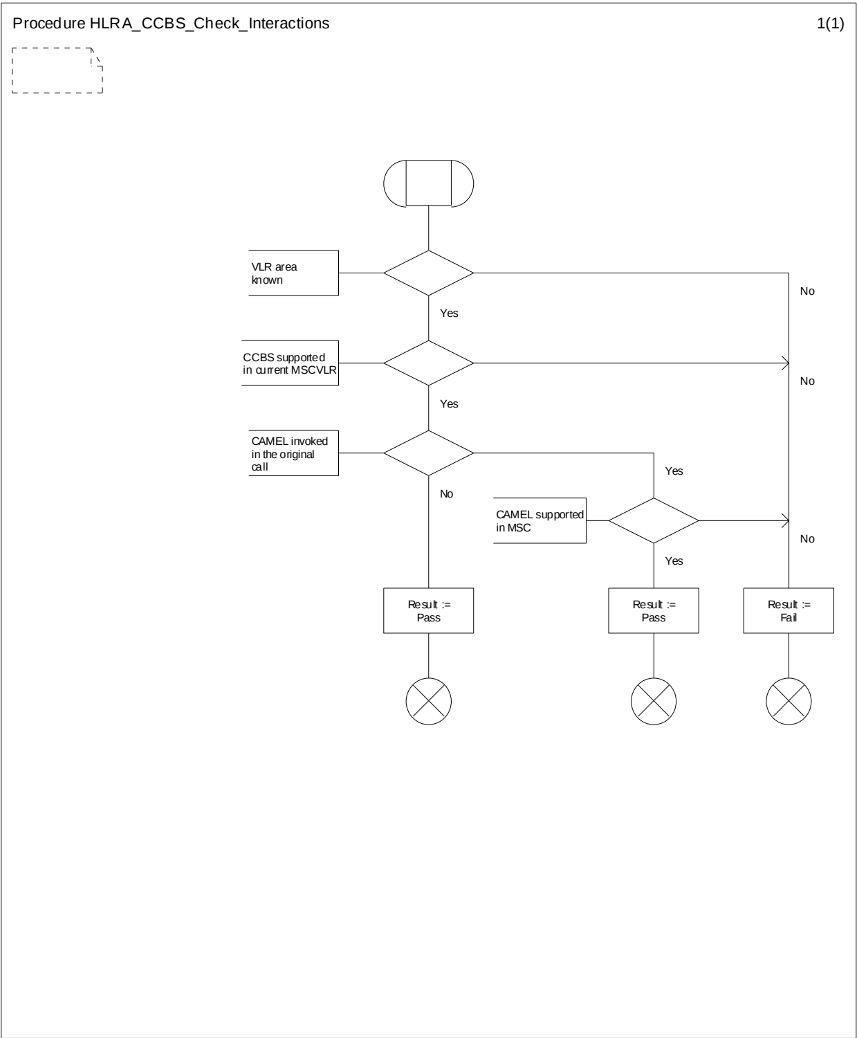
Figure 11.1.2.7: Procedure HLRA_CCBS_Check_Interactions
