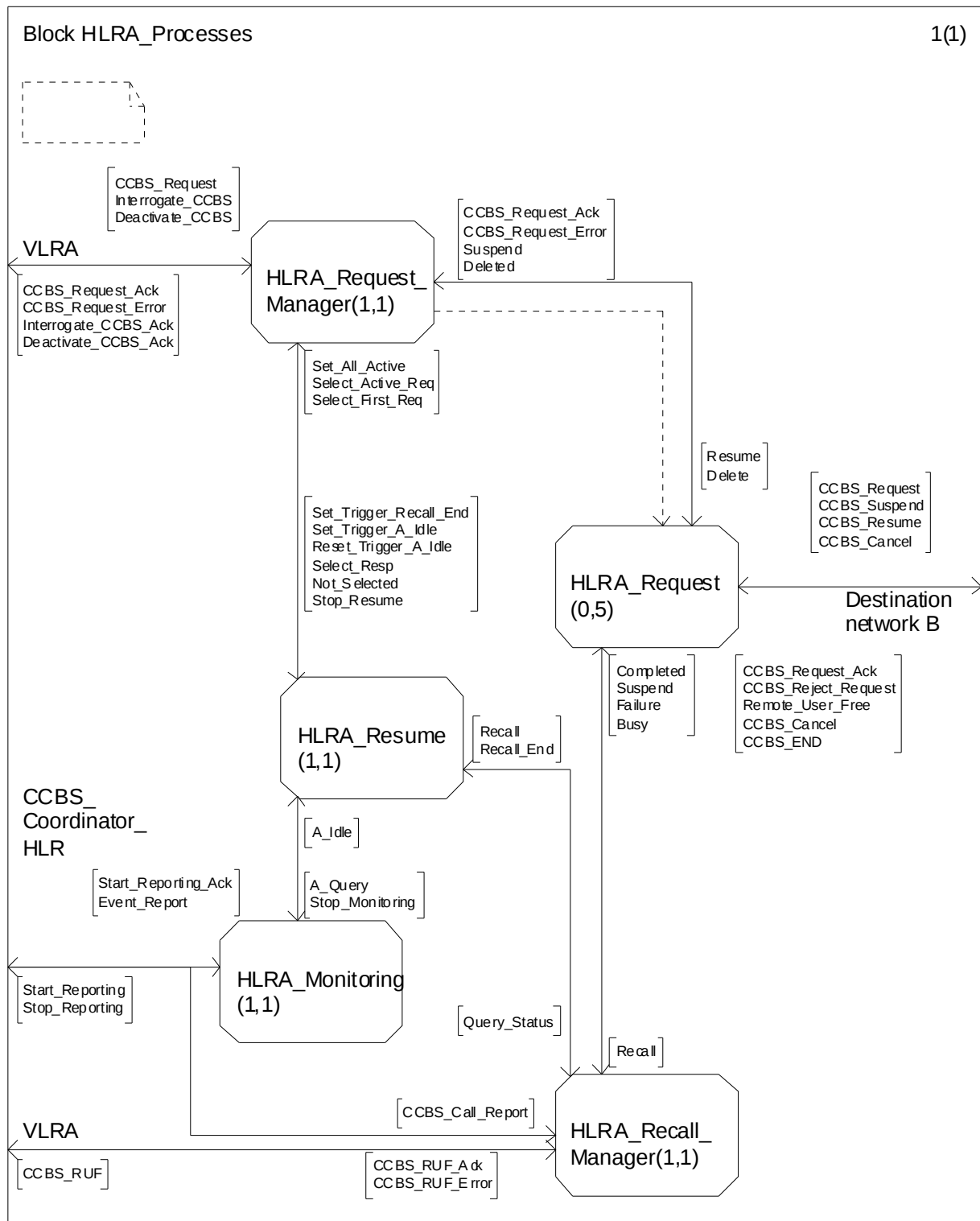
Figure 11.1.2.1: HLRA Processes
