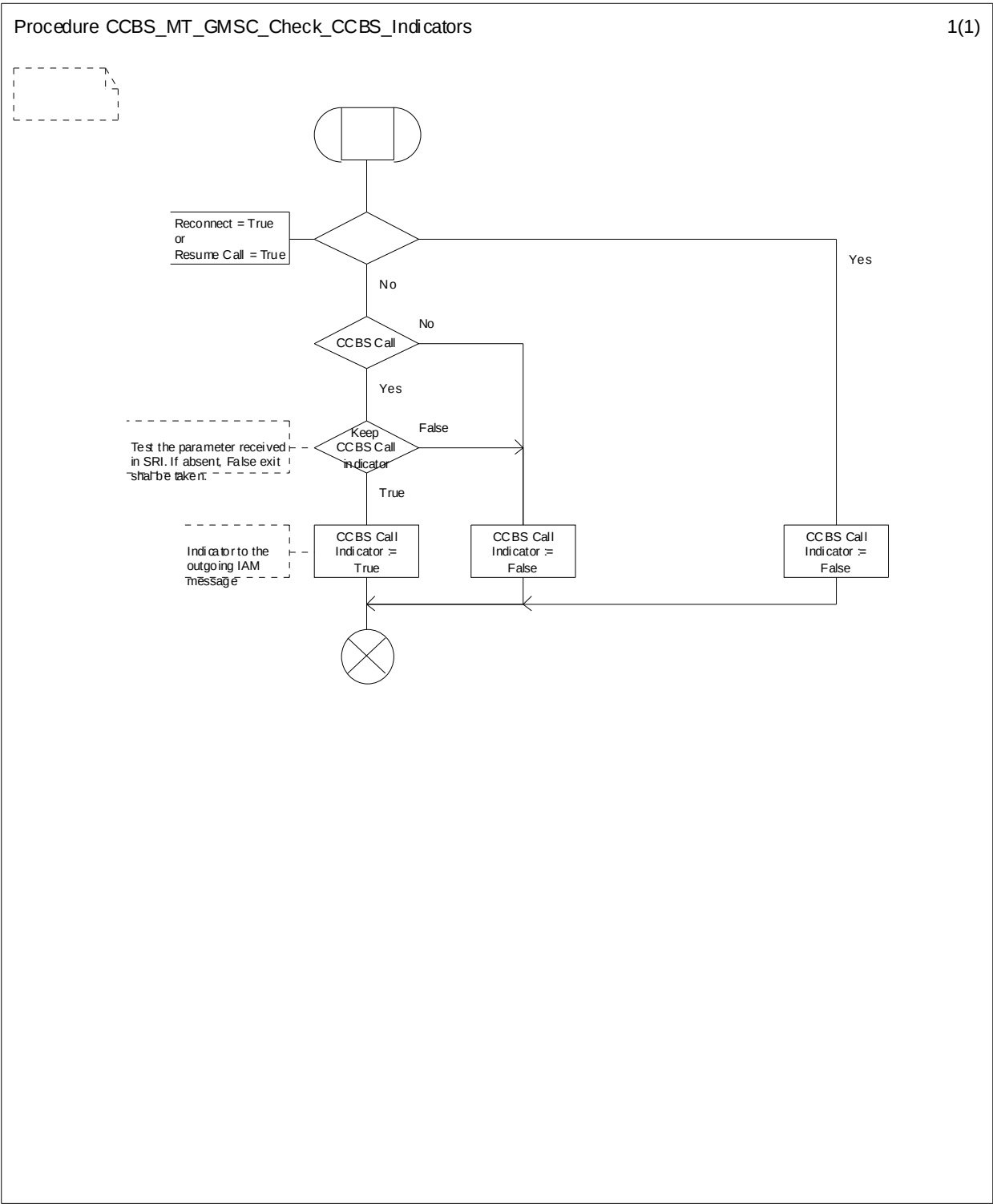
Figure 11.2.1.2: Procedure CCBS_MT_GMSC_Check_CCBS_Indicators
