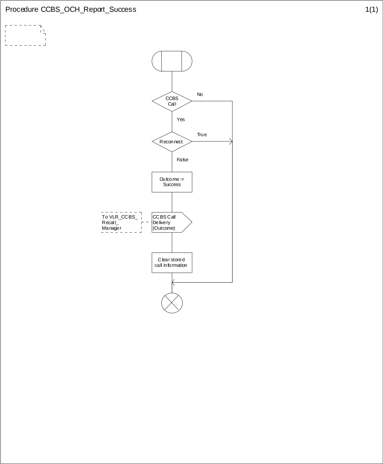
Figure 11.1.1.11: Procedure CCBS_OCH_Report_Success
