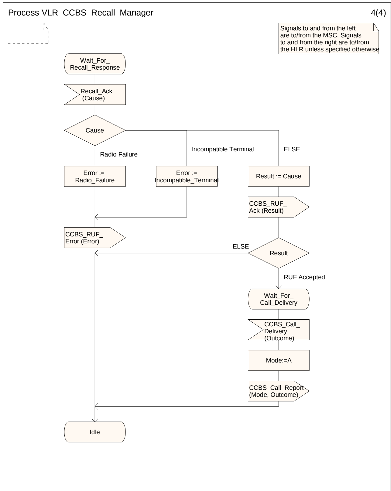
Figure 11.1.1.2: Process VLR_CCBS_Recall_Manager (sheet 4 of 4)
