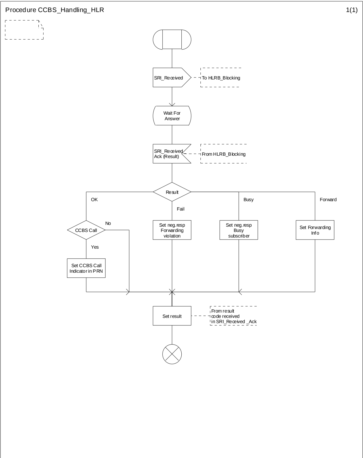
Figure 11.2.2.8: Procedure CCBS_Handling_HLR
