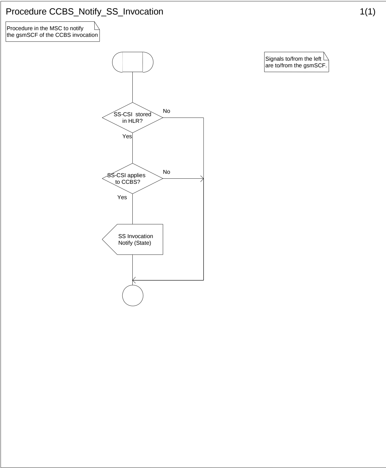
Figure 11.1.2.8: Procedure CCBS_Notify_SS_Invocation
