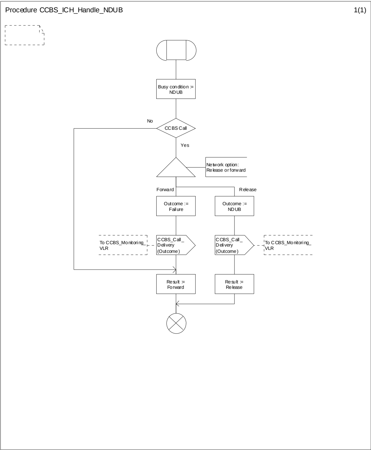
Figure 11.2.3.7: Procedure CCBS_ICH_Handle_NDUB
