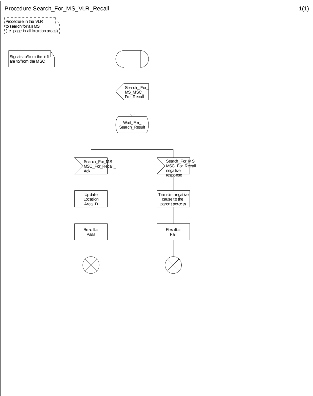
Figure 11.1.1.9: Procedure Search_For_MS_VLR_Recall
