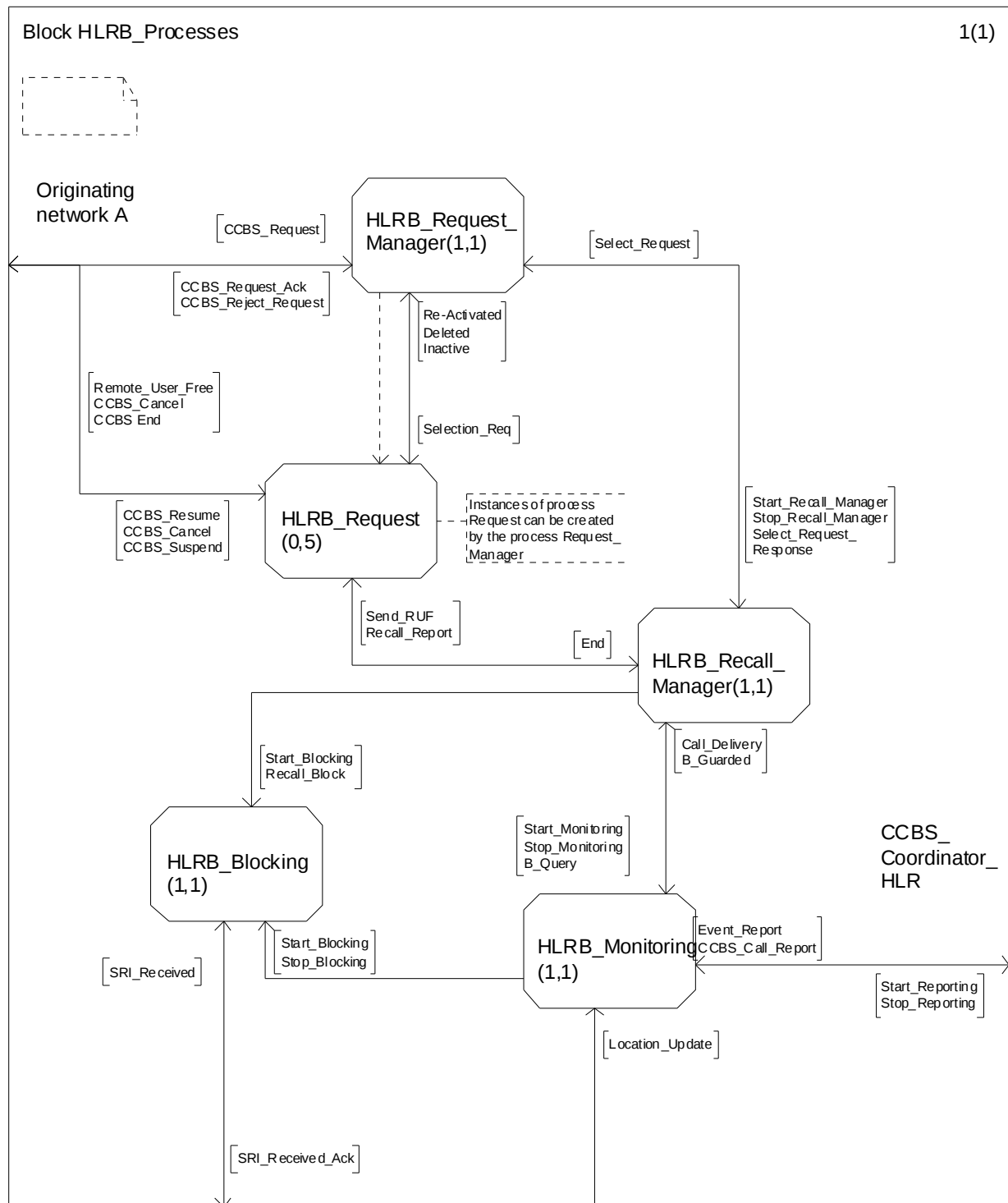
Figure 11.2.2.1: HLRB_Processes
