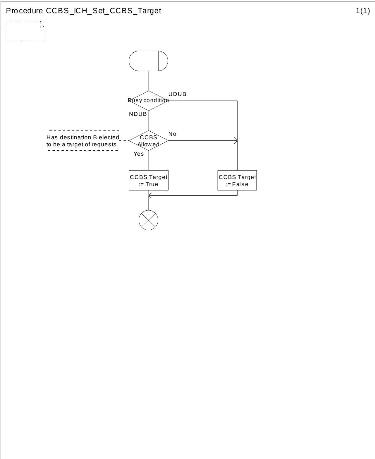
Figure 11.2.3.11: Procedure CCBS_ICH_Set_CCBS_Target
