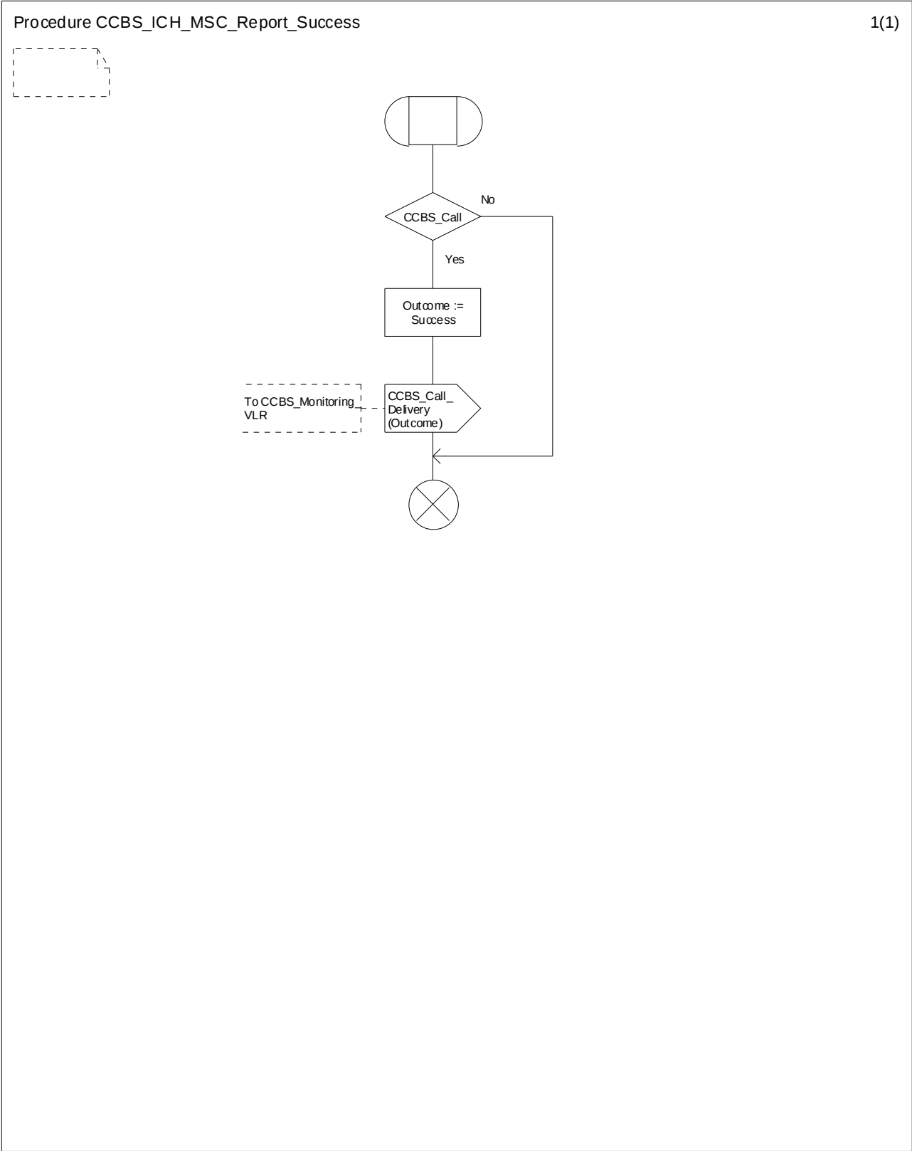
Figure 11.2.3.9: Procedure CCBS_ICH_MSC_Report_Success
