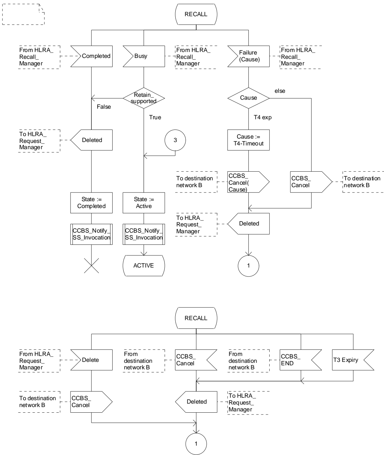
Figure 11.1.2.3: Process HLRA_Request (sheet 3 of 5)
