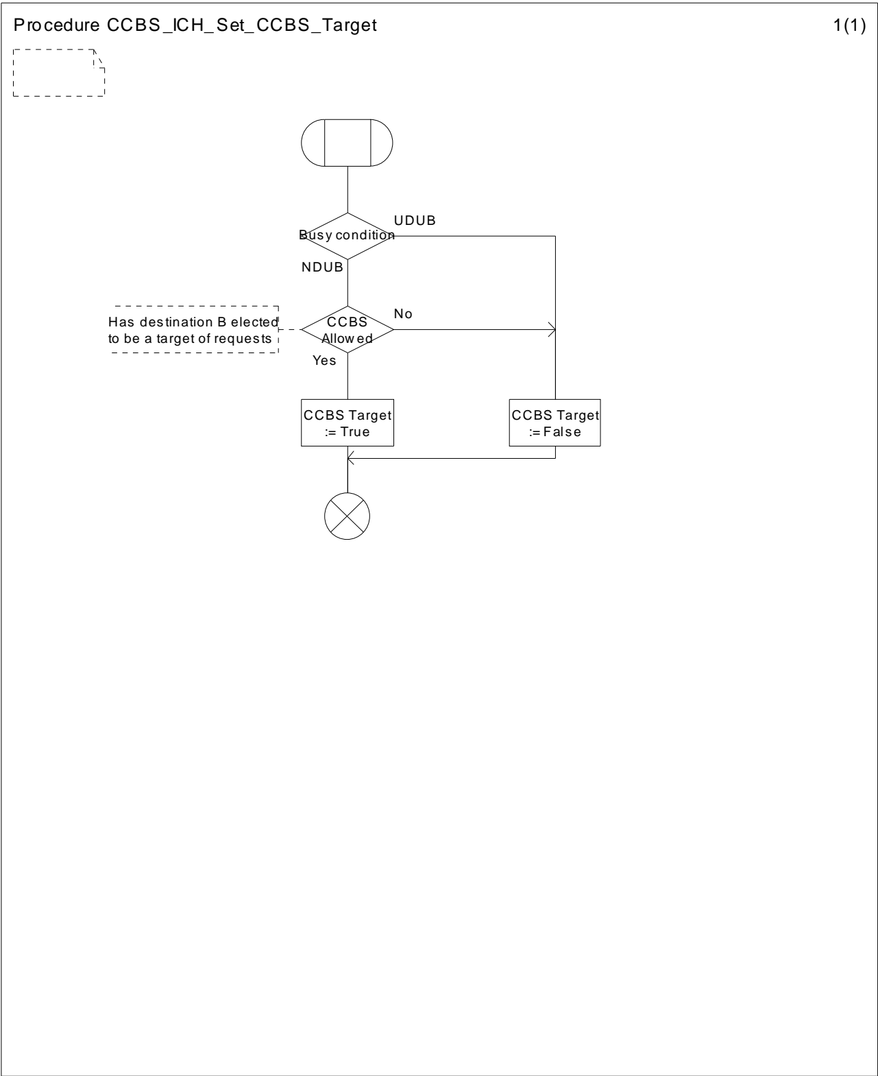
Figure 11.2.3.11: Procedure CCBS_ICH_Set_CCBS_Target
