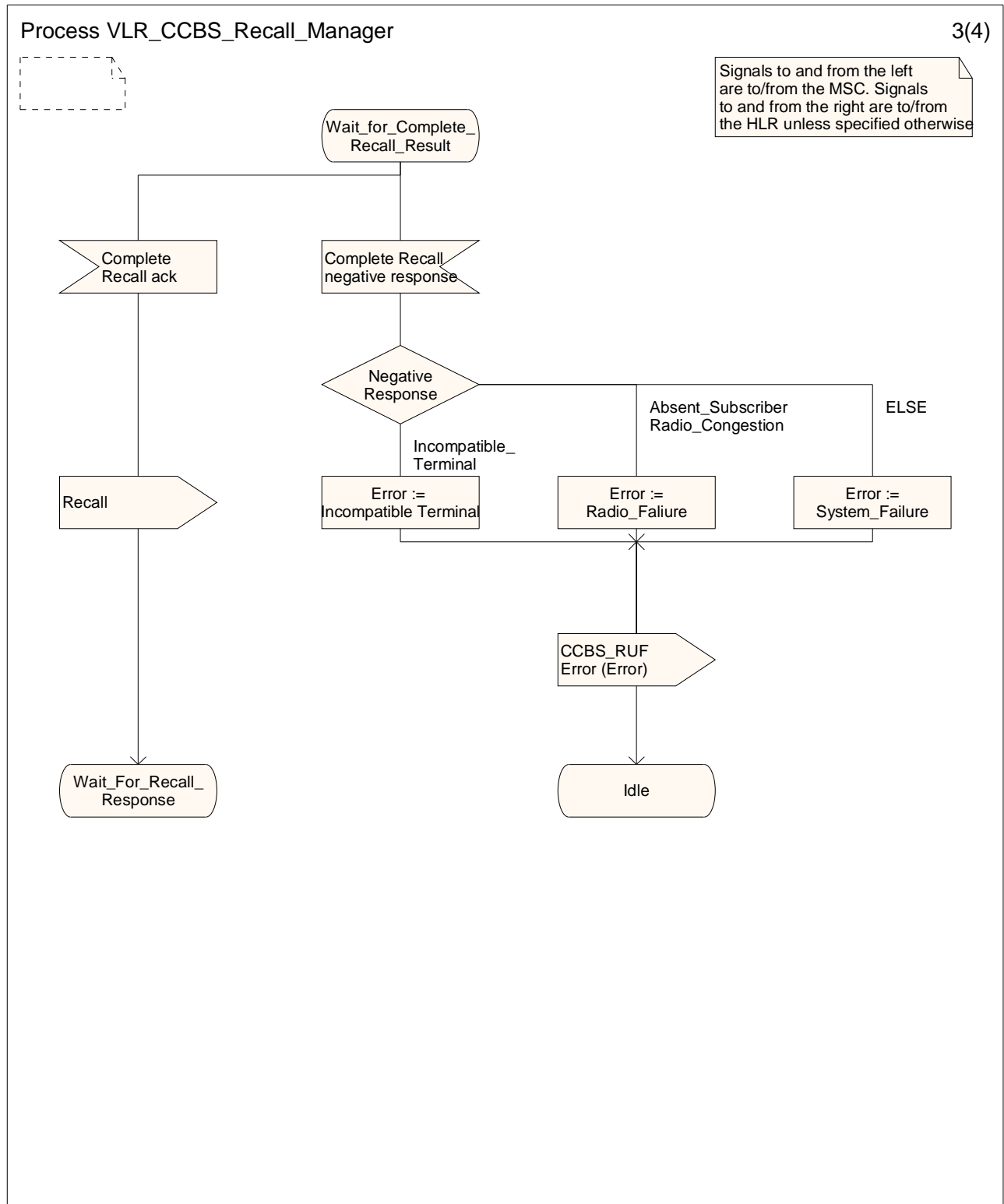
Figure 11.1.1.2: Process VLR_CCBS_Recall_Manager (sheet 3 of 4)
