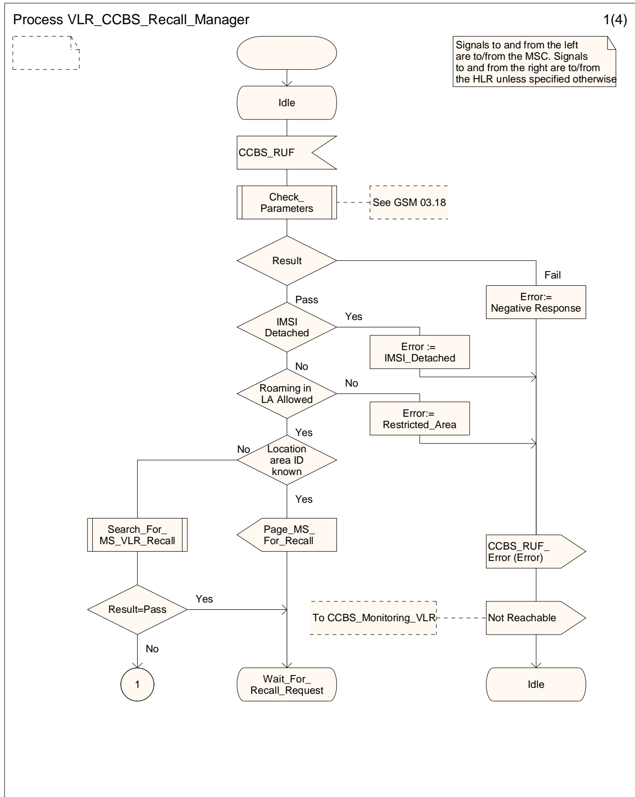
Figure 11.1.1.2: Process VLR_CCBS_Recall_Manager (sheet 1 of 4)
